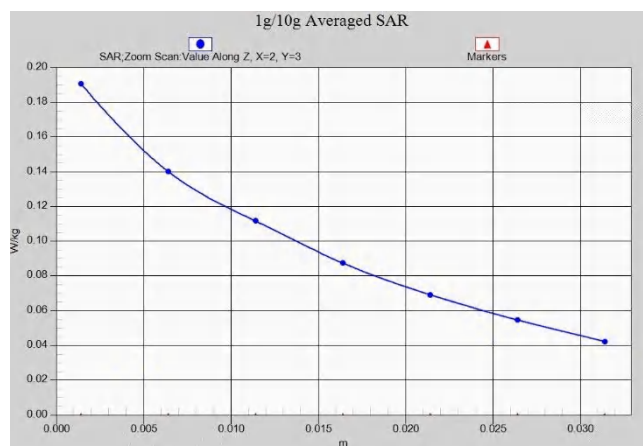
Z-Scan at power reference point (GSM850 ANT1 Body 15mm)
