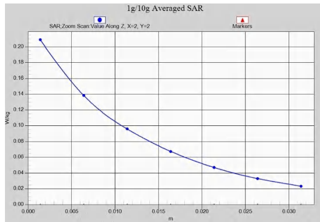
Z-Scan at power reference point (WCDMA1700 ANT0 Head)
