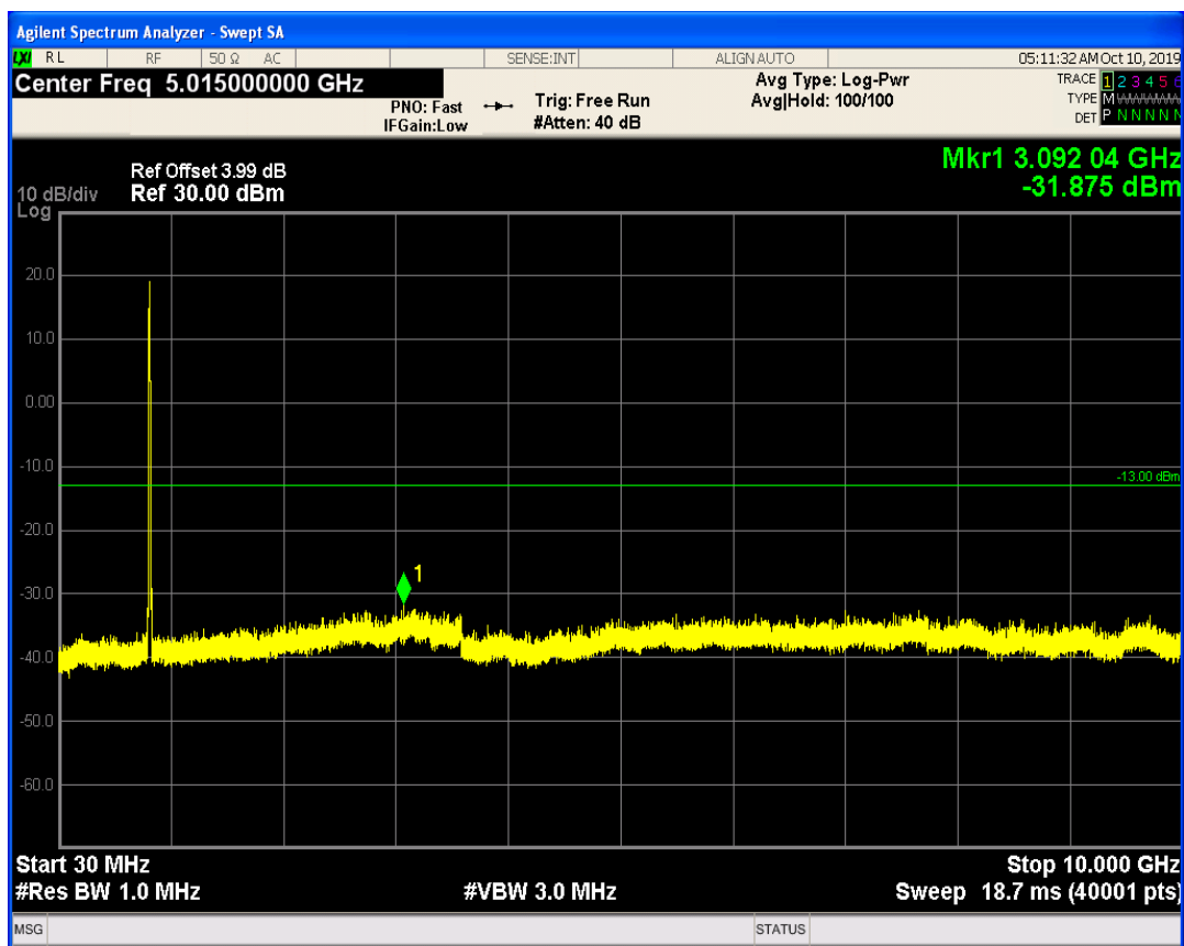
LTE Band19 QPSK BW=10MHz Channel=24100 RB Size=50 Position=#0
