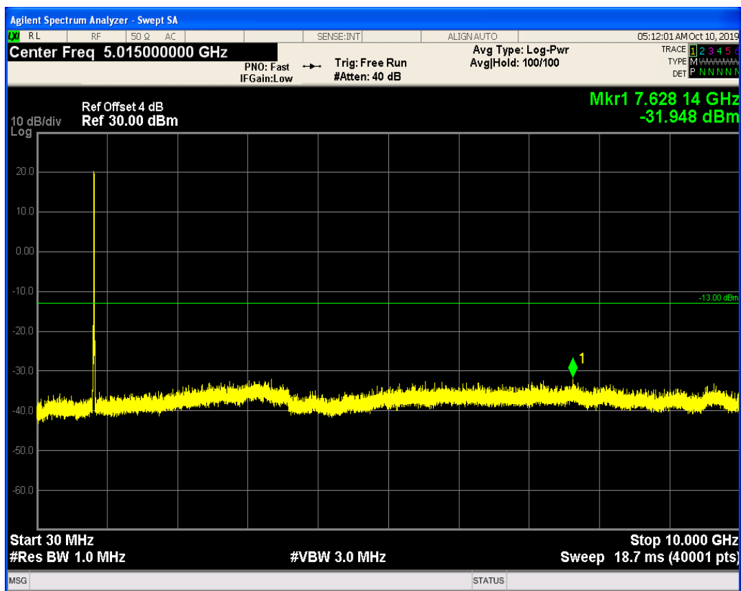
LTE Band19 QAM16 BW=10MHz Channel=24100 RB Size=50 Position=#0
