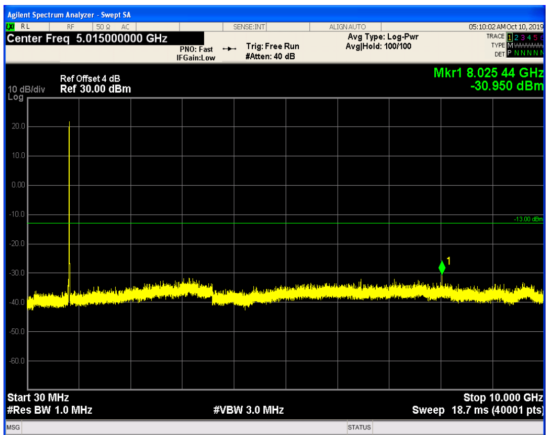
LTE Band19 QAM16 BW=5MHz Channel=24125 RB Size=25 Position=#0
