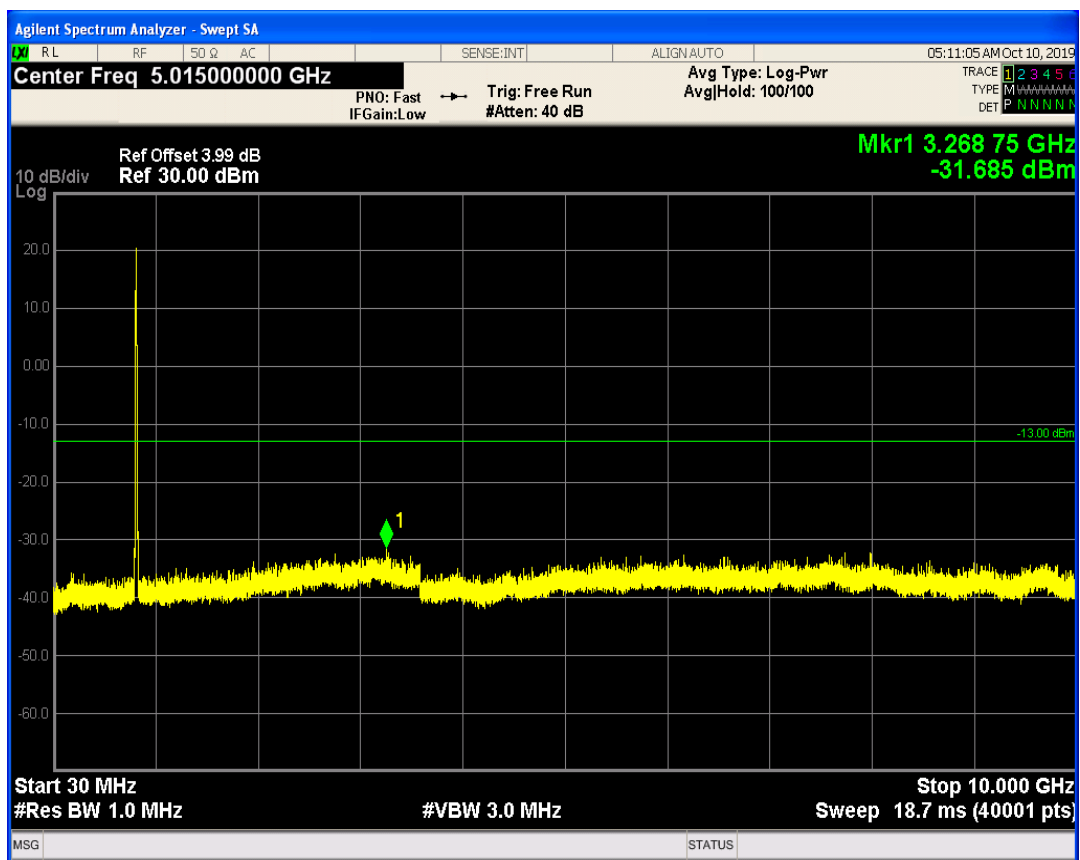
LTE Band19 QAM16 BW=10MHz Channel=24050 RB Size=50 Position=#0
