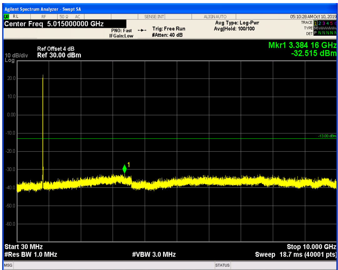
LTE Band19 QPSK BW=10MHz Channel=24050 RB Size=50 Position=#0
