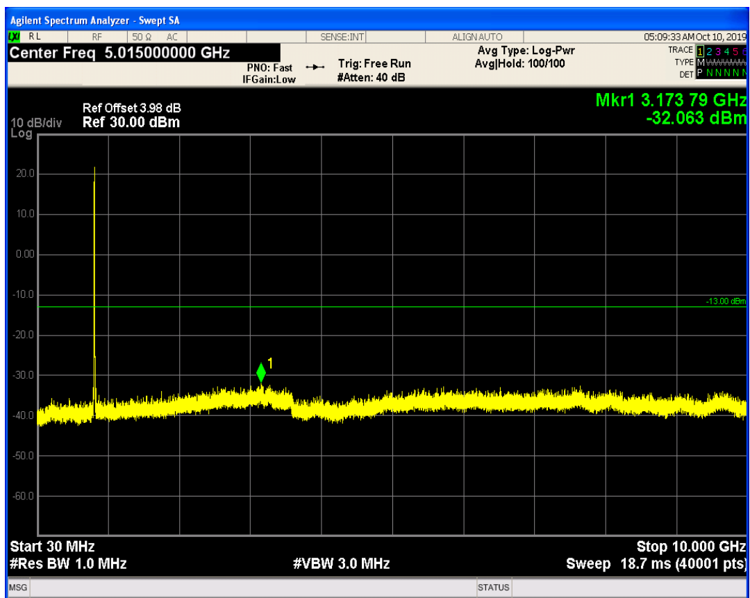
LTE Band19 QPSK BW=5MHz Channel=24125 RB Size=25 Position=#0
