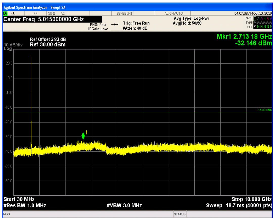
LTE Band19 QPSK BW=5MHz Channel=24025 RB Size=25 Position=#0
