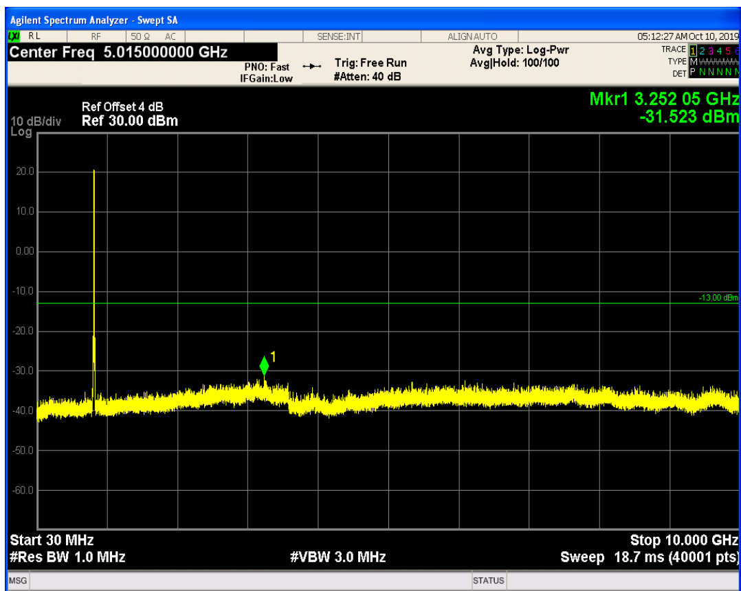
LTE Band19 QAM16 BW=15MHz Channel=24075 RB Size=75 Position=#0
