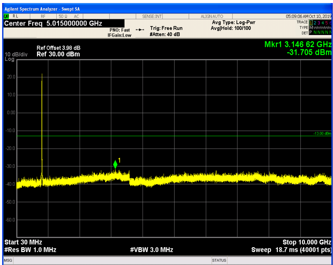
LTE Band19 QAM16 BW=5MHz Channel=24025 RB Size=25 Position=#0
