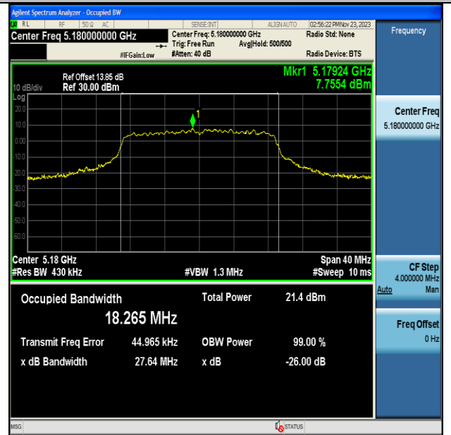
11AC20MIMO-Ant7-5180
