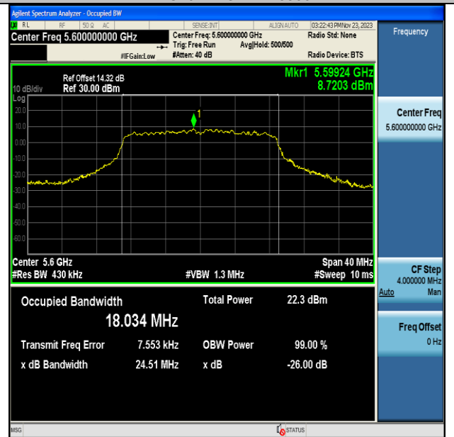
11AC20MIMO-Ant7-5600
