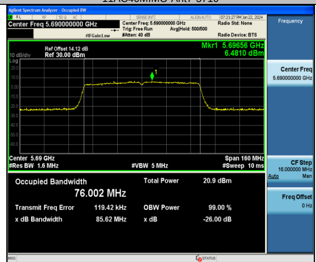
11AC80MIMO-Ant7-5690
