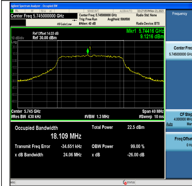
11AC20MIMO-Ant6-5745
