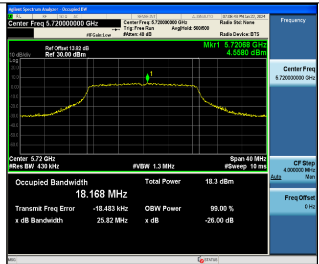
11AC20MIMO-Ant7-5720
