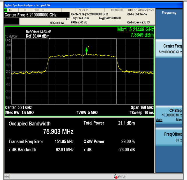
11AC80MIMO-Ant7-5210
