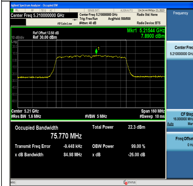
11AC80MIMO-Ant6-5210
