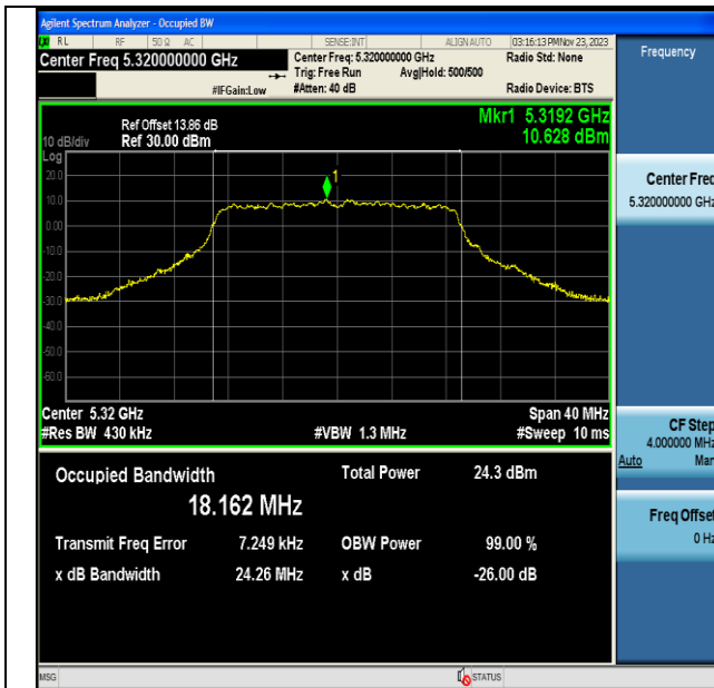
11AC20MIMO-Ant6-5320
