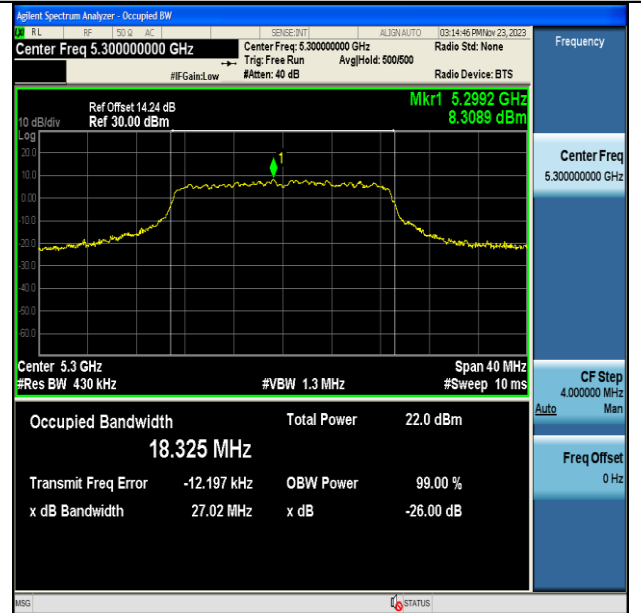
11AC20MIMO-Ant7-5300
