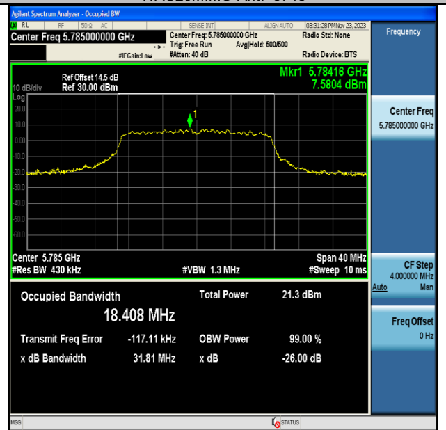
11AC20MIMO-Ant7-5785
