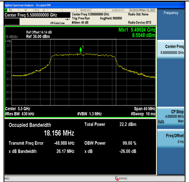
11AC20MIMO-Ant7-5500
