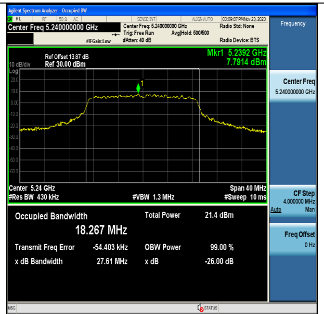
11AC20MIMO-Ant7-5240
