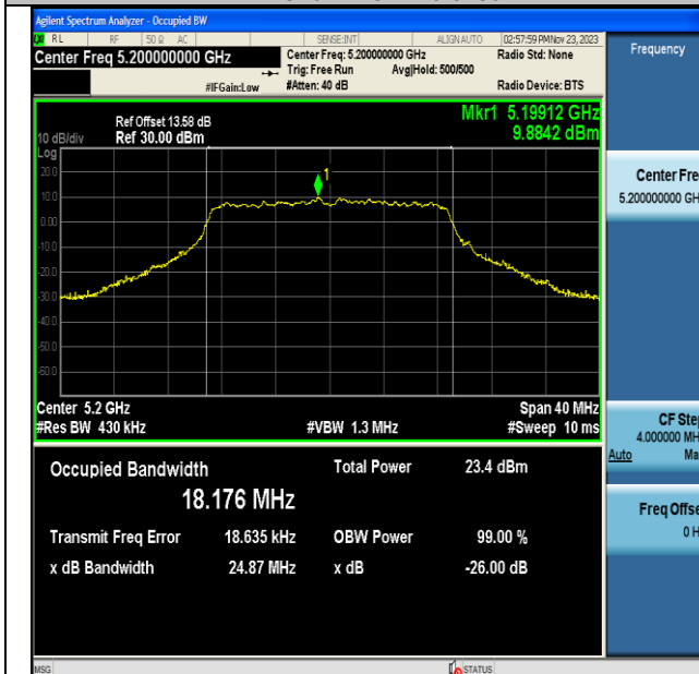
11AC20MIMO-Ant6-5200
