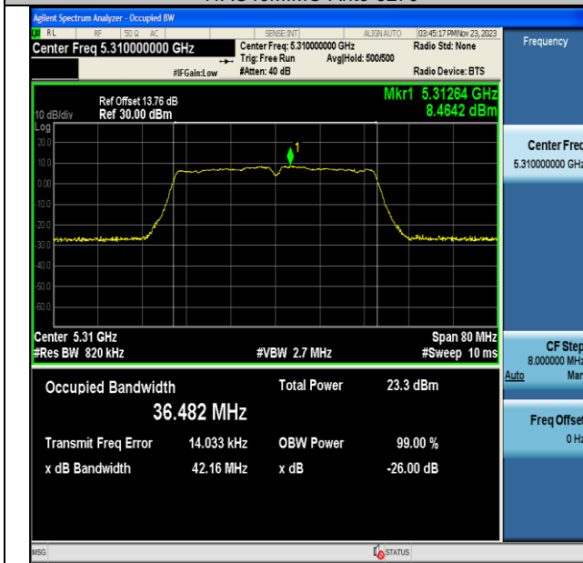
11AC40MIMO-Ant6-5310
