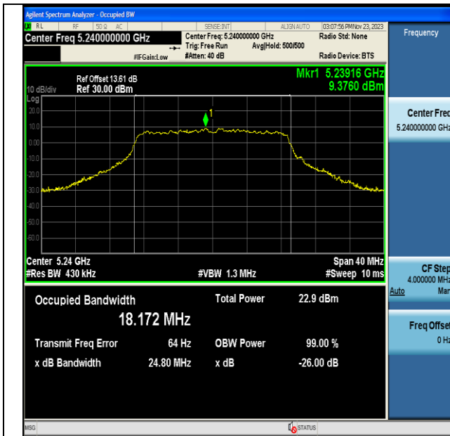
11AC20MIMO-Ant6-5240
