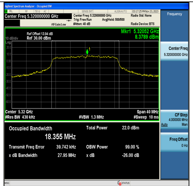
11AC20MIMO-Ant7-5320
