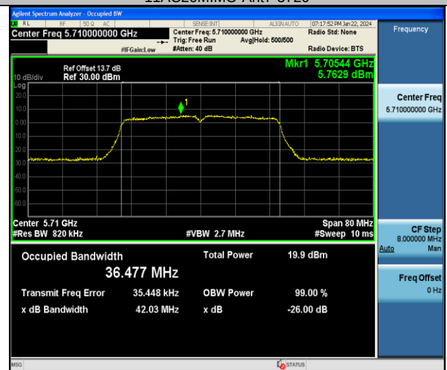
11AC40MIMO-Ant7-5710
