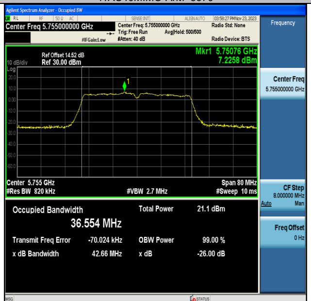
11AC40MIMO-Ant7-5755
