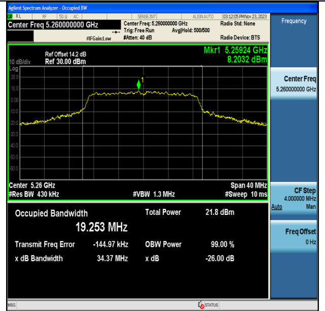
11AC20MIMO-Ant7-5260
