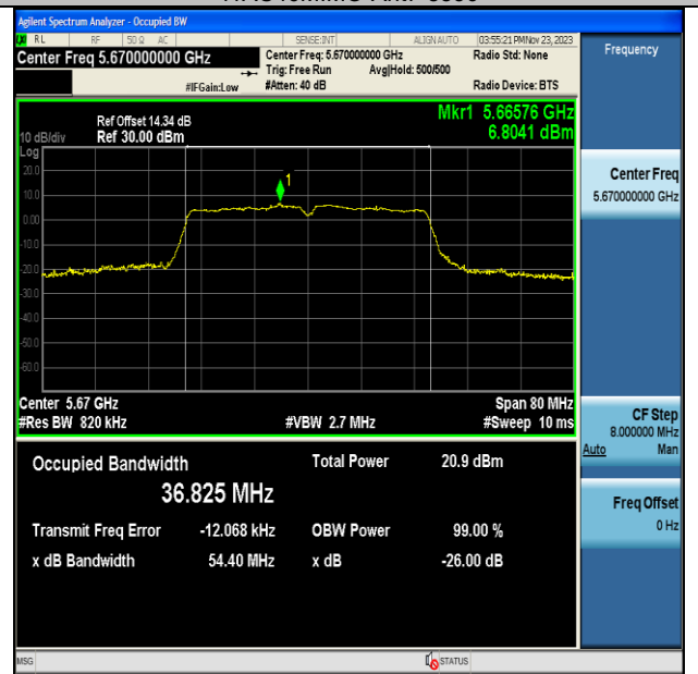
11AC40MIMO-Ant7-5670
