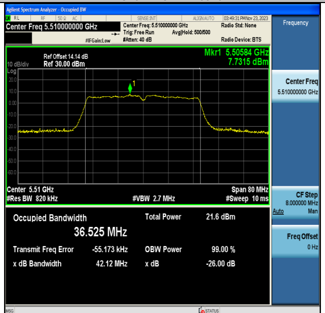
11AC40MIMO-Ant7-5510
