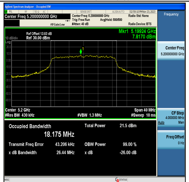
11AC20MIMO-Ant7-5200
