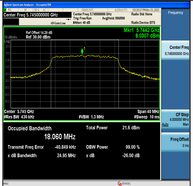
11AC20MIMO-Ant7-5745
