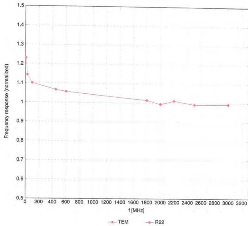
Frequency Response of E-Field (TEM-Cell:ifi110 EXX, Waveguide:R22)
