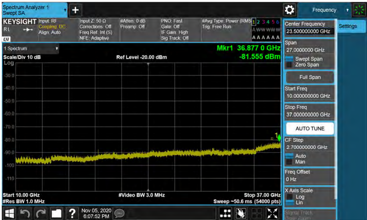
BAND 48. Conducted Spurious Plot 2 (20 MHz Ch. 56640 QPSK RB 1, Offset 0)
