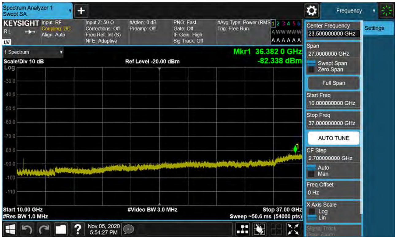
BAND 48. Conducted Spurious Plot 2 (20 MHz Ch. 55340 QPSK RB 1, Offset 0)
