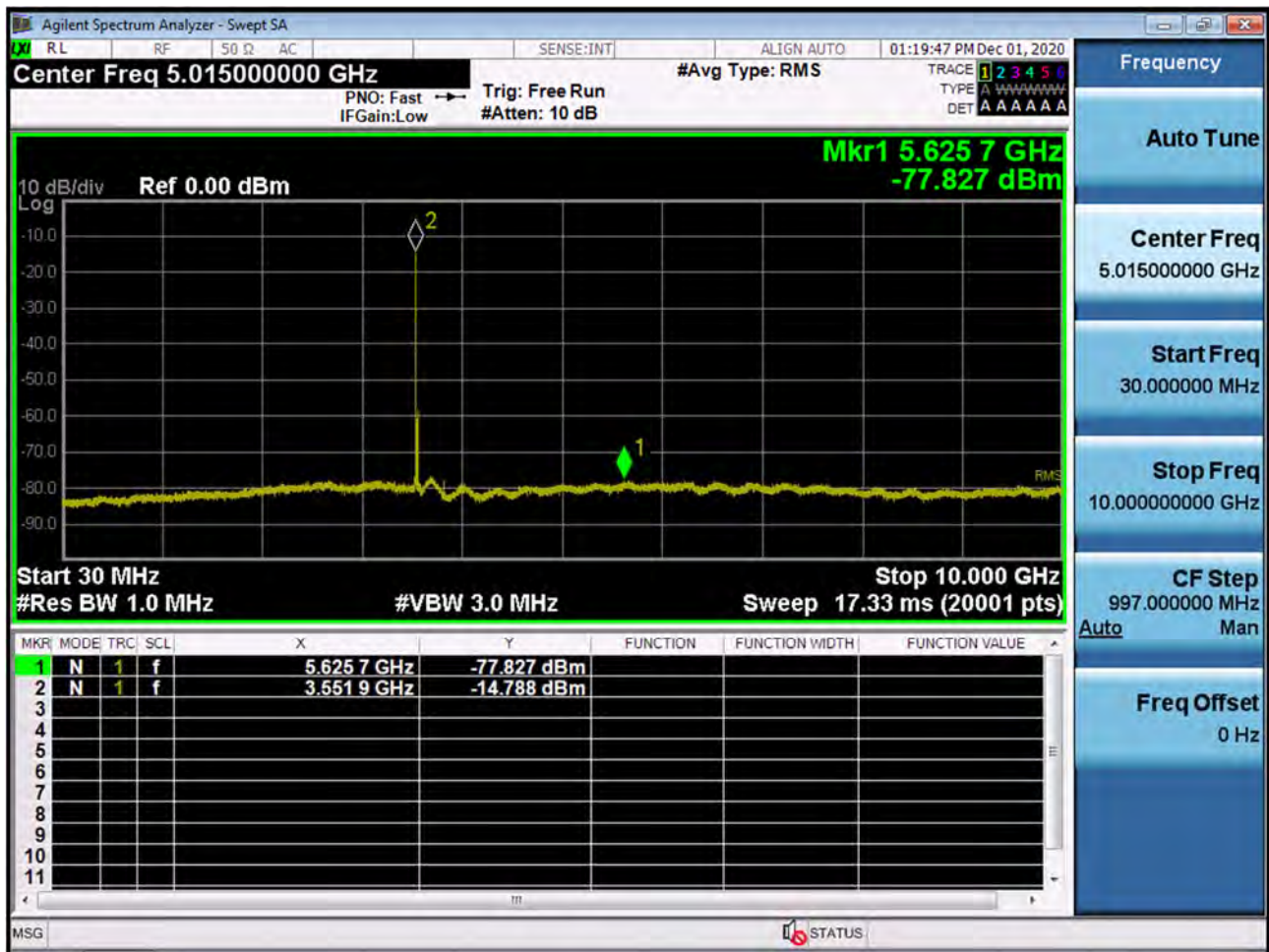
BAND 48. Conducted Spurious Plot 1 (20 MHz Ch.55340 QPSK RB 1, Offset 0)
