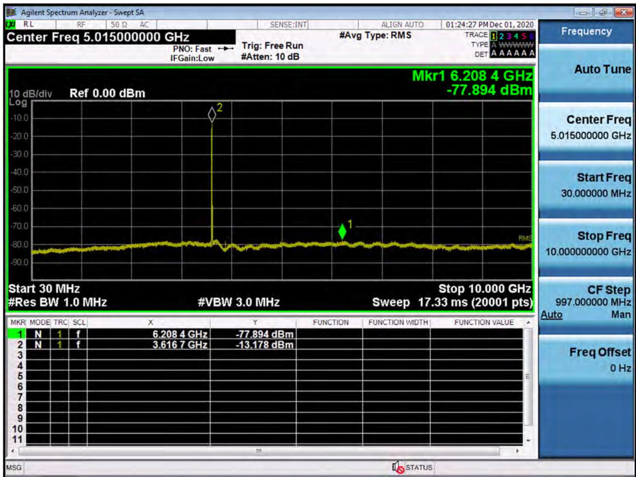
BAND 48. Conducted Spurious Plot 1 (20 MHz Ch.55990 QPSK RB 1, Offset 0)
