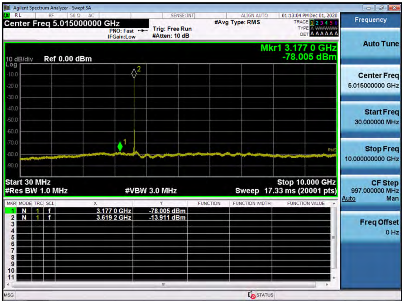
BAND 48. Conducted Spurious Plot 1 (15 MHz Ch.55990 QPSK RB 1, Offset 0)
