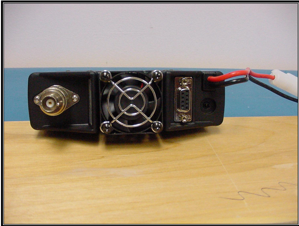
PHOTOGRAPH 9: REAR VIEW OF EUT
