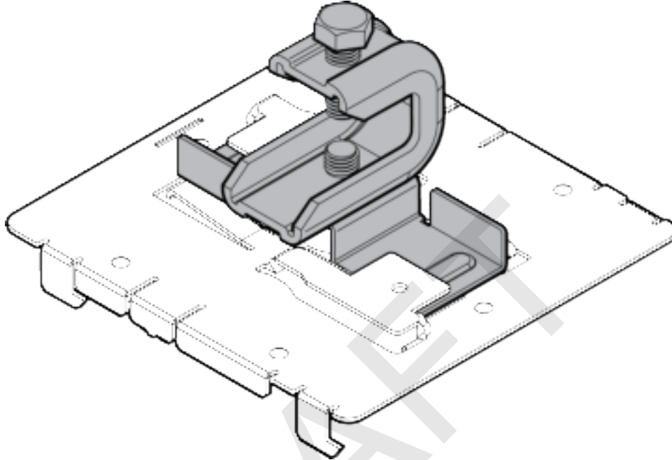
Figure 9: Beam clip accessory attached to the main mounting bracket
