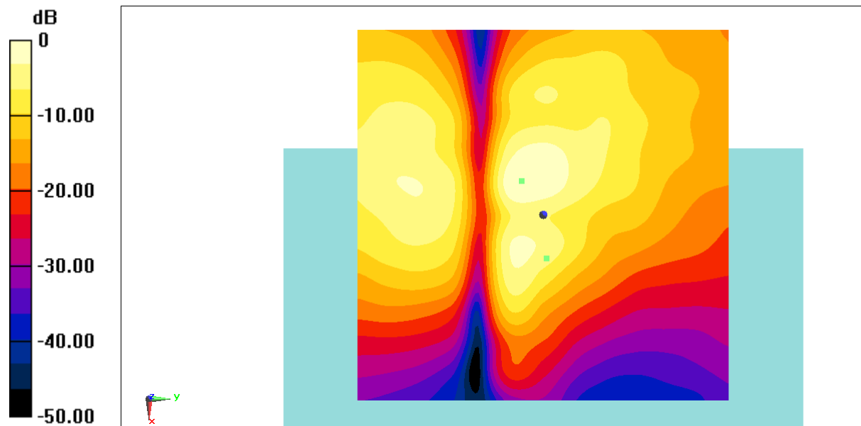
Fig B.11 T-Coil WiFi-2.4G
