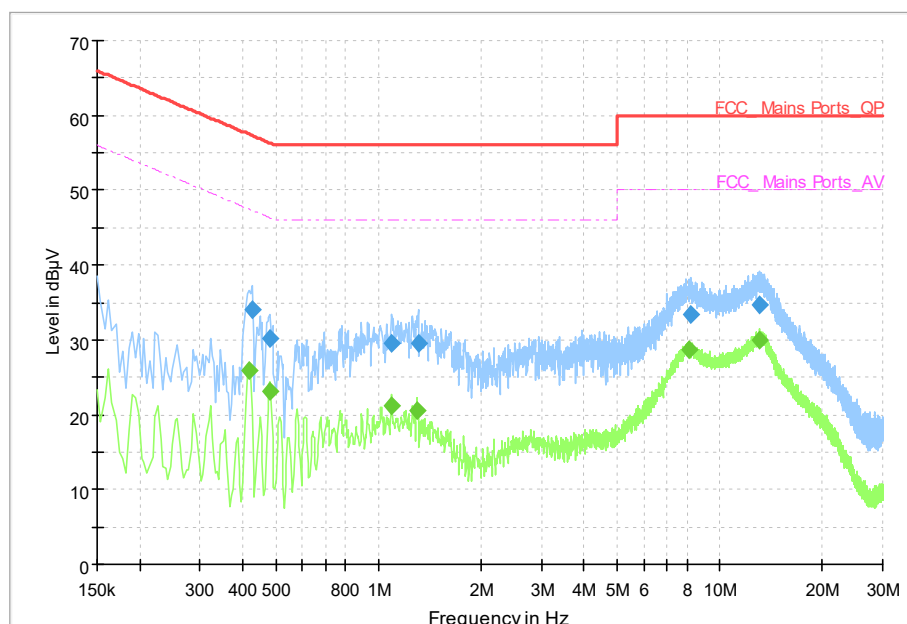
Fig.22 AC Power line Conducted Emission (Idle), LE 1M
