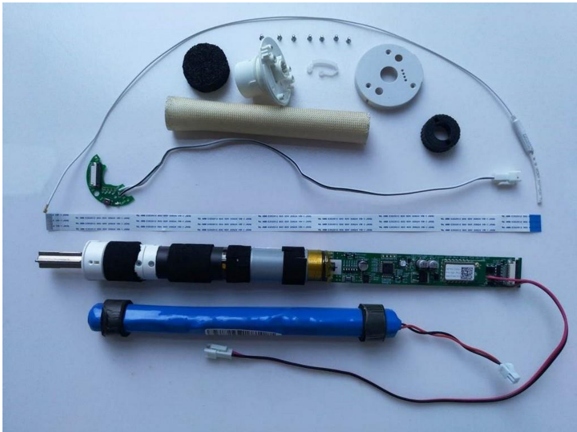
Cover open, Inside View
