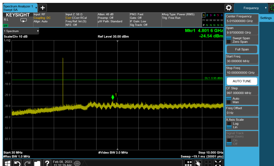
Plot 7-25. Conducted Spurious Plot (Bluetooth, GFSK – Ch. 39)
