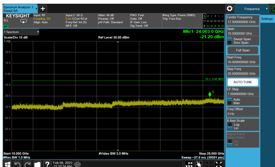
Plot 7-26. Conducted Spurious Plot (Bluetooth, GFSK – Ch. 39)
