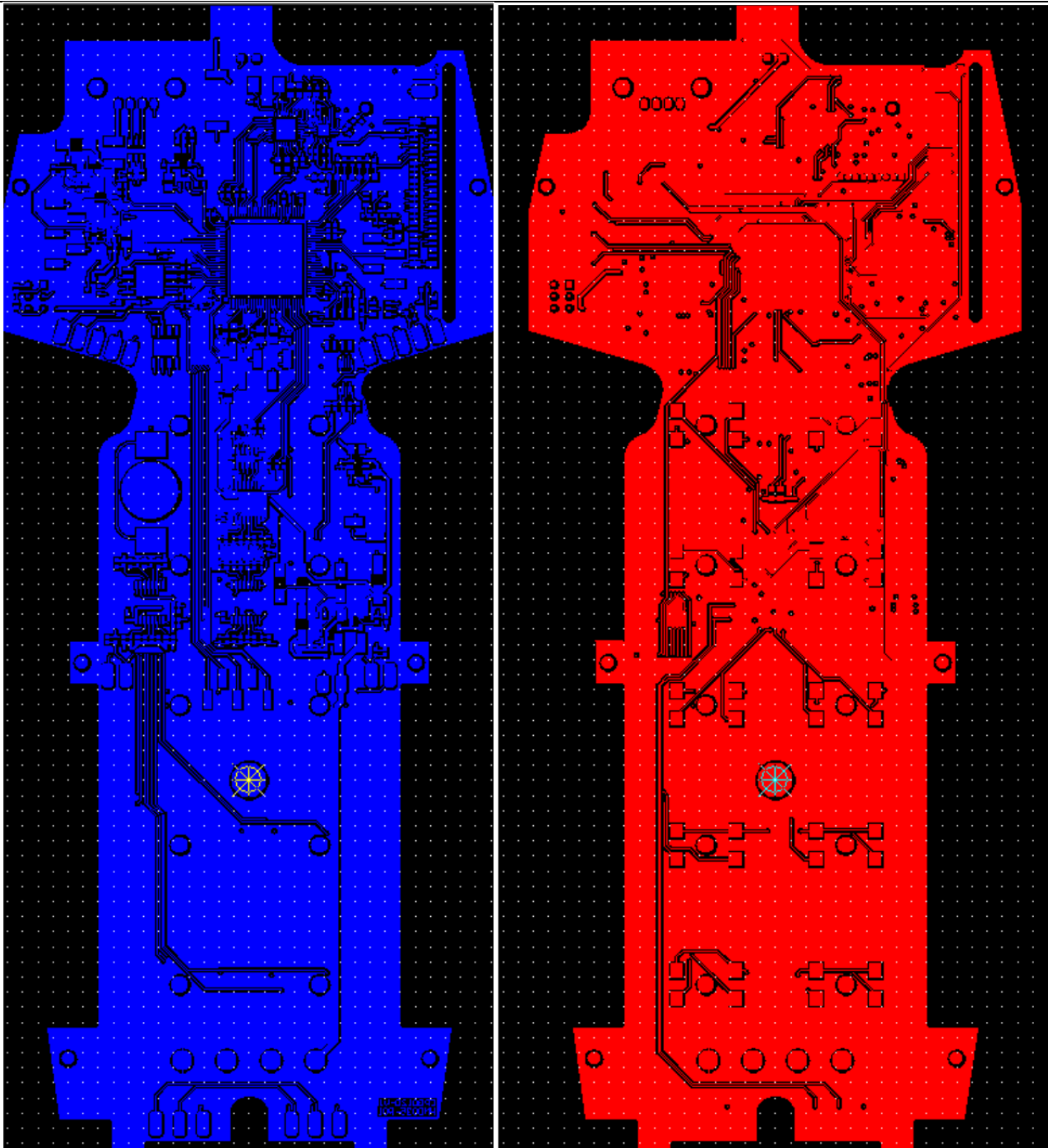
PCB Outer Layers; Left Component Side; Right Button Side
