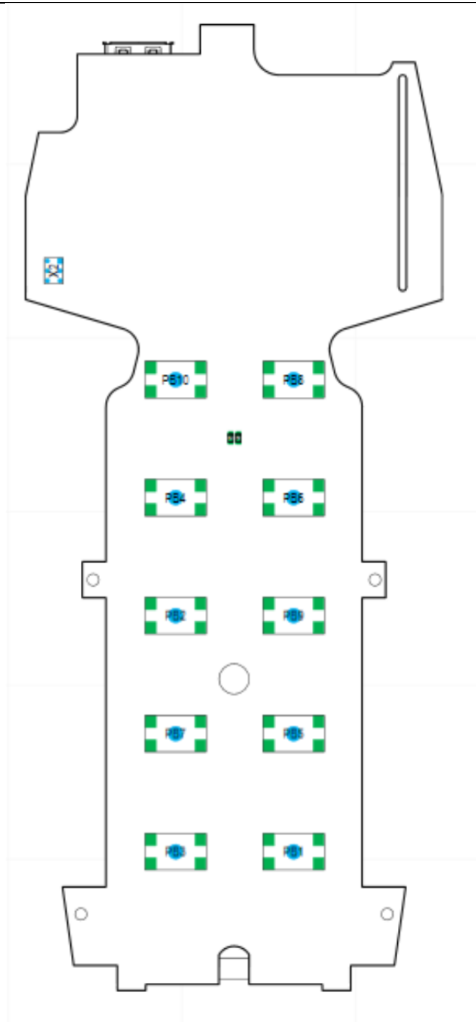
Top Side or Button Side View Drawing
