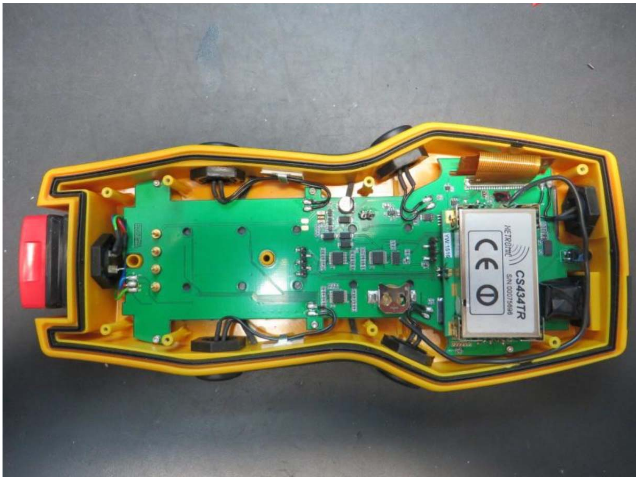
Component Side View; (The CS434TR module visible above is certified separately.) The MFS radio is part of the main board.
