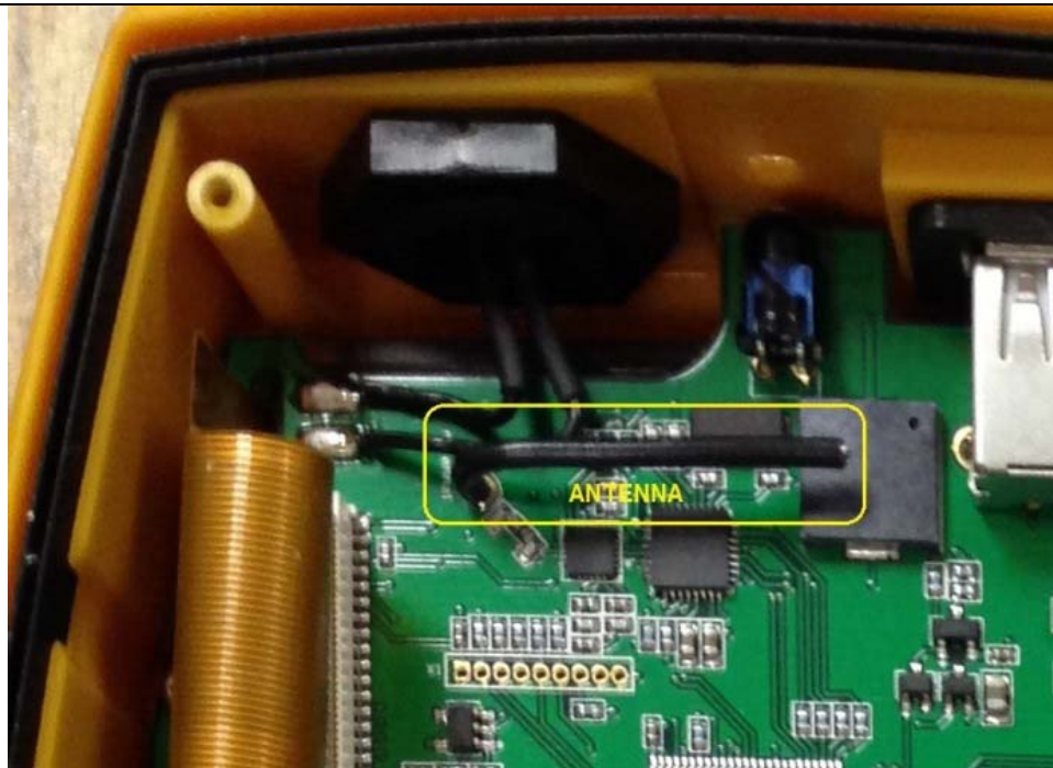
Antenna Detail
