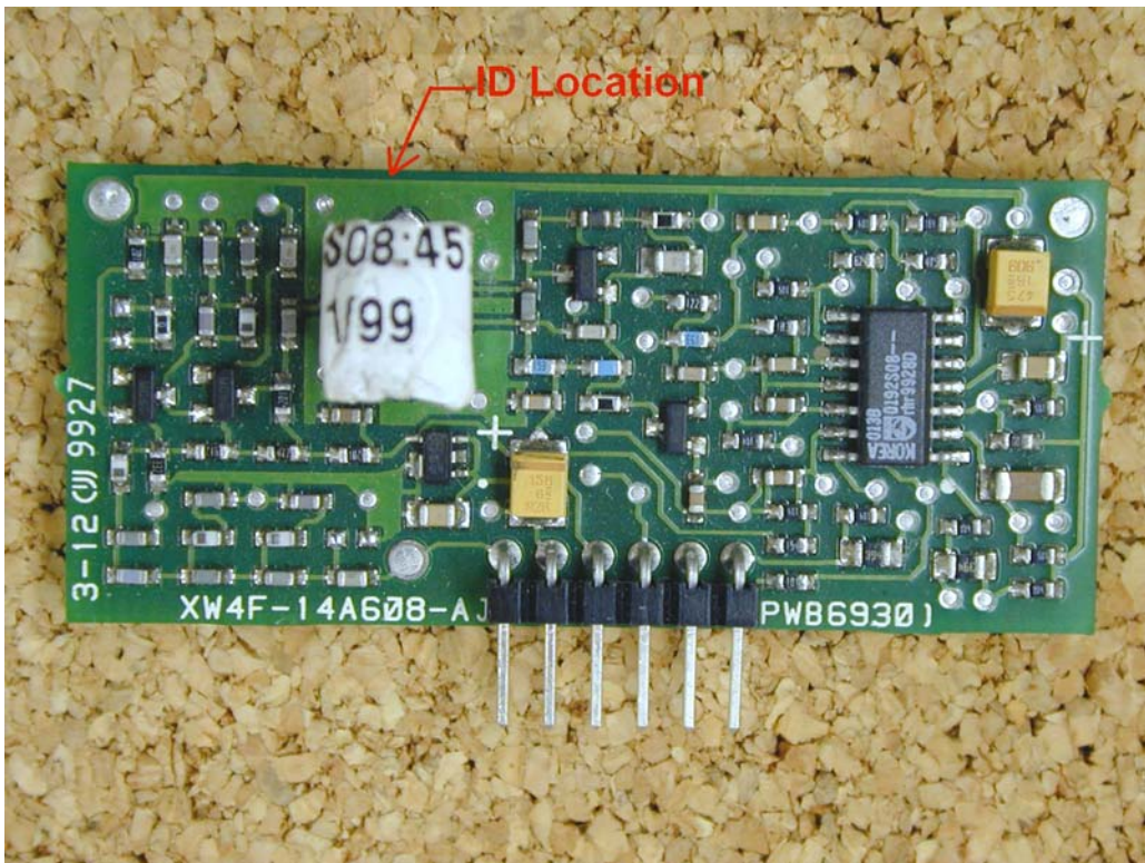
Photo of ID location for receiver
