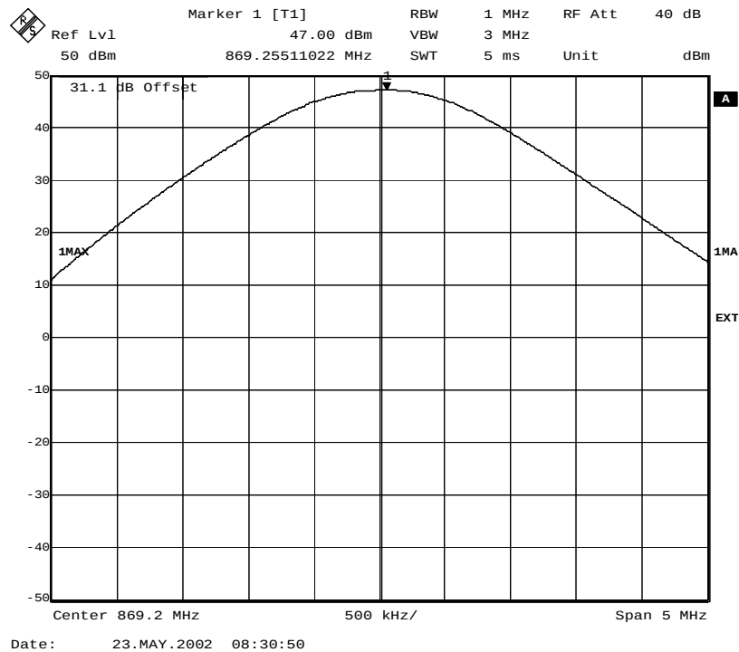
Fig. 4 – RF power at the antenna connector (GMSK modulation).
