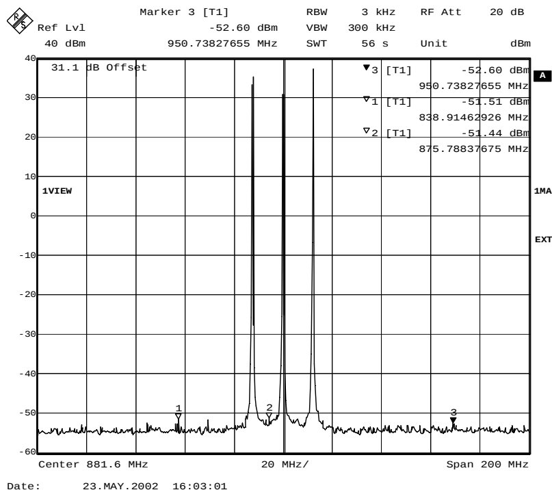
Fig. 53 – Slow frequency hopping – RBW = 3 kHz, reduced video bandwidth VBW = 300kHz (8PSK modulation)
