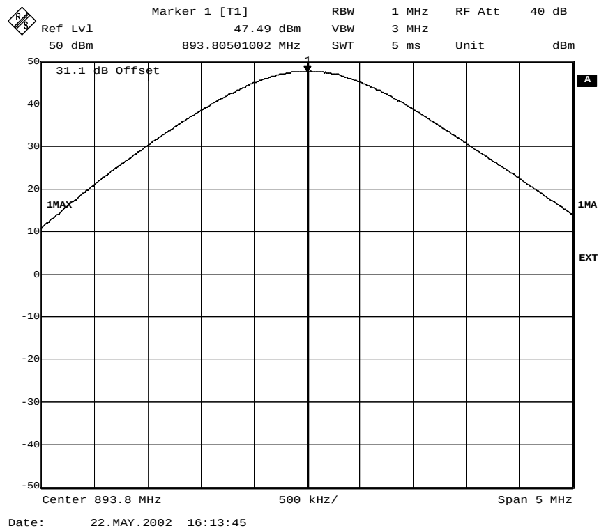
Fig. 9 – RF power at the antenna connector (8PSK modulation).
