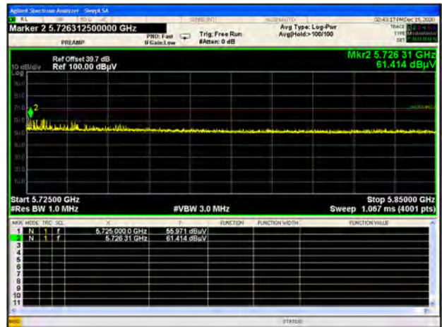
U-NII-2C 11ac20 CH140 Peak
