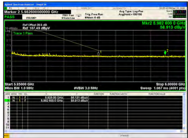
U-NII-3 11a CH165 Peak
