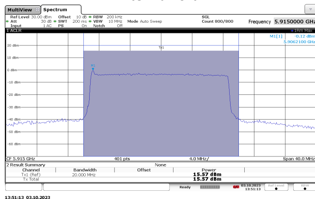
Antenna Port 1
