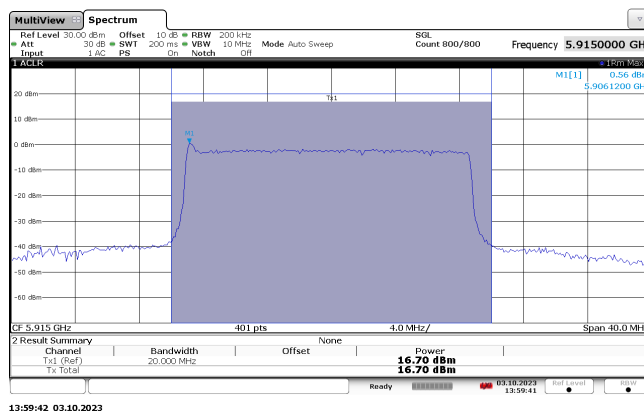
Antenna Port 2
