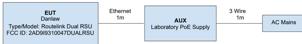
Figure 3.1.1 EUT Test Configuration Diagram.
