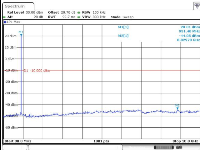
Spurious Emission 30MHz~10GHz Plot
