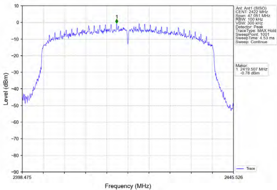
802.11ax(HEW40)_LCH_2422MHz_RU484_Left_Ant1 (SISO)_NTNV
