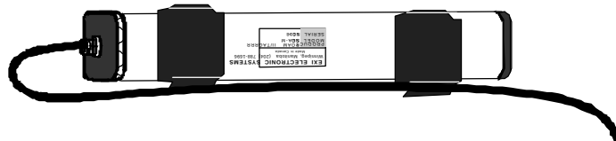
Figure 7 - Securing the Exciter Antenna Cable
