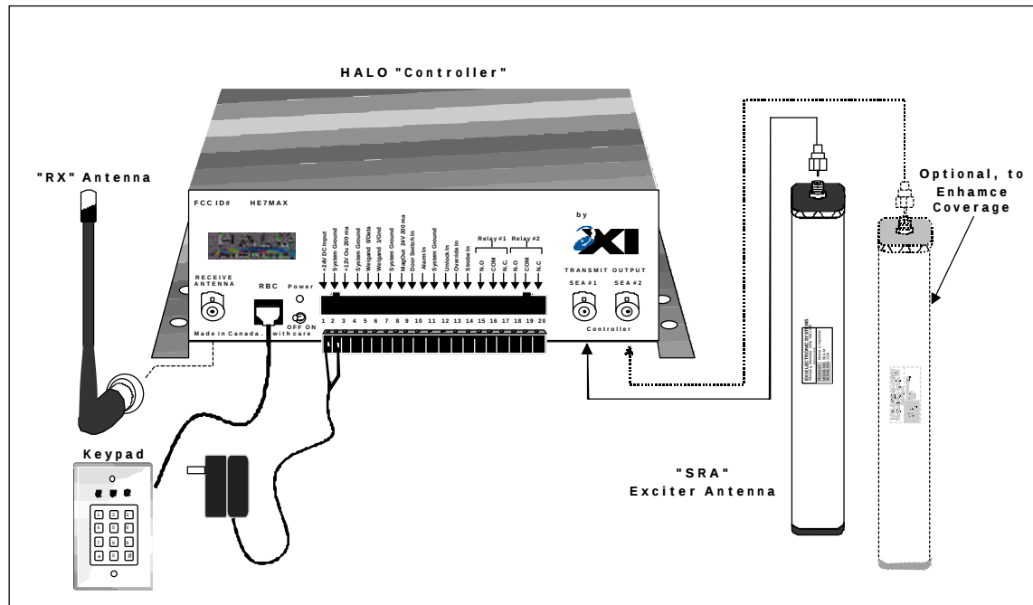
Figure 6 - HALO Controller Typical Hook-up Diagram
