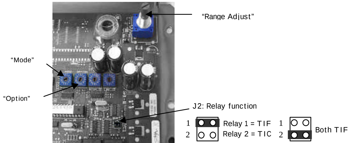
Figure 8 – Controller Switch Identification
