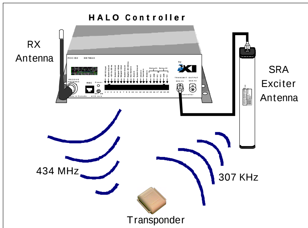
Figure 1 - Controller Operation
