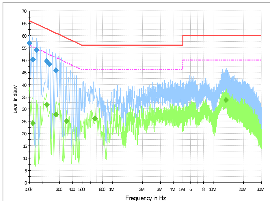
Fig.B.10.2 AC Powerline Conducted Emission-Iidle
