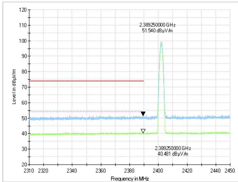
Fig.62. Frequency Band Edges: 8DPSK, Channel 0, 2.31 GHz - 2.45GHz
