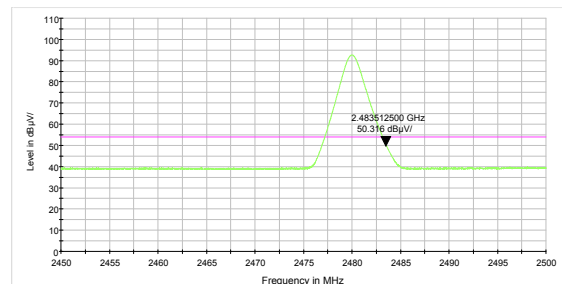
3DH5-Channel 78: Average
