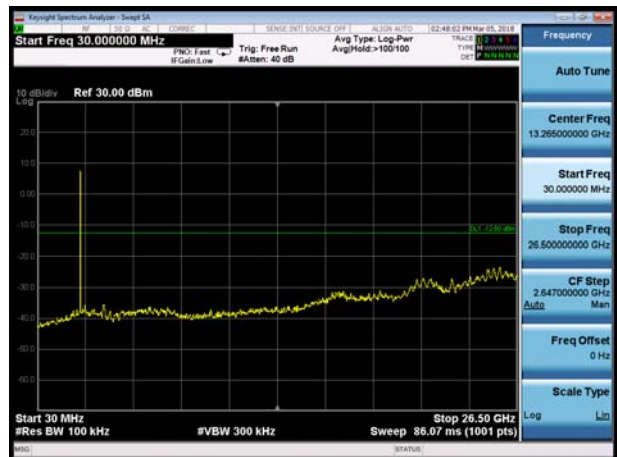
2DH5-CH39 0.03GHz to 26.5GHz
