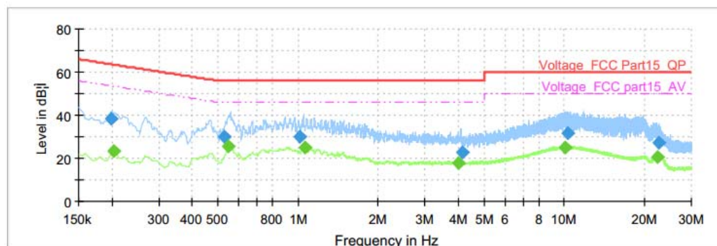
BT_L_0.15-30Mhz
