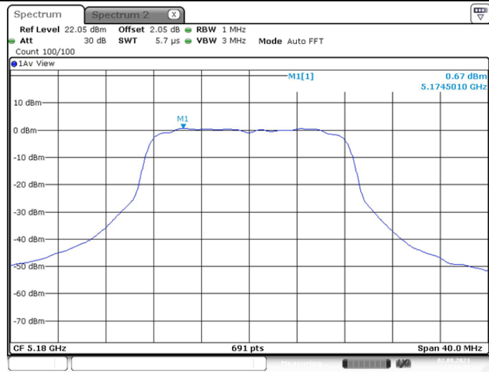
802.11a_5180
