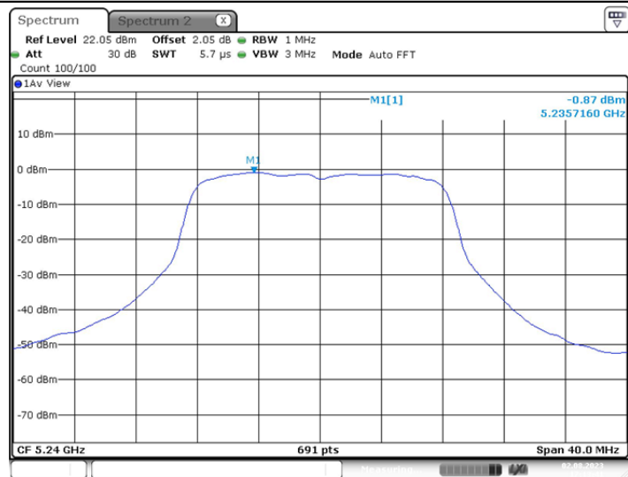
802.11a_5240
