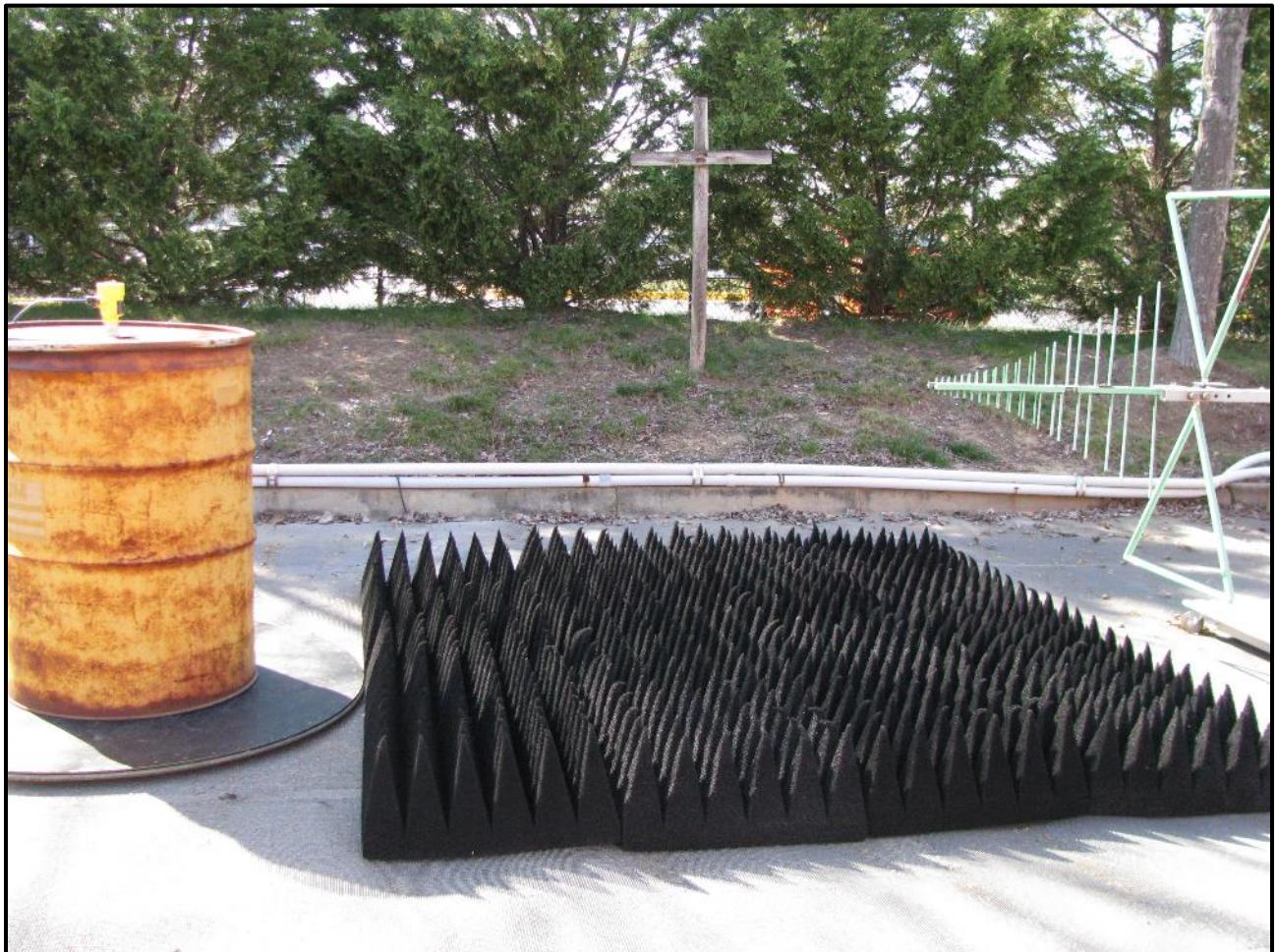
Photograph 19: Radiated Emissions – TC #4; Steel Container, Front View
