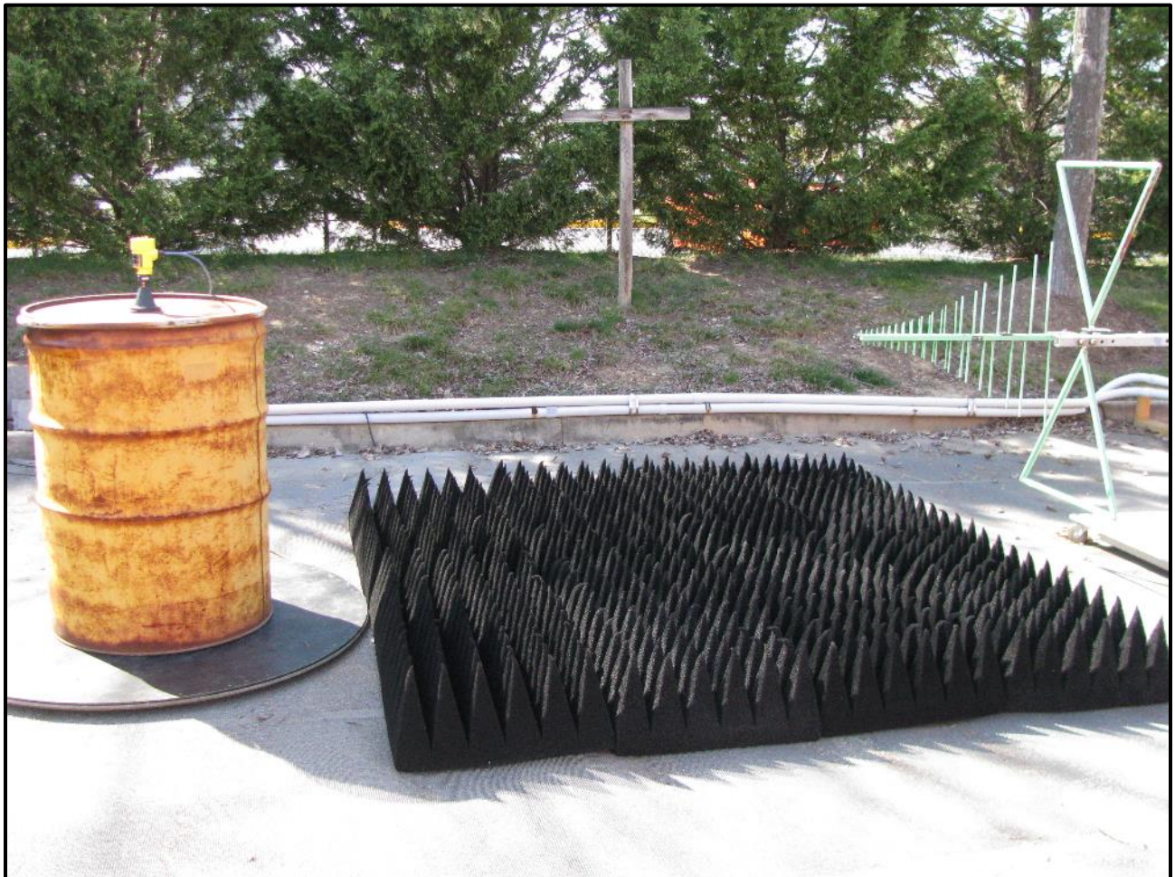
Photograph 13: Radiated Emissions – TC #1; Steel Container, Front View
