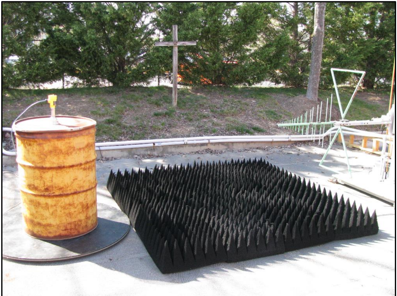
Photograph 30: Radiated Emissions – TC #9; Steel Container, Rear View
