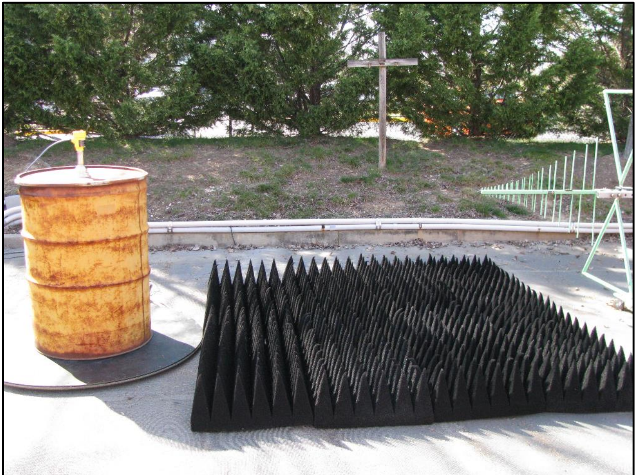
Photograph 29: Radiated Emissions – TC #9; Steel Container, Front View
