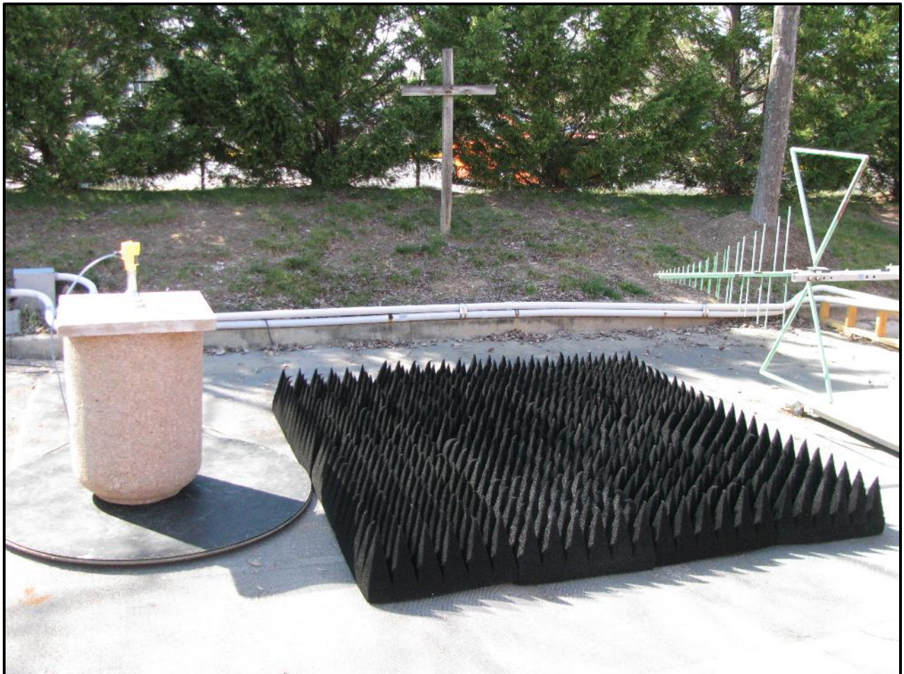
Photograph 44: Radiated Emissions – TC #7; Concrete Container, Rear View
