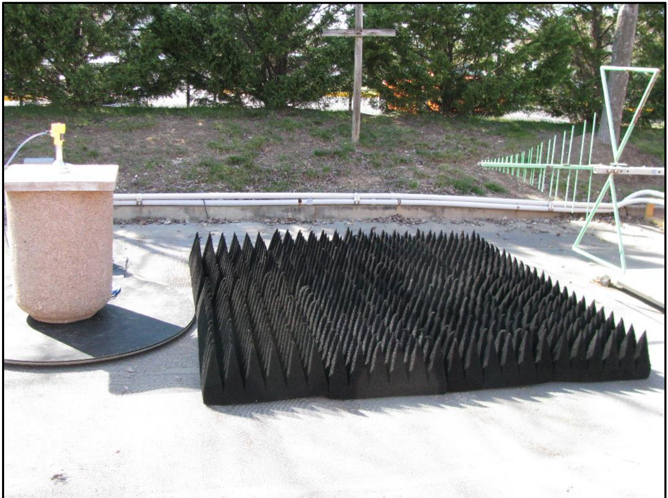
Photograph 48: Radiated Emissions – TC #9; Concrete Container, Rear View
