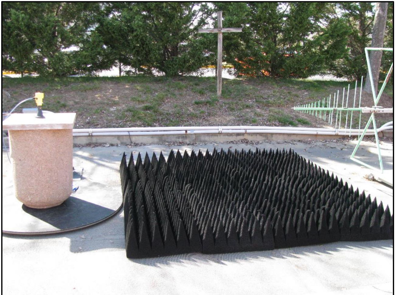
Photograph 31: Radiated Emissions – TC #1; Concrete Container, Front View
