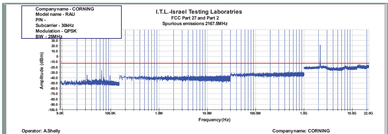
Figure 1037: Spurious Emissions at Antenna Terminal QPSK 25MHz B.W.; 2167.5MHz, 30kHz
