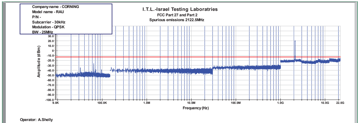
Figure 1035: Spurious Emissions at Antenna Terminal QPSK 25MHz B.W.; 2122.5MHz, 30kHz
