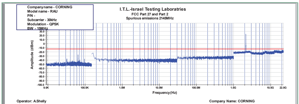
Figure 1018: Spurious Emissions at Antenna Terminal QPSK 15MHz B.W.; 2145.0MHz, 30kHz
