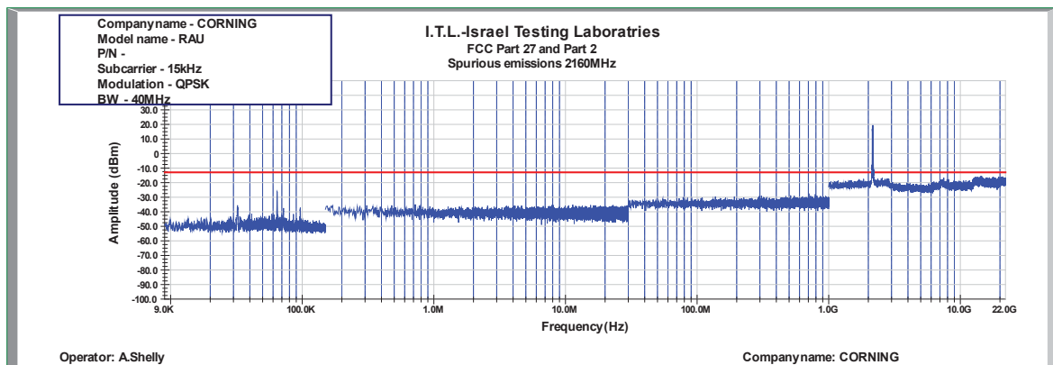
Figure 1043: Spurious Emissions at Antenna Terminal QPSK 40MHz B.W.; 2160.0MHz, 15kHz
