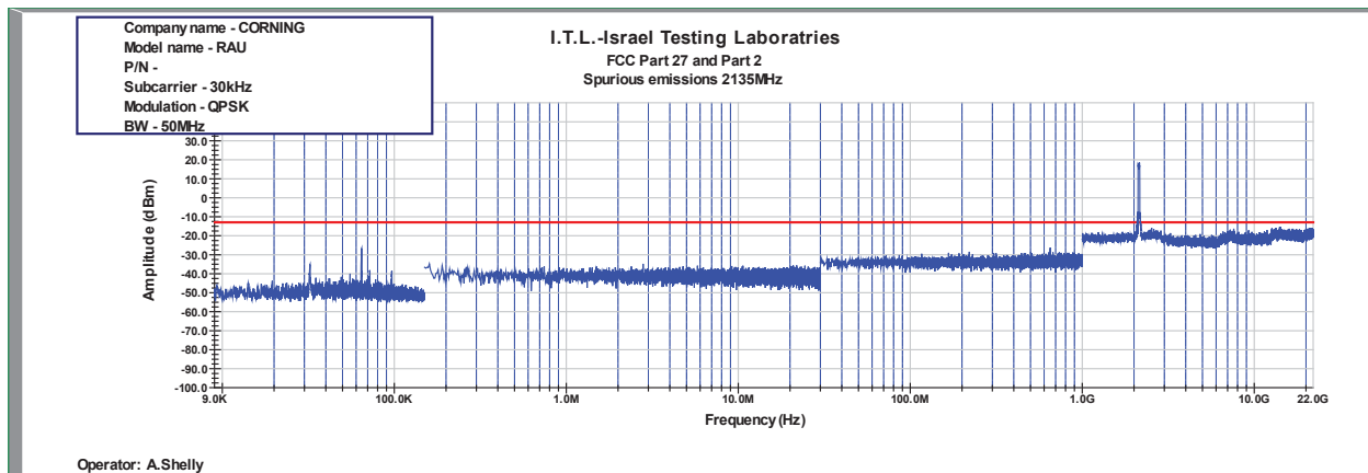
Figure 1053: Spurious Emissions at Antenna Terminal QPSK 50MHz B.W.; 2135.0MHz, 30kHz
