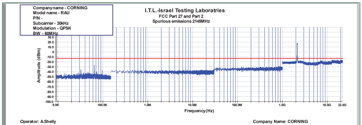
Figure 1060: Spurious Emissions at Antenna Terminal QPSK 60MHz B.W.; 2145.0MHz, 30kHz
