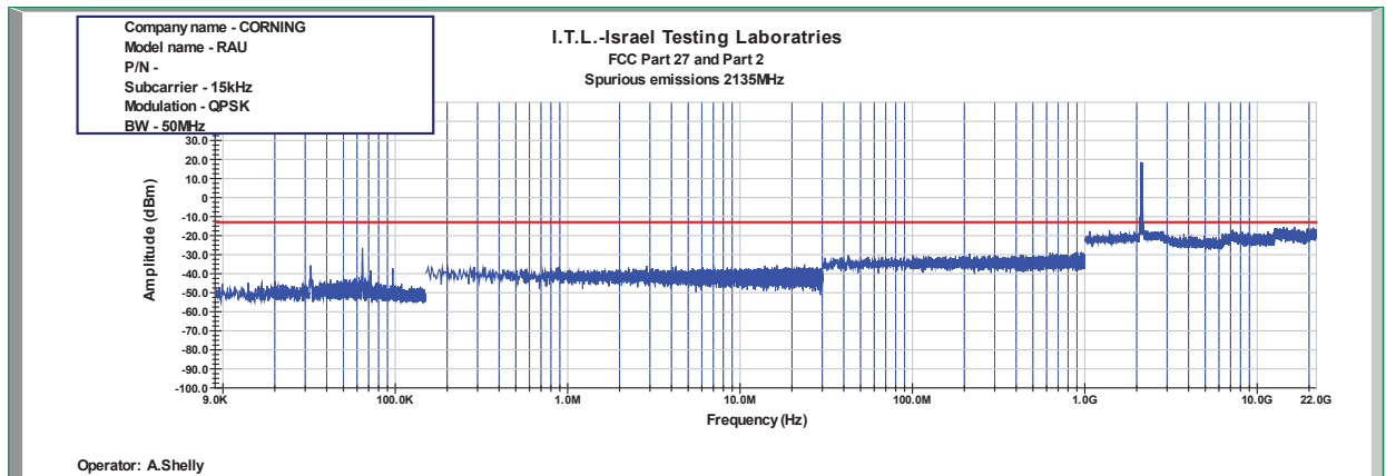
Figure 1050: Spurious Emissions at Antenna Terminal QPSK 50MHz B.W.; 2135.0MHz, 15kHz
