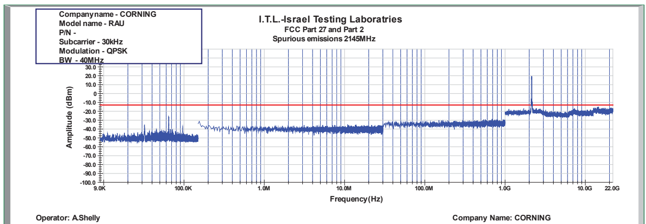
Figure 1045: Spurious Emissions at Antenna Terminal QPSK 40MHz B.W.; 2145.0MHz, 30kHz
