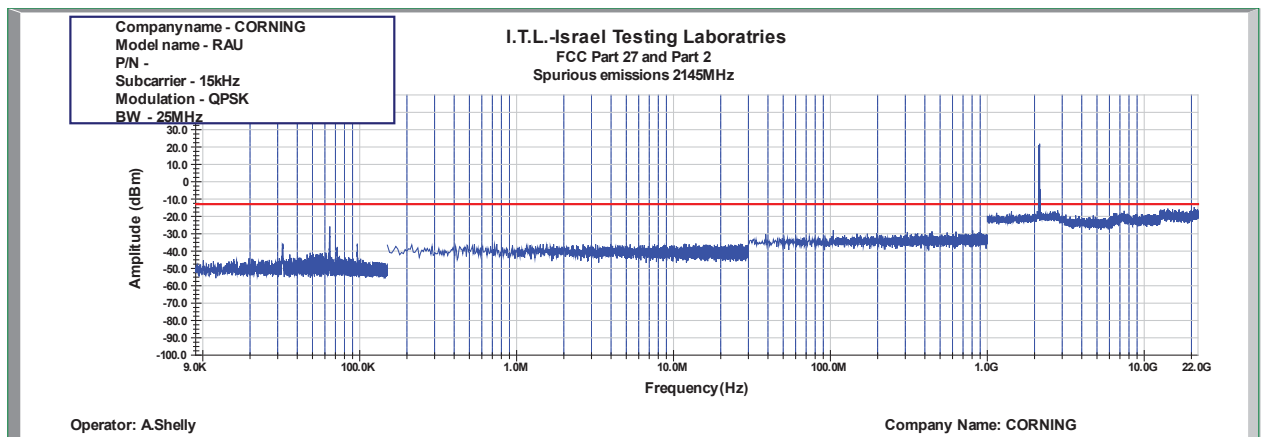
Figure 1033: Spurious Emissions at Antenna Terminal QPSK 25MHz B.W.; 2145.0MHz, 15kHz
