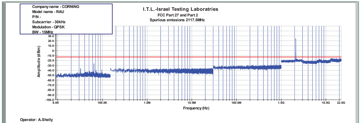
Figure 1017: Spurious Emissions at Antenna Terminal QPSK 15MHz B.W.; 2117.5MHz, 30kHz
