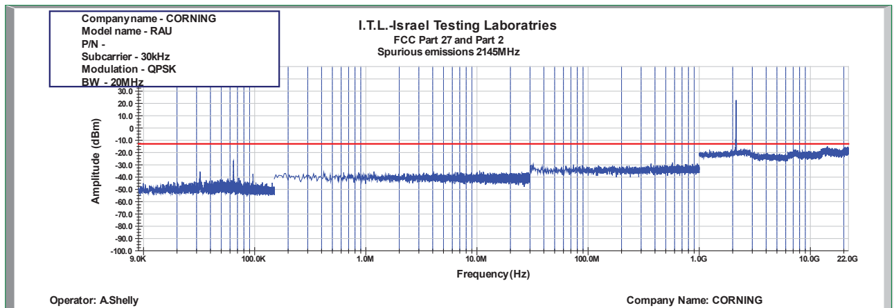
Figure 1027: Spurious Emissions at Antenna Terminal QPSK 20MHz B.W.; 2145.0MHz, 30kHz
