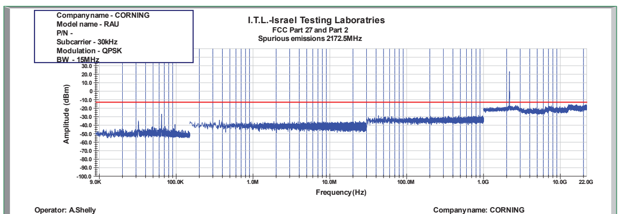
Figure 1019: Spurious Emissions at Antenna Terminal QPSK 15MHz B.W.; 2172.5MHz, 30kHz
