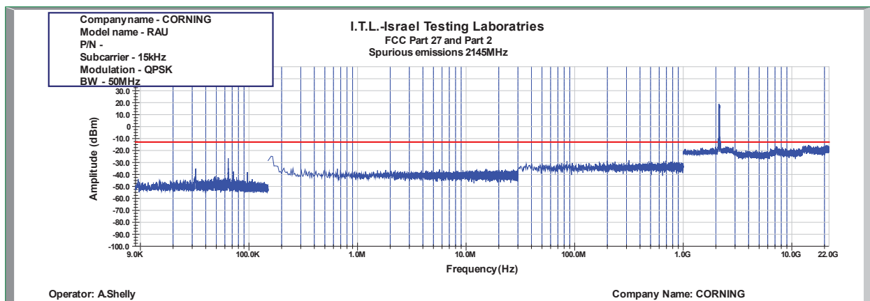
Figure 1051: Spurious Emissions at Antenna Terminal QPSK 50MHz B.W.; 2145.0MHz, 15kHz
