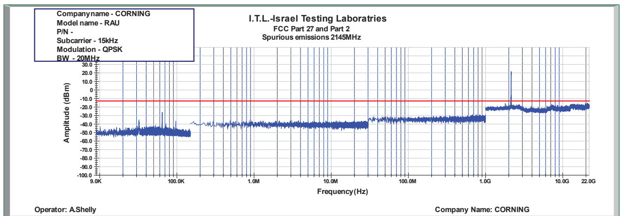
Figure 1024: Spurious Emissions at Antenna Terminal QPSK 20MHz B.W.; 2145.0MHz, 15kHz
