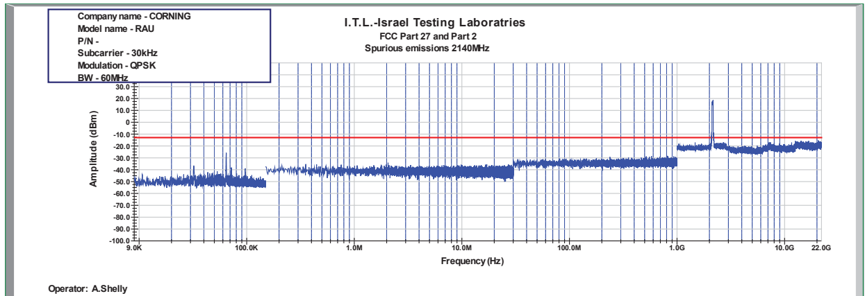
Figure 1059: Spurious Emissions at Antenna Terminal QPSK 60MHz B.W.; 2140.0MHz, 30kHz
