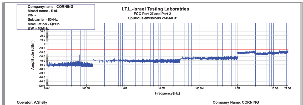
Figure 1012: Spurious Emissions at Antenna Terminal QPSK 10MHz B.W.; 2145.0MHz, 60kHz
