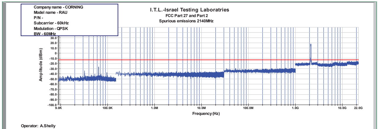
Figure 1062: Spurious Emissions at Antenna Terminal QPSK 60MHz B.W.; 2140.0MHz, 60kHz
