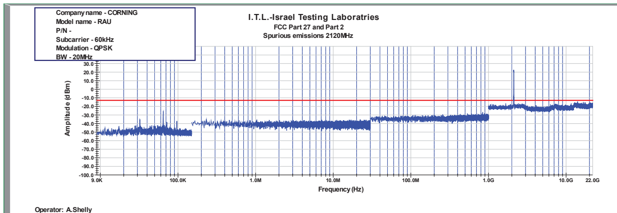
Figure 1029: Spurious Emissions at Antenna Terminal QPSK 20MHz B.W.; 2120.0MHz, 60kHz
