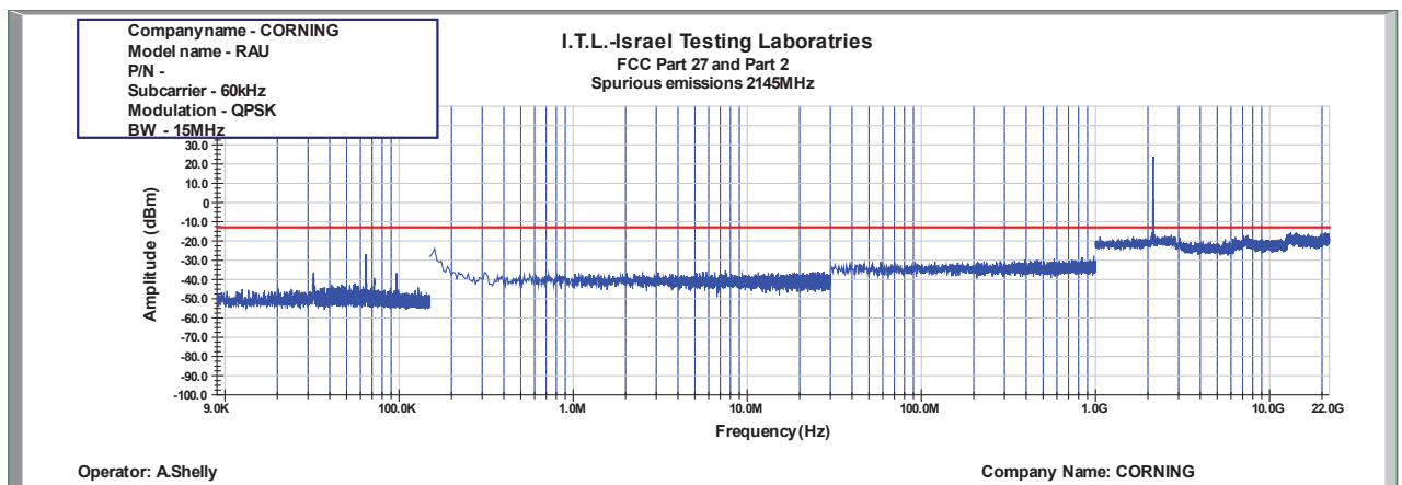
Figure 1021: Spurious Emissions at Antenna Terminal QPSK 15MHz B.W.; 2145.0MHz, 60kHz
