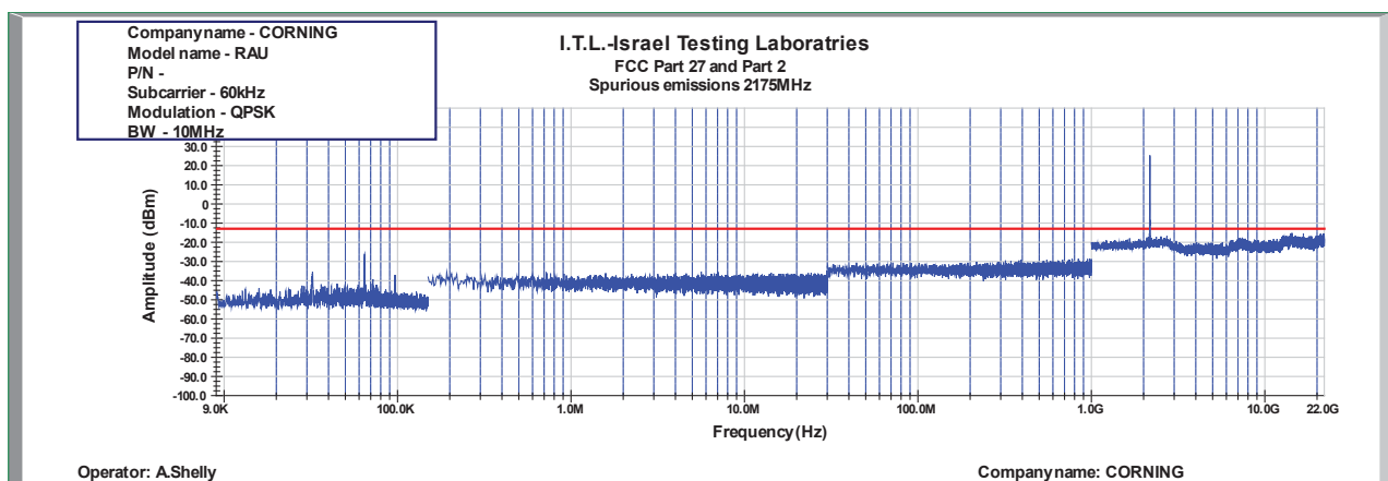
Figure 1013: Spurious Emissions at Antenna Terminal QPSK 10MHz B.W.; 2175.0MHz, 60kHz
