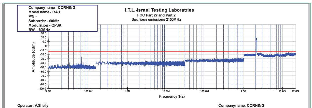
Figure 1064: Spurious Emissions at Antenna Terminal QPSK 60MHz B.W.; 2150.0MHz, 60kHz
