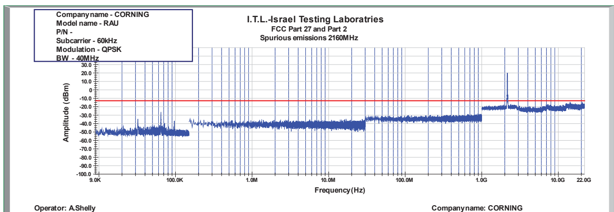
Figure 1049: Spurious Emissions at Antenna Terminal QPSK 40MHz B.W.; 2160.0MHz, 60kHz
