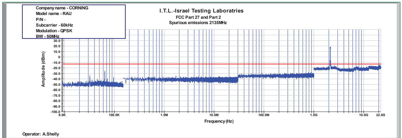
Figure 1056: Spurious Emissions at Antenna Terminal QPSK 50MHz B.W.; 2135.0MHz, 60kHz
