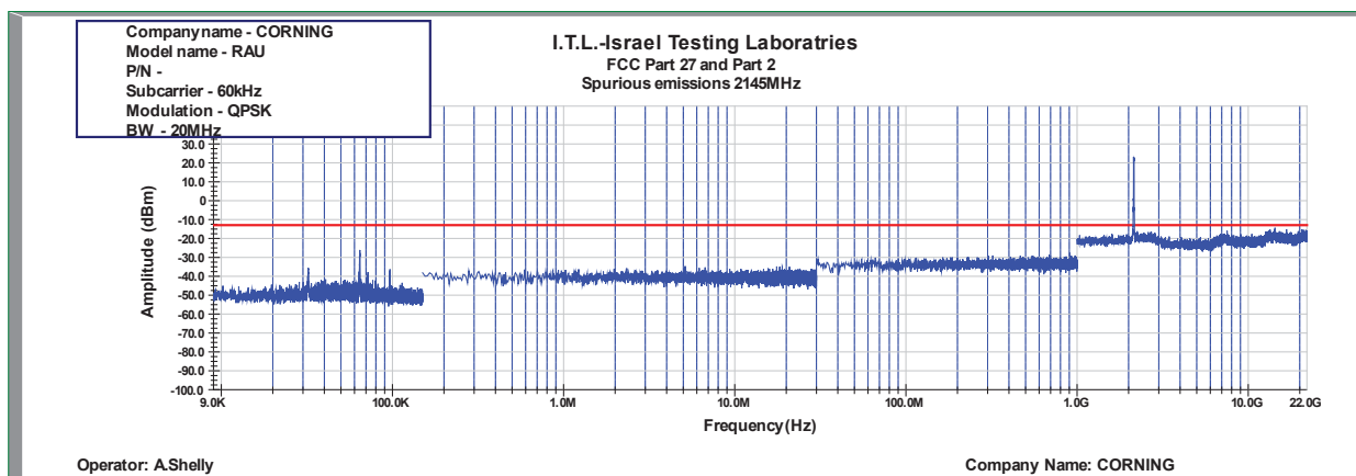
Figure 1030: Spurious Emissions at Antenna Terminal QPSK 20MHz B.W.; 2145.0MHz, 60kHz
