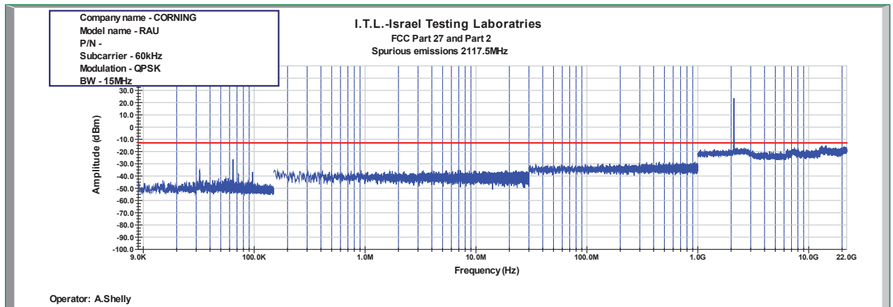
Figure 1020: Spurious Emissions at Antenna Terminal QPSK 15MHz B.W.; 2117.5MHz, 60kHz
