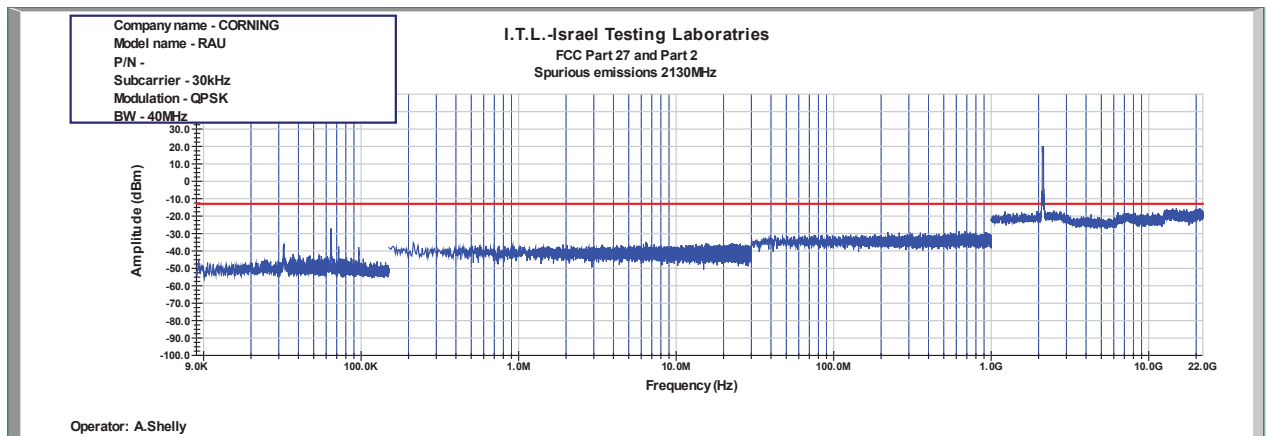
Figure 1044: Spurious Emissions at Antenna Terminal QPSK 40MHz B.W.; 2130.0MHz, 30kHz
