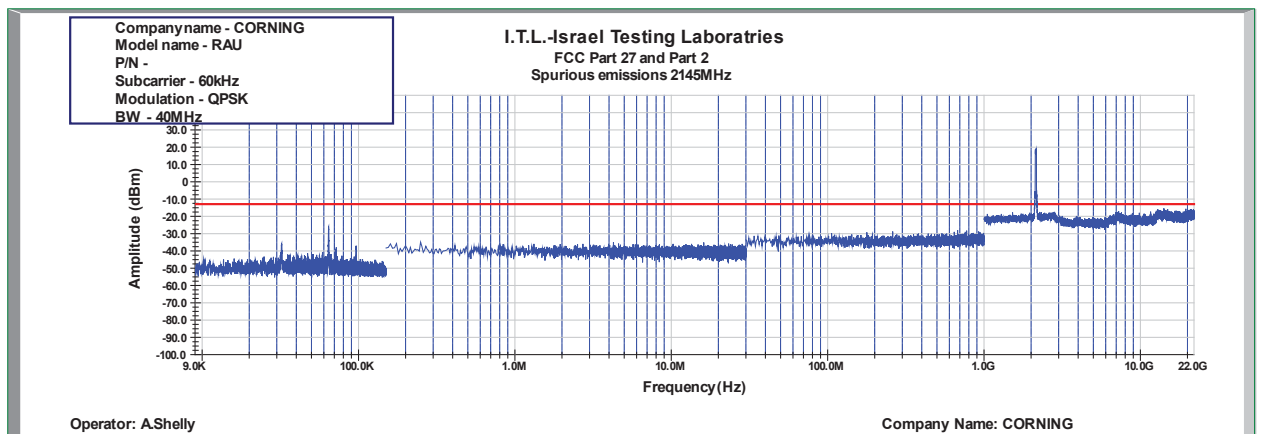
Figure 1048: Spurious Emissions at Antenna Terminal QPSK 40MHz B.W.; 2145.0MHz, 60kHz
