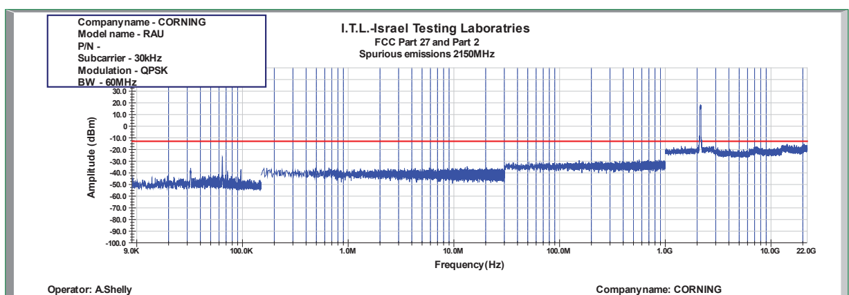
Figure 1061: Spurious Emissions at Antenna Terminal QPSK 60MHz B.W.; 2150.0MHz, 30kHz
