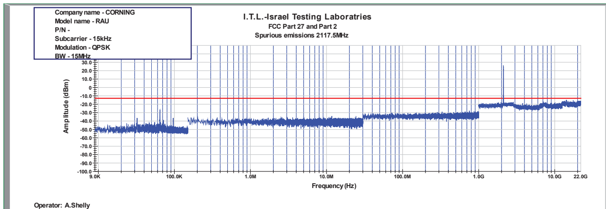
Figure 1014: Spurious Emissions at Antenna Terminal QPSK 15MHz B.W.; 2117.5MHz, 15kHz
