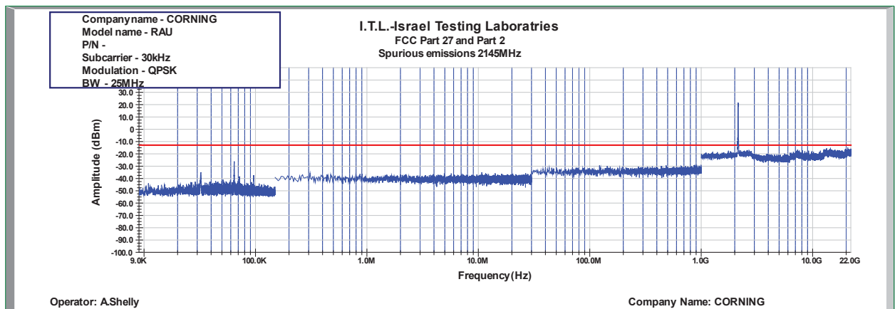
Figure 1036: Spurious Emissions at Antenna Terminal QPSK 25MHz B.W.; 2145.0MHz, 30kHz
