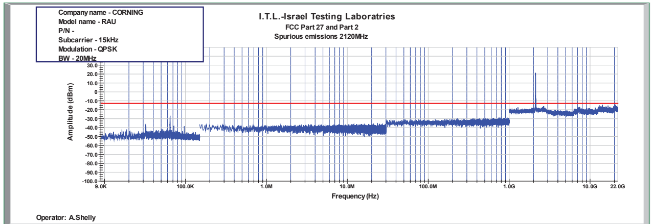
Figure 1023: Spurious Emissions at Antenna Terminal QPSK 20MHz B.W.; 2120.0MHz, 15kHz
