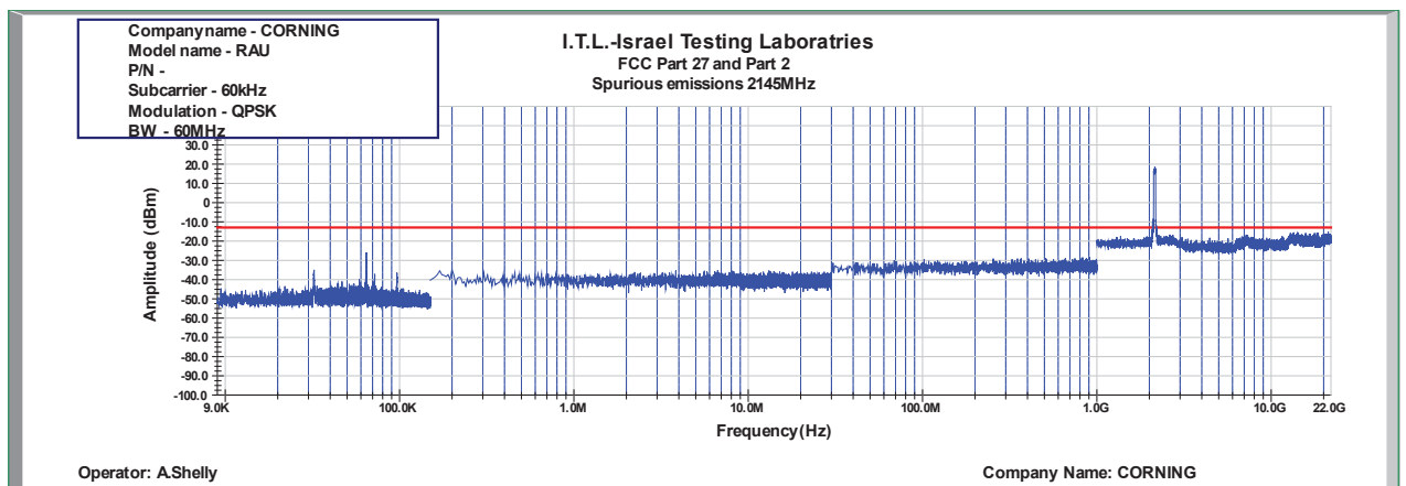
Figure 1063: Spurious Emissions at Antenna Terminal QPSK 60MHz B.W.; 2145.0MHz, 60kHz
