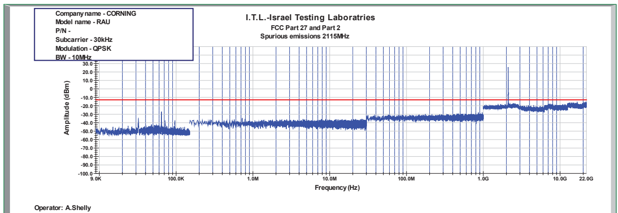
Figure 1008: Spurious Emissions at Antenna Terminal QPSK 10MHz B.W.; 2115.0MHz, 30kHz
