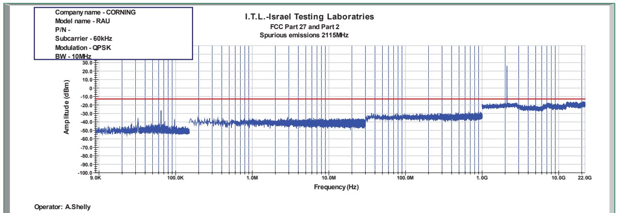
Figure 1011: Spurious Emissions at Antenna Terminal QPSK 10MHz B.W.; 2115.0MHz, 60kHz
