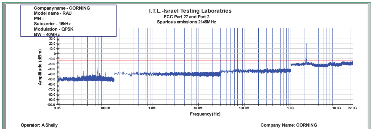
Figure 1042: Spurious Emissions at Antenna Terminal QPSK 40MHz B.W.; 2145.0MHz, 15kHz
