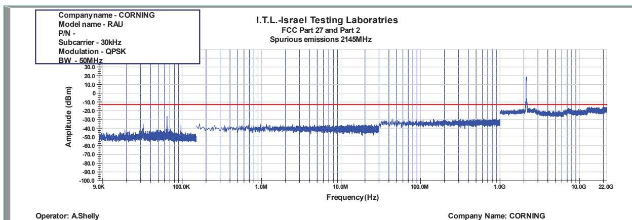
Figure 1054: Spurious Emissions at Antenna Terminal QPSK 50MHz B.W.; 2145.0MHz, 30kHz
