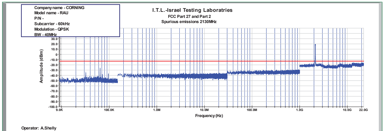
Figure 1047: Spurious Emissions at Antenna Terminal QPSK 40MHz B.W.; 2130.0MHz, 60kHz
