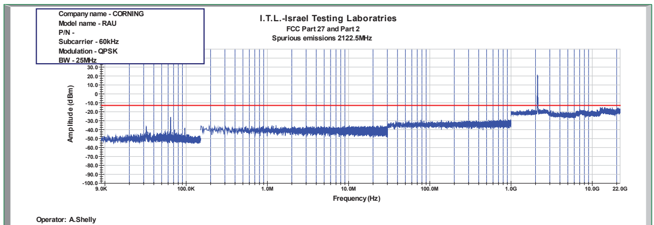
Figure 1038: Spurious Emissions at Antenna Terminal QPSK 25MHz B.W.; 2122.5MHz, 60kHz
