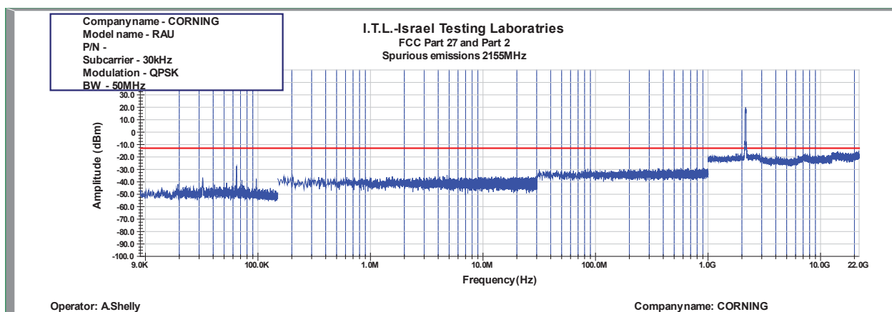
Figure 1055: Spurious Emissions at Antenna Terminal QPSK 50MHz B.W.; 2155.0MHz, 30kHz
