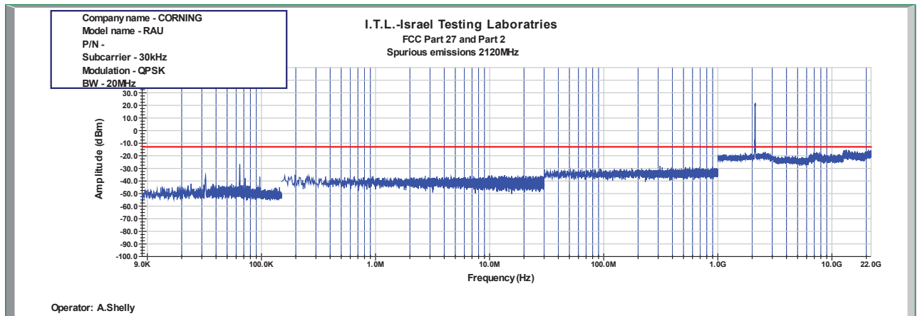
Figure 1026: Spurious Emissions at Antenna Terminal QPSK 20MHz B.W.; 2120.0MHz, 30kHz
