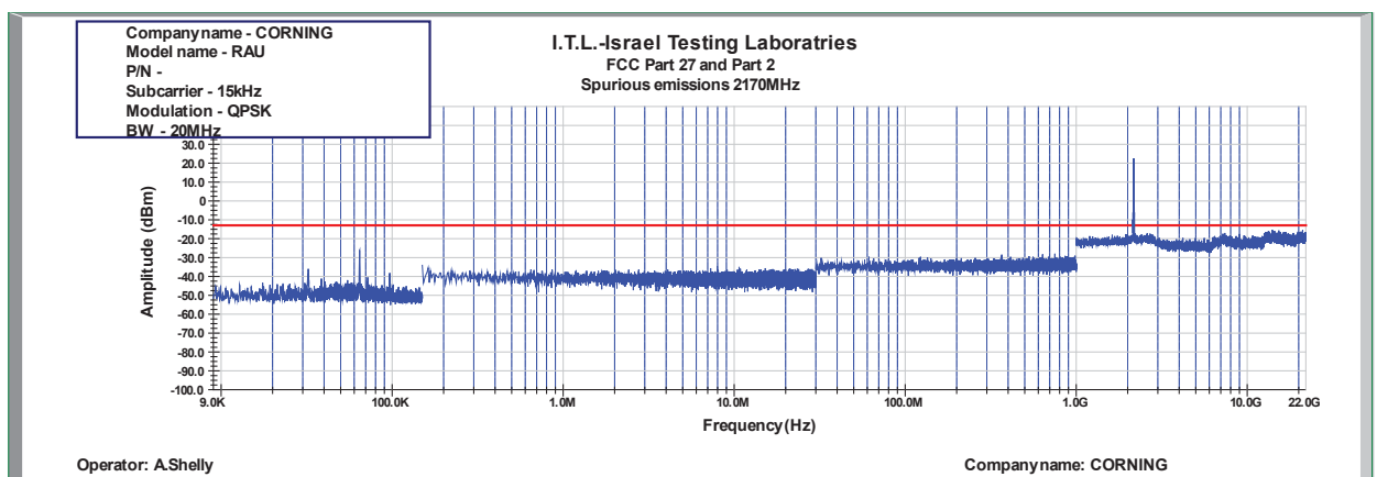
Figure 1025: Spurious Emissions at Antenna Terminal QPSK 20MHz B.W.; 2170.0MHz, 15kHz
