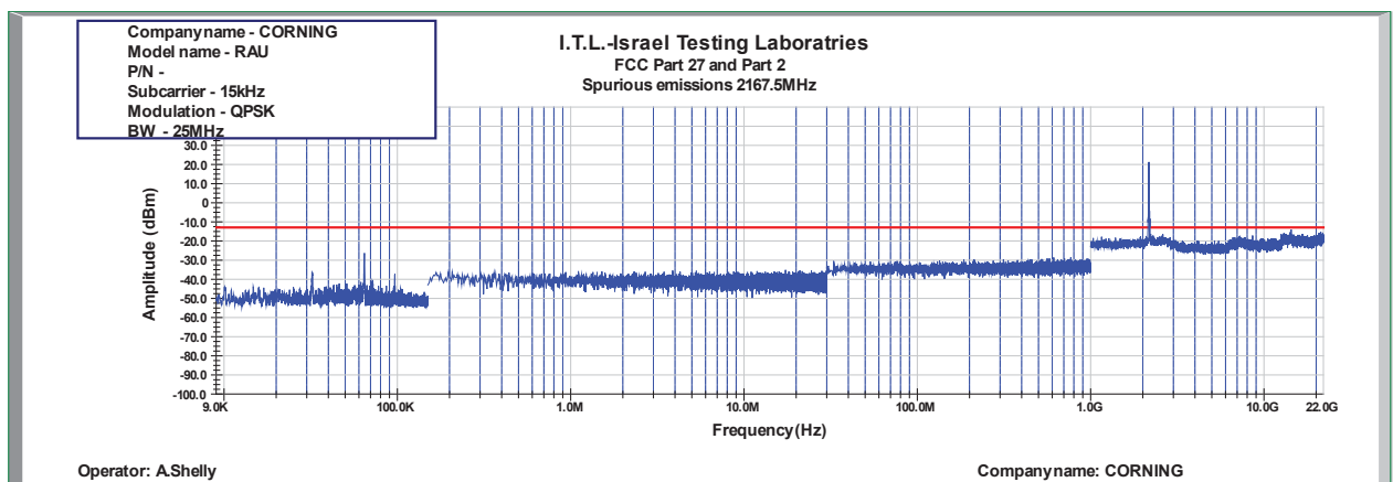
Figure 1034: Spurious Emissions at Antenna Terminal QPSK 25MHz B.W.; 2167.5MHz, 15kHz
