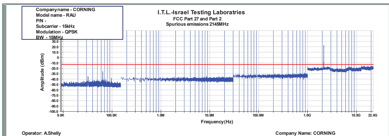
Figure 1015: Spurious Emissions at Antenna Terminal QPSK 15MHz B.W.; 2145.0MHz, 15kHz
