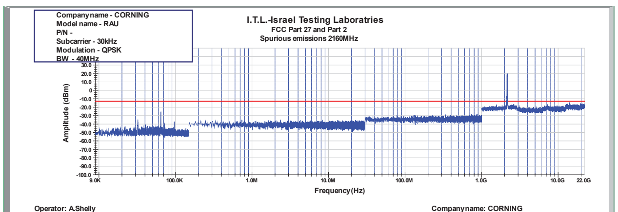
Figure 1046: Spurious Emissions at Antenna Terminal QPSK 40MHz B.W.; 2160.0MHz, 30kHz
