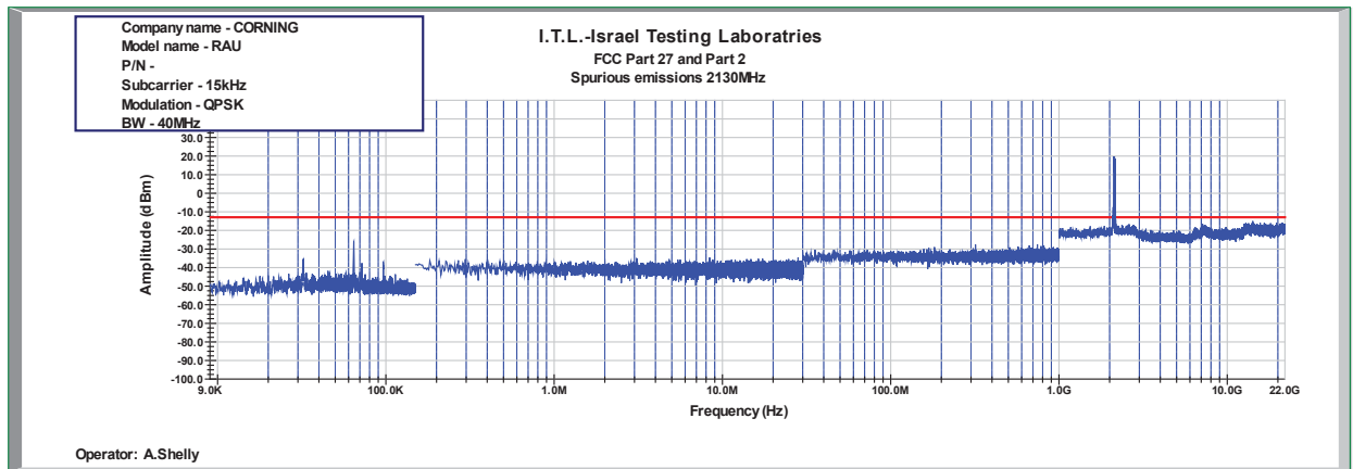
Figure 1041: Spurious Emissions at Antenna Terminal QPSK 40MHz B.W.; 2130.0MHz, 15kHz
