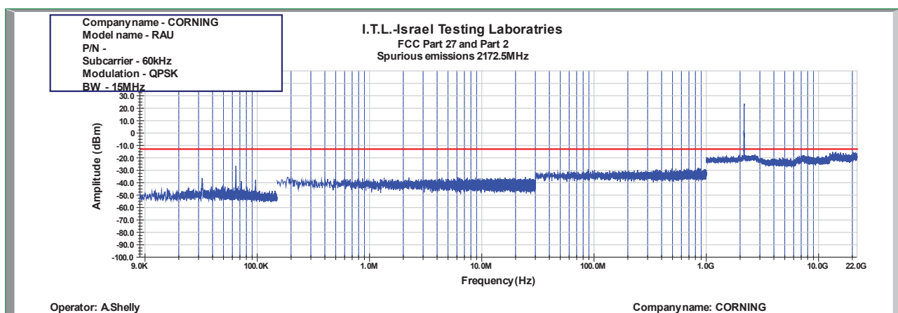
Figure 1022: Spurious Emissions at Antenna Terminal QPSK 15MHz B.W.; 2172.5MHz, 60kHz
