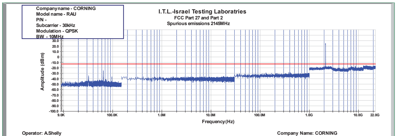
Figure 1009: Spurious Emissions at Antenna Terminal QPSK 10MHz B.W.; 2145.0MHz, 30kHz
