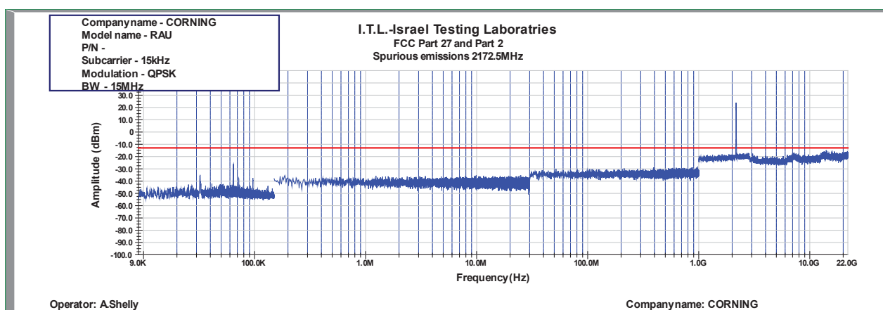
Figure 1016: Spurious Emissions at Antenna Terminal QPSK 15MHz B.W.; 2172.5MHz, 15kHz
