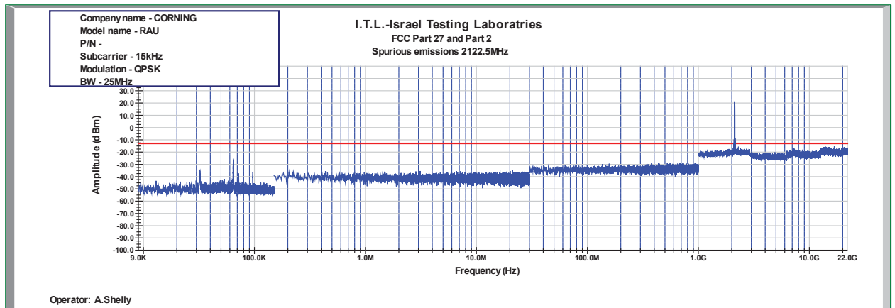
Figure 1032: Spurious Emissions at Antenna Terminal QPSK 25MHz B.W.; 2122.5MHz, 15kHz
