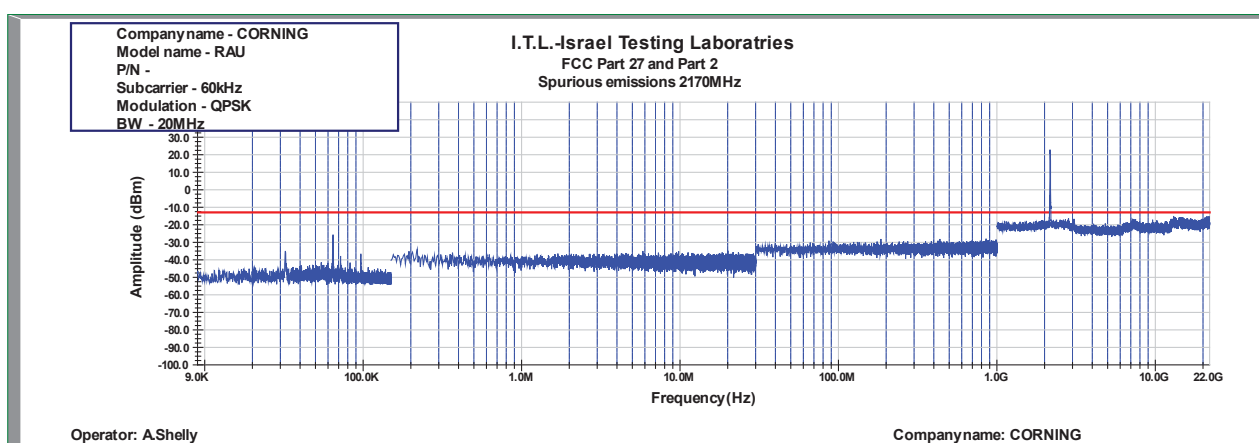
Figure 1031: Spurious Emissions at Antenna Terminal QPSK 20MHz B.W.; 2170.0MHz, 60kHz
