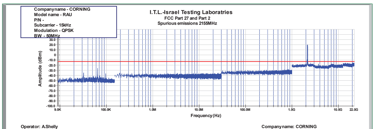
Figure 1052: Spurious Emissions at Antenna Terminal QPSK 50MHz B.W.; 2155.0MHz, 15kHz
