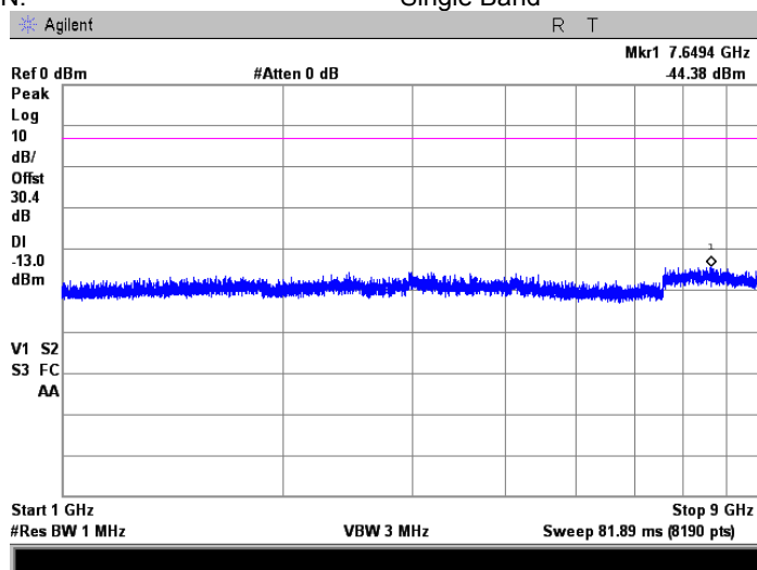
Plot 7.8.108 Spurious emission measurements in 1000 - 9000 MHz at high carrier frequency
