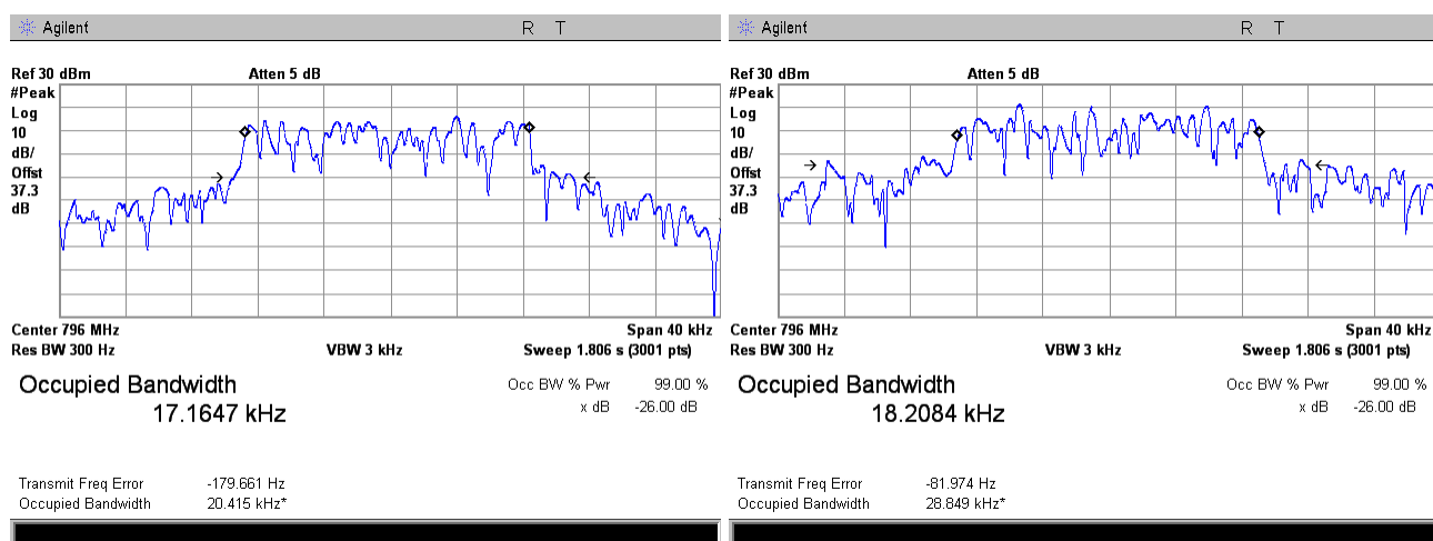
Plot 7.2.18 Occupied bandwidth test result at low frequency carrier, Port 2
