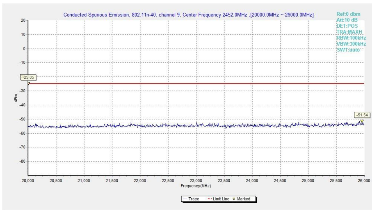
Fig.A.6.1.95 Transmitter Spurious Emission - Conducted (802.11n-HT40, Ch9, 20 GHz-26 GHz)
