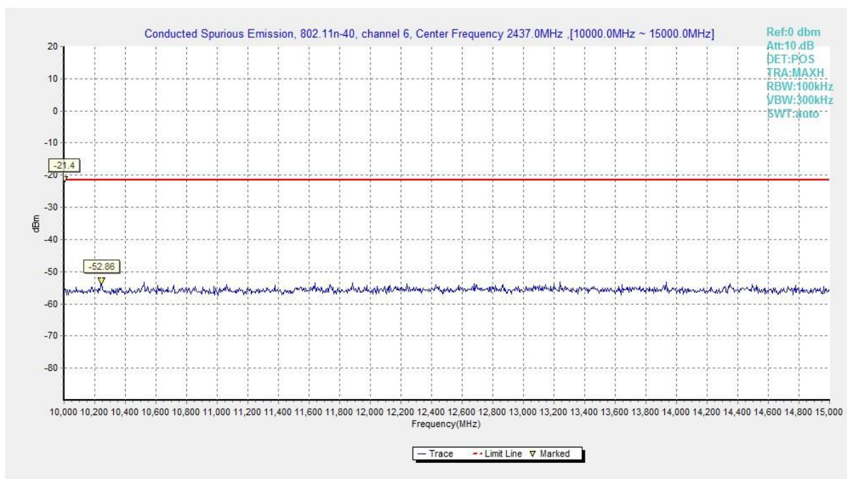
Fig.A.6.1.85 Transmitter Spurious Emission - Conducted (802.11n-HT40, Ch6, 10 GHz-15 GHz)
