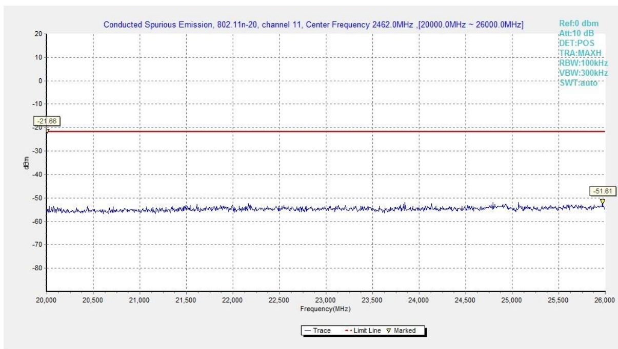
Fig.A.6.1.71 Transmitter Spurious Emission - Conducted (802.11n-HT20, Ch11, 20 GHz-26 GHz)
