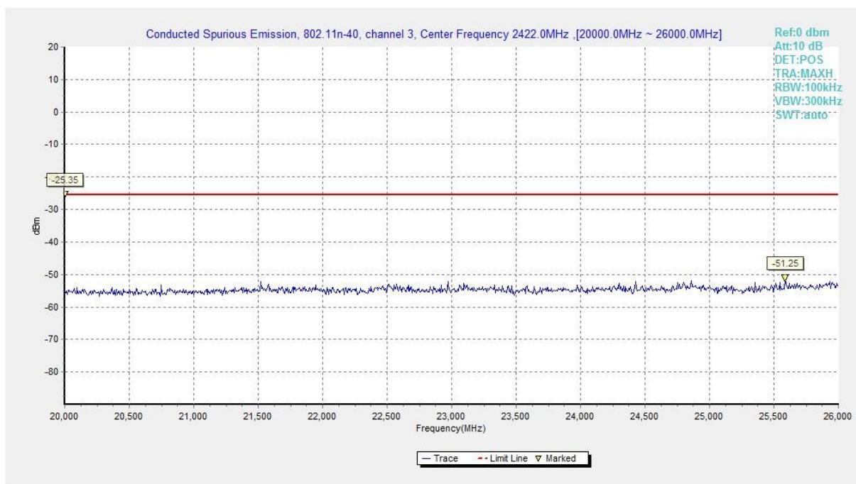
Fig.A.6.1.79 Transmitter Spurious Emission - Conducted (802.11n-HT40, Ch3, 20 GHz-26 GHz)
