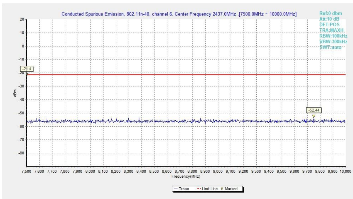
Fig.A.6.1.84 Transmitter Spurious Emission - Conducted (802.11n-HT40, Ch6, 7.5 GHz-10 GHz)
