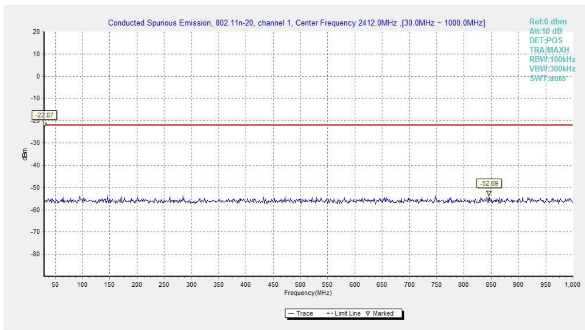
Fig.A.6.1.49 Transmitter Spurious Emission - Conducted (802.11n-HT20, Ch1, 30 MHz-1 GHz)
