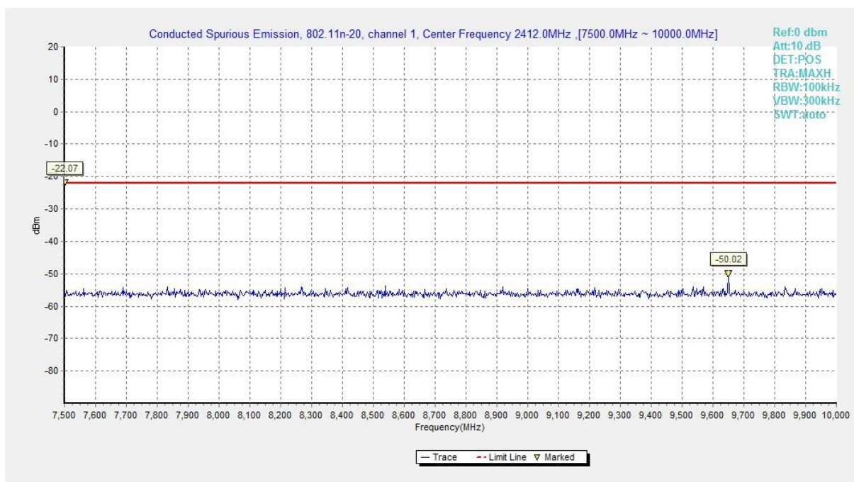
Fig.A.6.1.52 Transmitter Spurious Emission - Conducted (802.11n-HT20, Ch1, 7.5 GHz-10 GHz)
