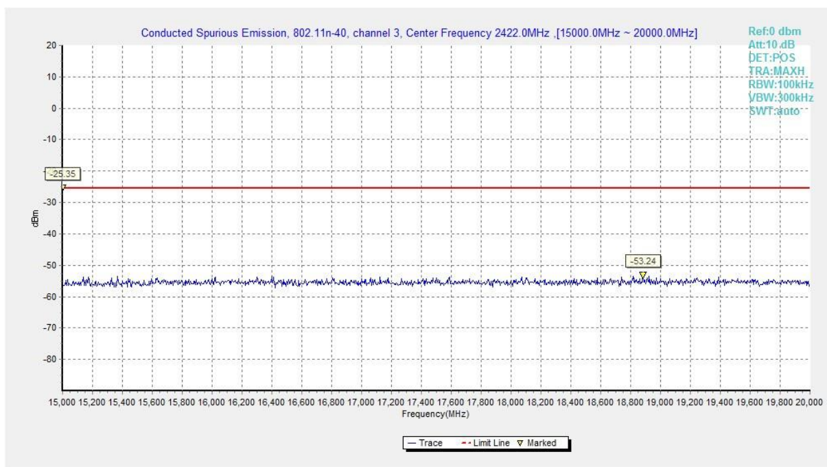
Fig.A.6.1.78 Transmitter Spurious Emission - Conducted (802.11n-HT40, Ch3, 15 GHz-20 GHz)
