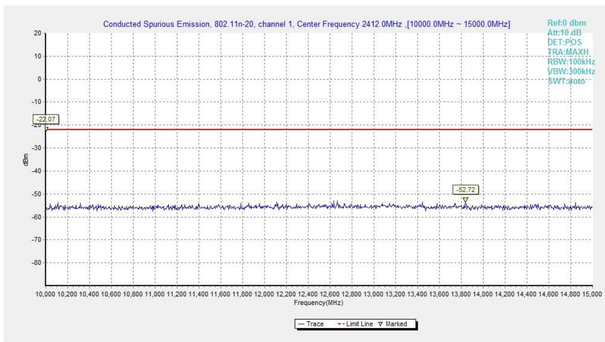
Fig.A.6.1.53 Transmitter Spurious Emission - Conducted (802.11n-HT20, Ch1, 10 GHz-15 GHz)
