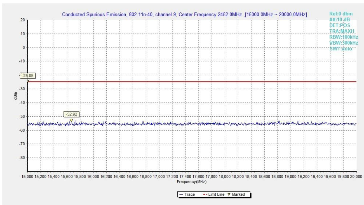
Fig.A.6.1.94 Transmitter Spurious Emission - Conducted (802.11n-HT40, Ch9, 15 GHz-20 GHz)
