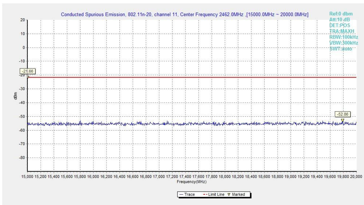
Fig.A.6.1.70 Transmitter Spurious Emission - Conducted (802.11n-HT20, Ch11, 15 GHz-20 GHz)
