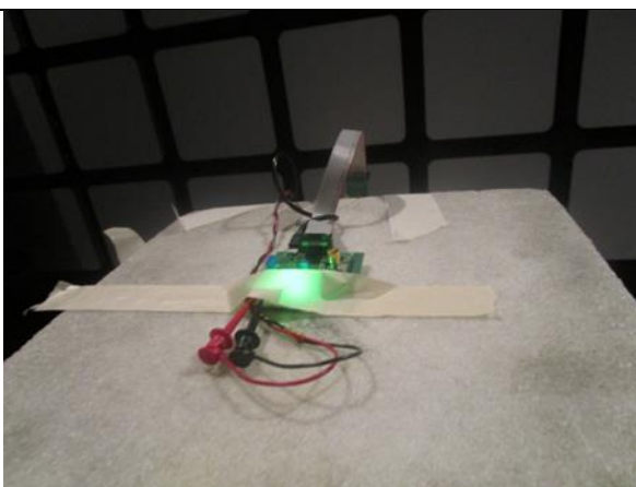
Flat Orientation
