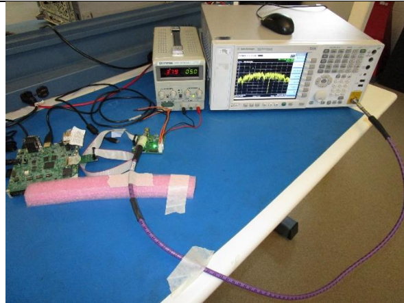
Conducted Emissions
