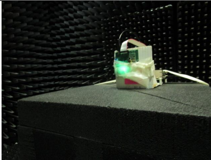
Radiated Emissions
