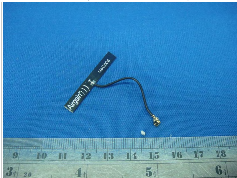
Antenna 2 (P/N: N2420GS-PK1-B40UR2)
