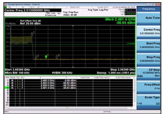
Conducted Emission: 8DPSK, 2480,2DH5 ,Band Edge
