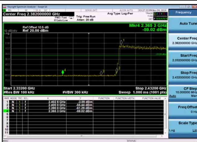
Conducted Emission: 8DPSK,2402,2DH5 ,Band Edge
