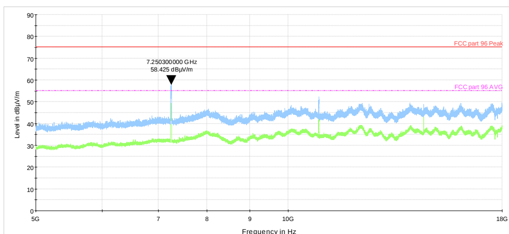
Plot 7.5.12 Radiated emission measurements in 5000 – 18000 MHz range
