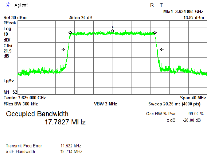
Plot 7.3.15 Occupied bandwidth test result at mid frequency
