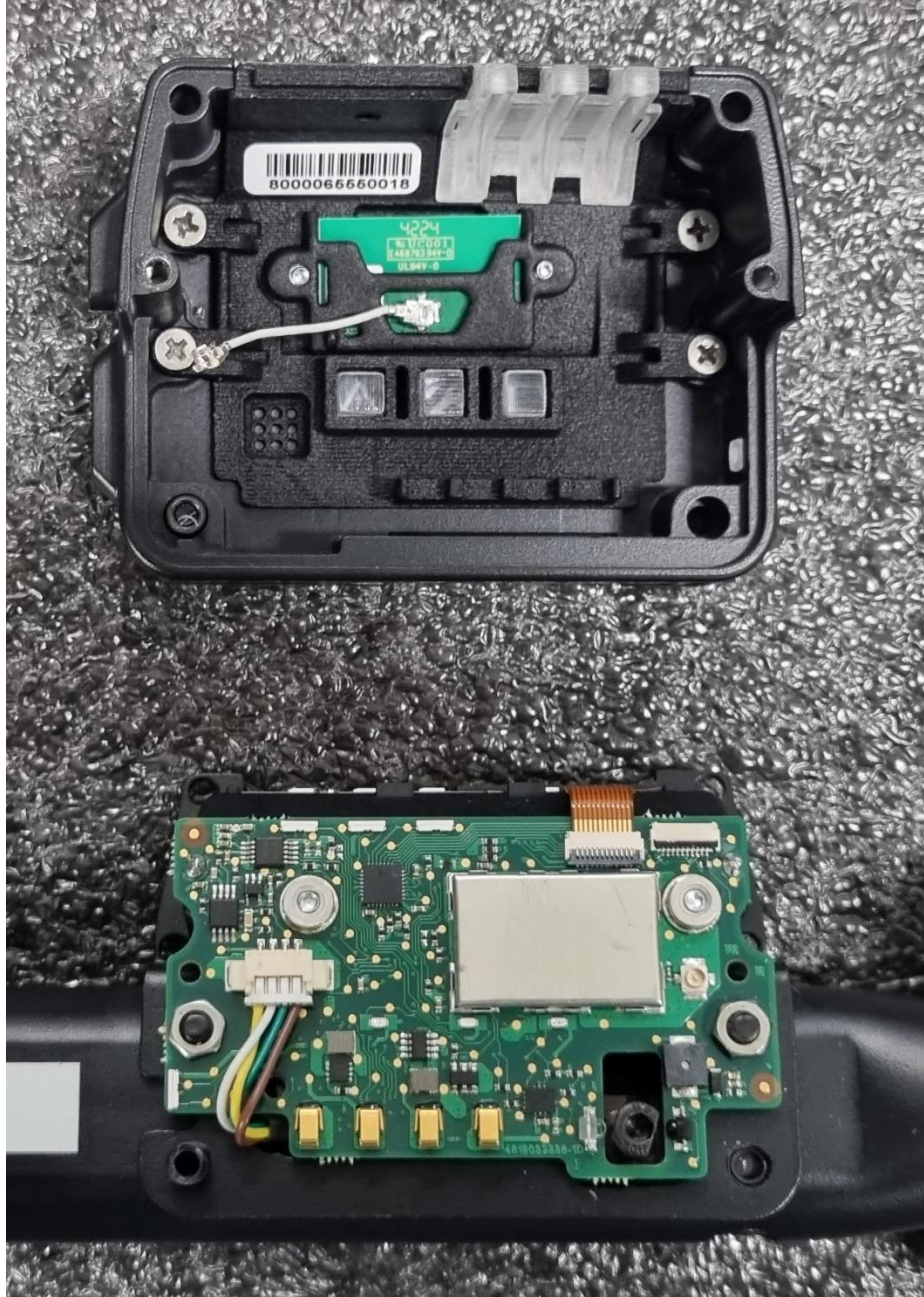
MTRwrench Electronic Housing Opened
