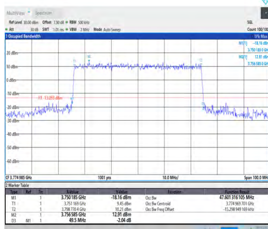
1-N78-3700-3800-30-50-H-6-CP-QPSK-Outer_Full-1 33@0-Ant1-47.601-49.500-≤50-PASS
