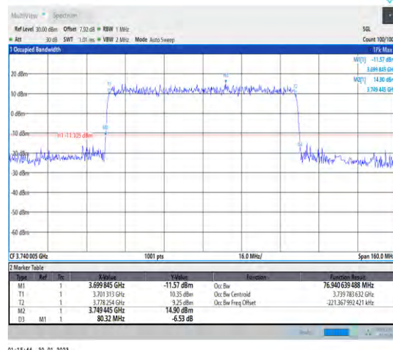
1-N78-3700-3800-30-80-L-4-DFT-64QAM-Outer_Full -216@0-Ant1-76.941-80.320-≤80-PASS
