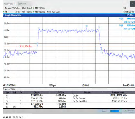
1-N78-3700-3800-30-20-L-8-CP-64QAM-Outer_Full-51@0-Ant1-18.278-19.320-≤20-PASS
