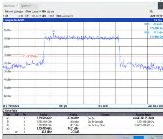
1-N78-3700-3800-30-50-H-3-DFT-16QAM-Outer_Ful I-128@0-Ant1-45.65-47.500-≤50-PASS
