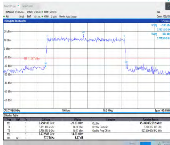
1-N78-3700-3800-30-50-H-4-DFT-64QAM-Outer_Ful I-128@0-Ant1-45.786-47.700-≤50-PASS
