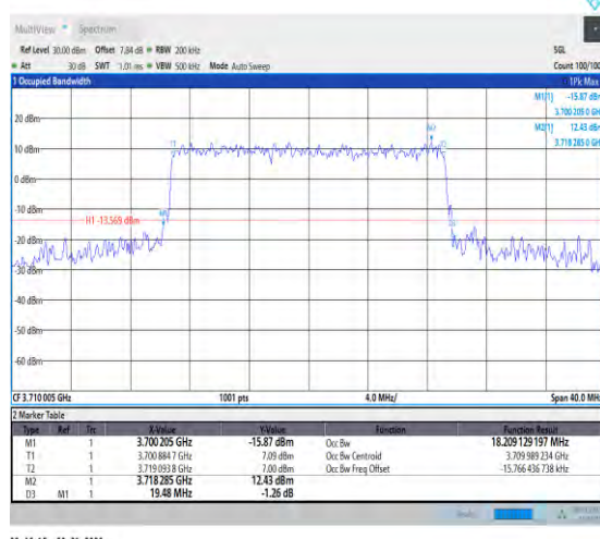
1-N78-3700-3800-30-20-L-6-CP-QPSK-Outer_Full-5 1@0-Ant1-18.209-19.480-≤20-PASS
