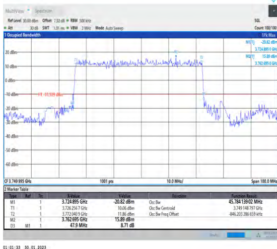
1-N78-3700-3800-30-50-M-2-DFT-P12BPSK-Outer_Ful Full-128@0-Ant1-45.784-47.900-≤50-PASS
