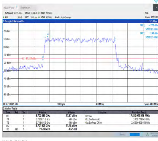
1-N78-3700-3800-30-20-L-5-DFT-256QAM-Outer_F ull-50@0-Ant1-17.813-19.280-≤20-PASS
