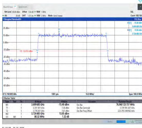
1-N78-3700-3800-30-80-L-5-DFT-256QAM-Outer_F ull-216@0-Ant1-76.96-80.320-≤80-PASS
