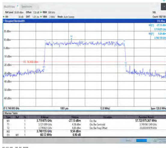
1-N78-3700-3800-30-60-M-9-CP-256QAM-Outer_Fu II-162@0-Ant1-57.724-60.120-≤60-PASS
