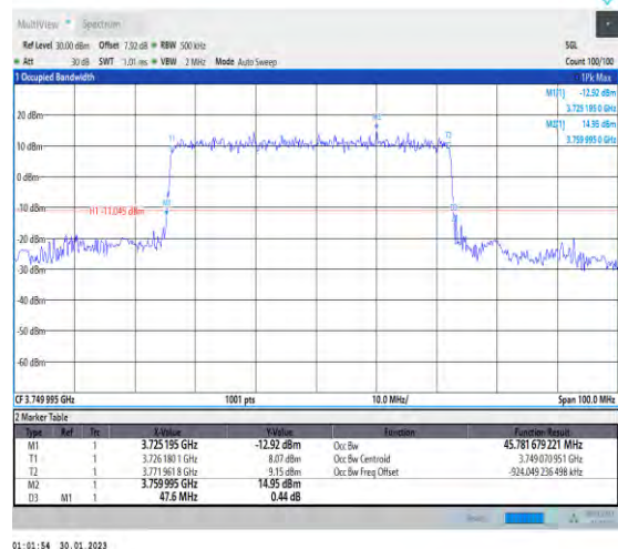
1-N78-3700-3800-30-50-M-3-DFT-16QAM-Outer_Ful I-128@0-Ant1-45.782-47.600-≤50-PASS
