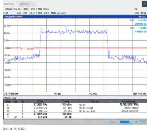
1-N78-3700-3800-30-50-M-1-DFT-QPSK-Outer_Full- 128@0-Ant1-45.782-47.700-≤50-PASS
