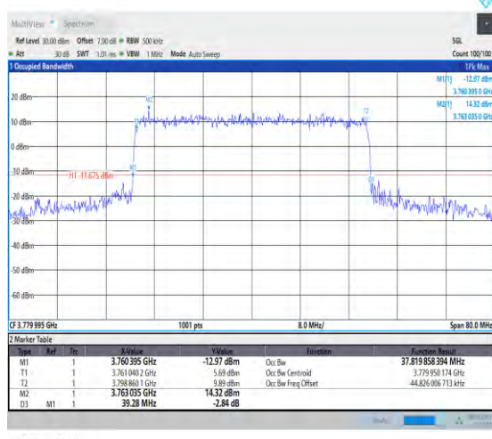
1-N78-3700-3800-30-40-H-8-CP-64QAM-Outer_Full-106@0-Ant1-37.82-39.280-≤40-PASS
