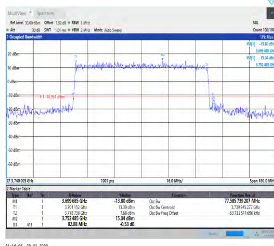
1-N78-3700-3800-30-80-L-6-CP-QPSK-Outer_Full-2 17@0-Ant1-77.586-82.880-≤80-PASS
