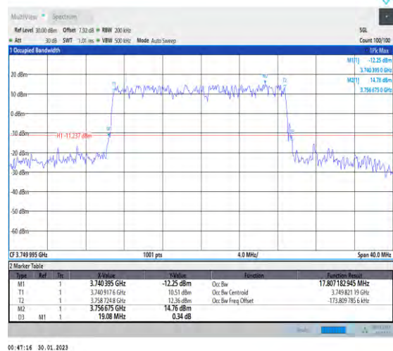
1-N78-3700-3800-30-20-M-1-DFT-QPSK-Outer_Full-50@0-Ant1-17.807-19.080-≤20-PASS
