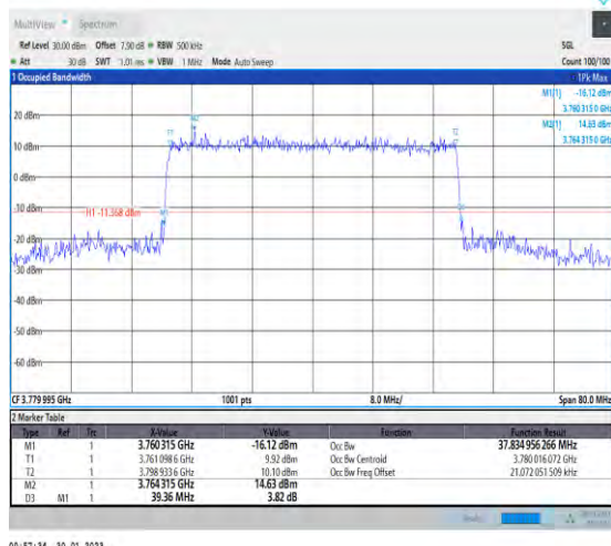
1-N78-3700-3800-30-40-H-6-CP-QPSK-Outer_Full-106@0-Ant1-37.835-39.360-≤40-PASS
