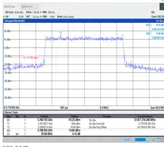
1-N78-3700-3800-30-40-H-7-CP-16QAM-Outer_Full-106@0-Ant1-37.811-39.680-≤40-PASS
