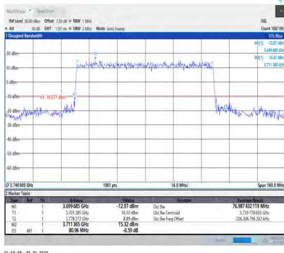
1-N78-3700-3800-30-80-L-3-DFT-16QAM-Outer_Full -216@0-Ant1-76.987-80.960-≤80-PASS
