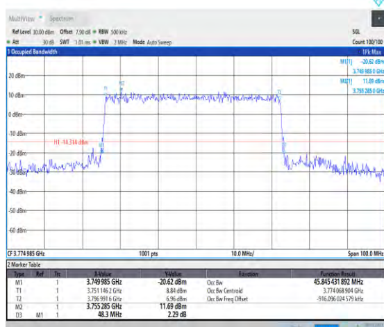
1-N78-3700-3800-30-50-H-5-DFT-256QAM-Outer_F ull-128@0-Ant1-45.845-48.300-≤50-PASS
