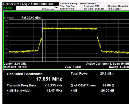
Channel: MIDDLE, Modulation: 16QAM, BW=20MHz
