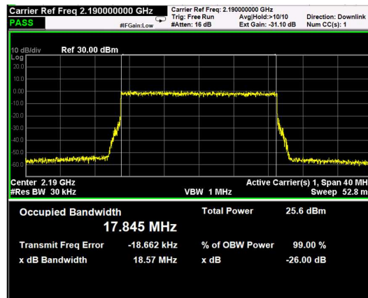
Channel: MIDDLE, Modulation: 256QAM, BW=20MHz
