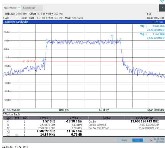
1-N38--30-15-L-8-CP-64QAM-Outer_Full-38@0- Ant1-13.606-14.970≤15-PASS
