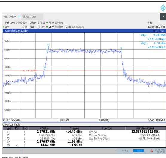
1-N38--30-15-L-6-CP-QPSK-Outer_Full-38@0-Ant1- 13.588-14.670-≤15-PASS
