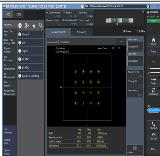
1-N38--30-40-M-7-CP-16QAM-Outer_Full-106@0-Ant1-see graph-PASS
