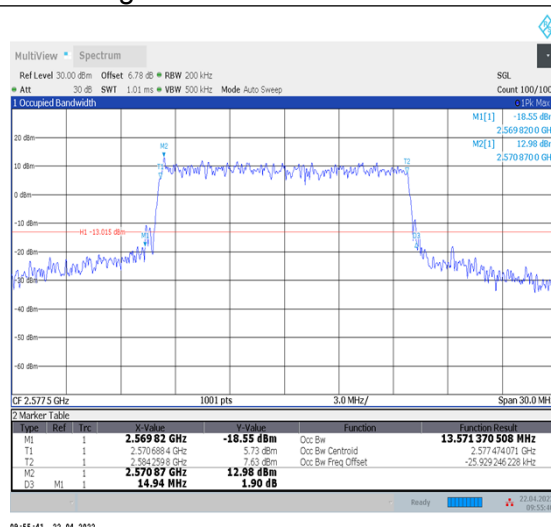
1-N38--30-15-L-7-CP-16QAM-Outer_Full-38@0- Ant1-13.571-14.940≤15-PASS
