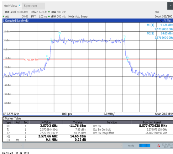
1-N38--30-10-L-1-DFT-QPSK-Outer_Full-24@0- Ant1-8.577-9.400-≤10-PASS
