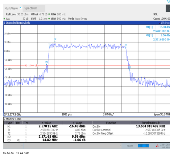
1-N38--30-15-L-9-CP-256QAM-Outer_Full-38@0- Ant1-13.604-14.820-≤15-PASS
