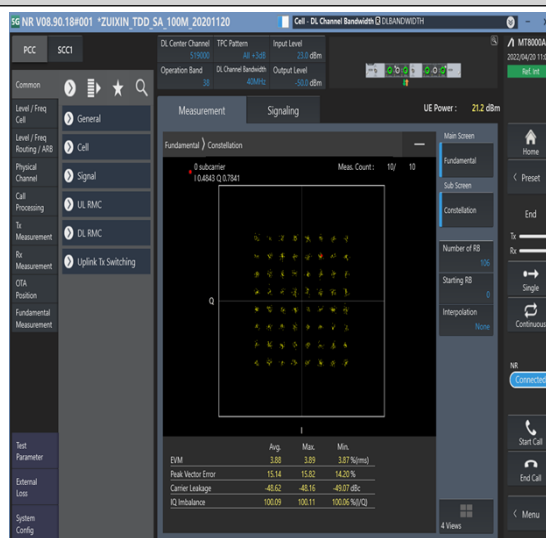
1-N38--30-40-M-8-CP-64QAM-Outer_Full-106@0-Ant1-see graph-PASS
