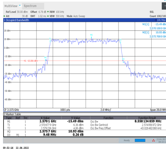
1-N38--30-10-L-4-DFT-64QAM-Outer_Full-24@0- Ant1-8.558-9.480-≤10-PASS
