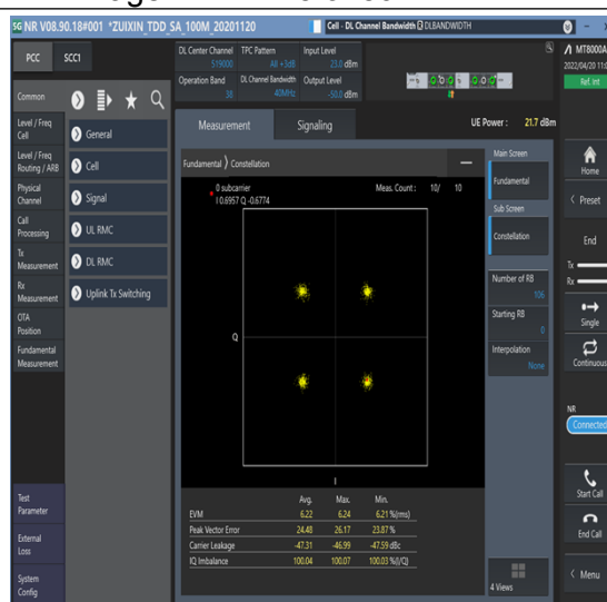
1-N38--30-40-M-6-CP-QPSK-Outer_Full-106@0-Ant1-see graph-PASS
