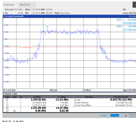
1-N38--30-10-L-2-DFT-PI2BPSK-Outer_Full-24@0- Ant1-8.544-9.360-≤10-PASS
