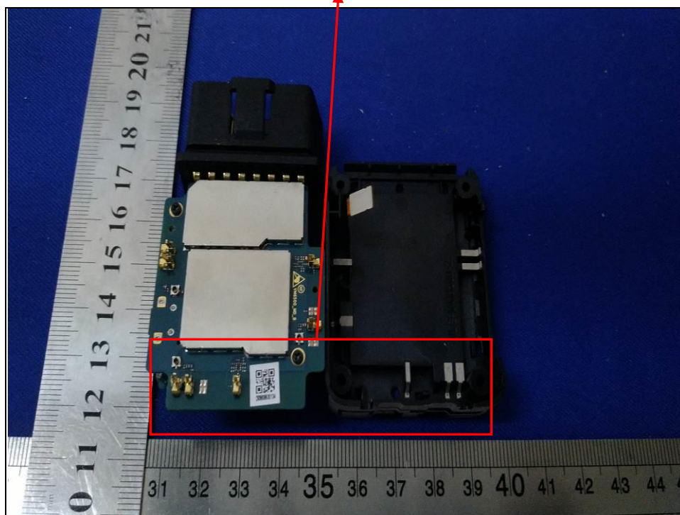
Diversity Antenna
