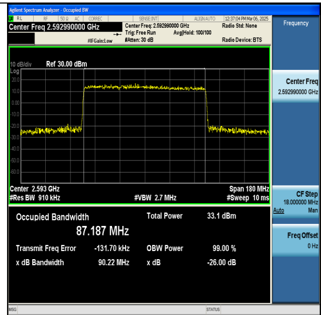
NTNV-n41-PC2-30-90-M-CP-QPSK-Outer_Full-Ant1-PASS
