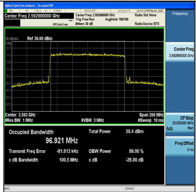
NTNV-n41-PC2-30-100-M-CP-256QAM-Outer_Full-Ant1- PASS
