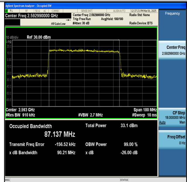
NTNV-n41-PC2-30-90-M-CP-64QAM-Outer_Full-Ant1-PASS
