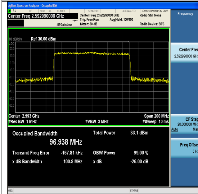
NTNV-n41-PC2-30-100-M-CP-64QAM-Outer_Full-Ant1- PASS
