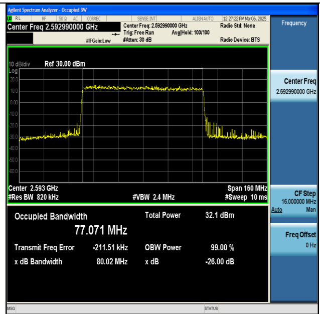
NTNV-n41-PC2-30-80-M-DFT-256QAM-Outer_Full-Ant1-PASS
