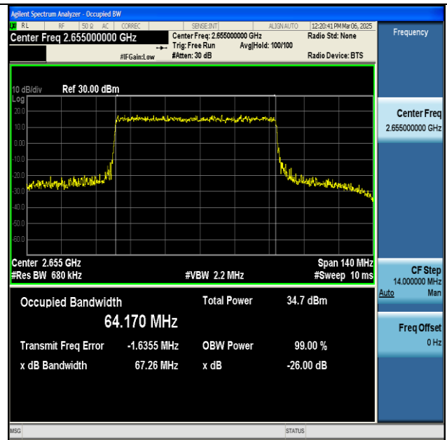
NTNV-n41-PC2-30-70-H-DFT-16QAM-Outer_Full-Ant1-1 PASS
