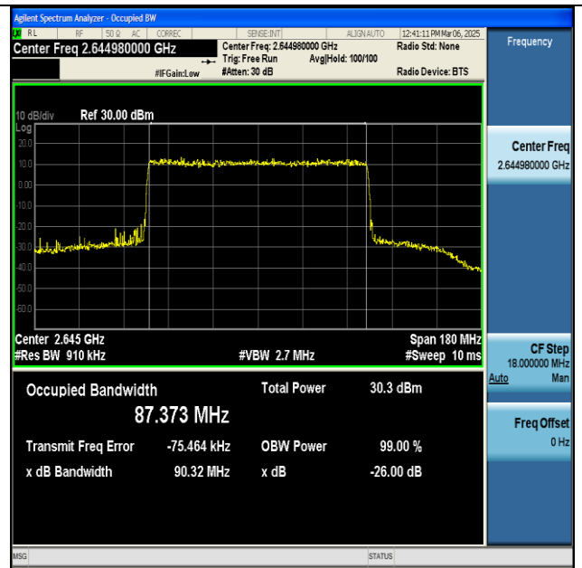
NTNV-n41-PC2-30-90-H-CP-256QAM-Outer_Full-Ant1- PASS
