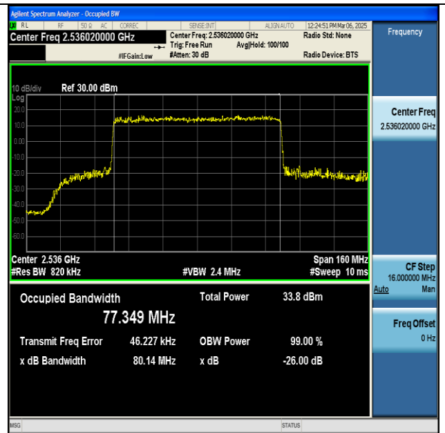
NTNV-n41-PC2-30-80-L-CP-QPSK-Outer_Full-Ant1-PASS
