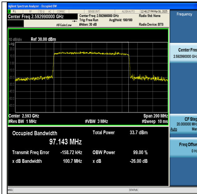
NTNV-n41-PC2-30-100-M-CP-QPSK-Outer_Full-Ant1- PASS
