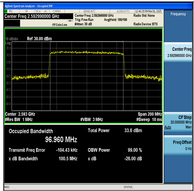
NTNV-n41-PC2-30-100-M-CP-16QAM-Outer_Full-Ant1- PASS
