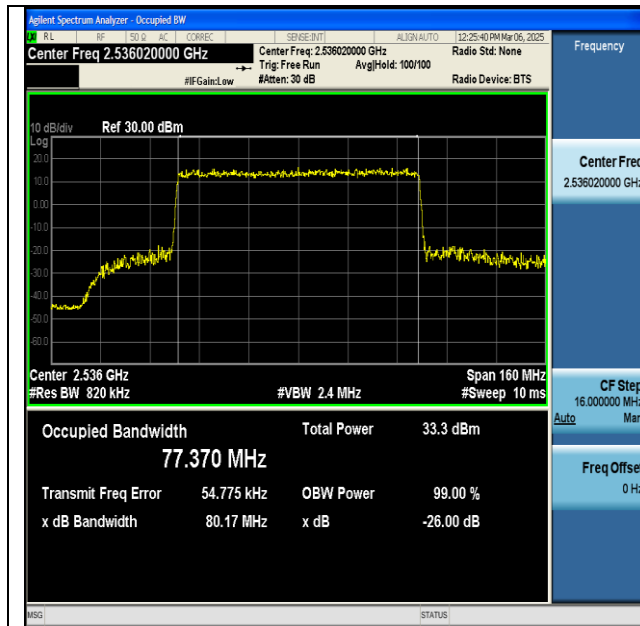
NTNV-n41-PC2-30-80-L-CP-256QAM-Outer_Full-Ant1- PASS
