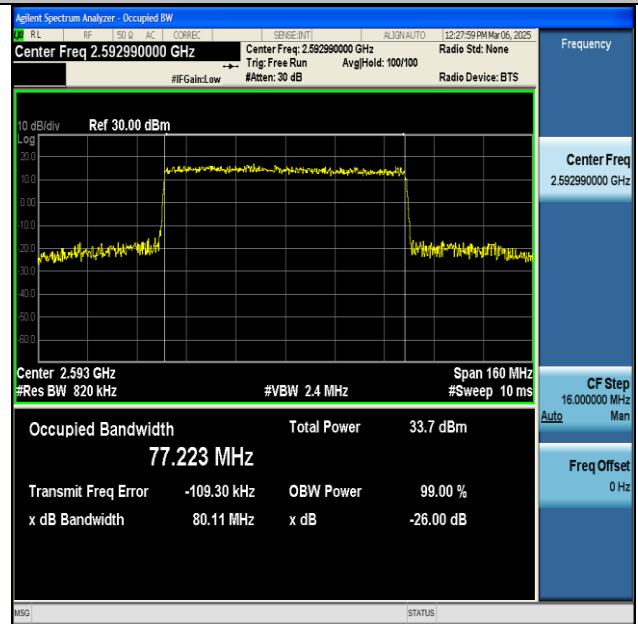
NTNV-n41-PC2-30-80-M-CP-16QAM-Outer_Full-Ant1-PASS
