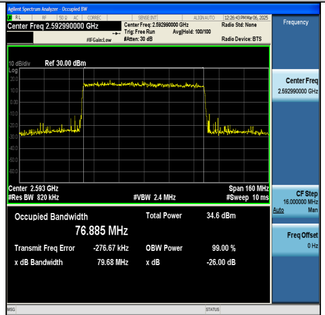
NTNV-n41-PC2-30-80-M-DFT-16QAM-Outer_Full-Ant1- PASS
