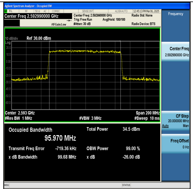
NTNV-n41-PC2-30-100-M-DFT-16QAM-Outer_Full-Ant1- PASS
