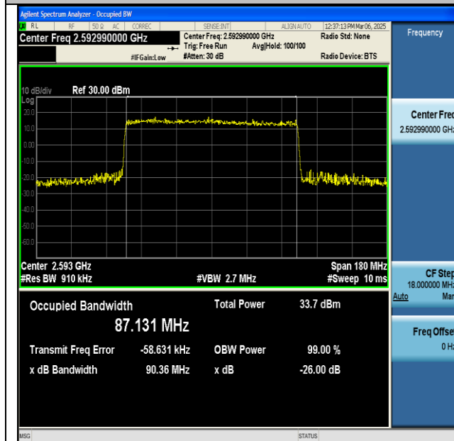
NTNV-n41-PC2-30-90-M-CP-16QAM-Outer_Full-Ant1-PASS
