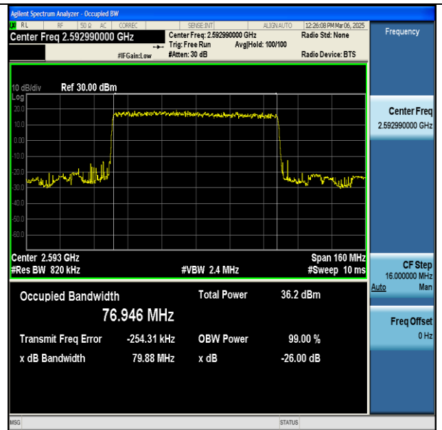
NTNV-n41-PC2-30-80-M-DFT-BPSK-Outer_Full-Ant1- PASS
