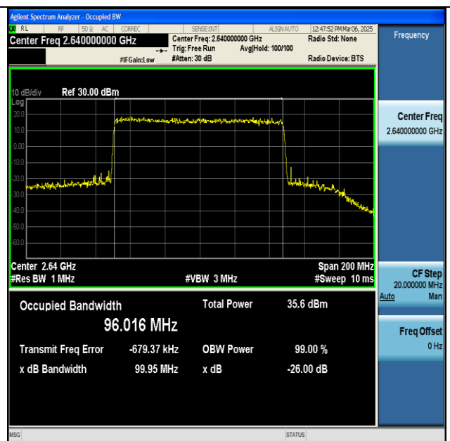
NTNV-n41-PC2-30-100-H-DFT-QPSK-Outer_Full-Ant1- PASS
