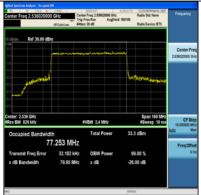
NTNV-n41-PC2-30-80-L-CP-64QAM-Outer_Full-Ant1-PASS
