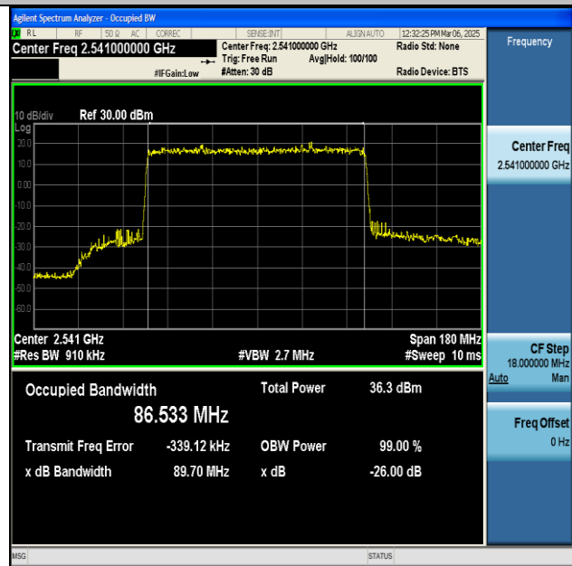
NTNV-n41-PC2-30-90-L-DFT-BPSK-Outer_Full-Ant1- PASS
