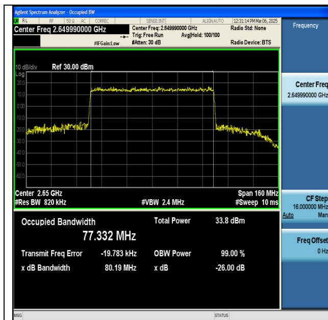
NTNV-n41-PC2-30-80-H-CP-16QAM-Outer_Full-Ant1- PASS
