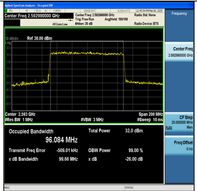
NTNV-n41-PC2-30-100-M-DFT-256QAM-Outer_Full-Ant1- PASS
