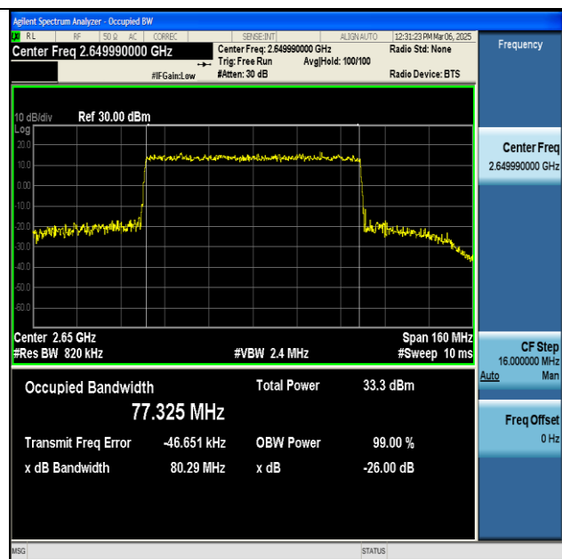
NTNV-n41-PC2-30-80-H-CP-64QAM-Outer_Full-Ant1- PASS
