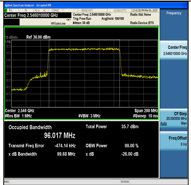
NTNV-n41-PC2-30-100-L-DFT-QPSK-Outer_Full-Ant1- PASS
