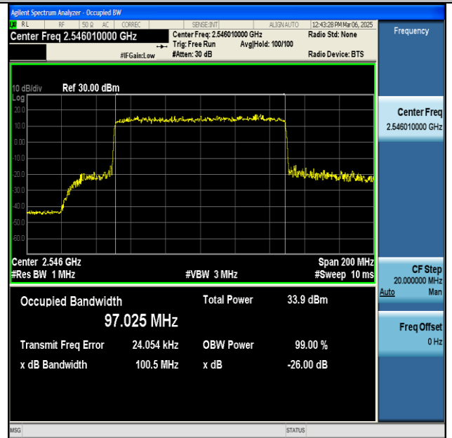
NTNV-n41-PC2-30-100-L-CP-QPSK-Outer_Full-Ant1- PASS
