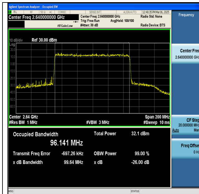
NTVN-n41-PC2-30-100-H-DFT-256QAM-Outer_Full-Ant1- PASS
