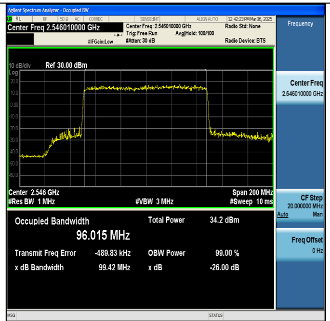
NTNV-n41-PC2-30-100-L-DFT-64QAM-Outer_Full-Ant1- PASS
