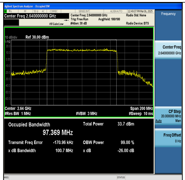
NTVN-n41-PC2-30-100-H-CP-QPSK-Outer_Full-Ant1- PASS
