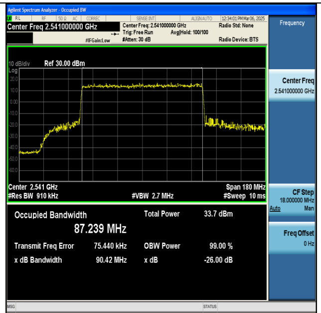
NTNV-n41-PC2-30-90-L-CP-16QAM-Outer_Full-Ant1-PASS
