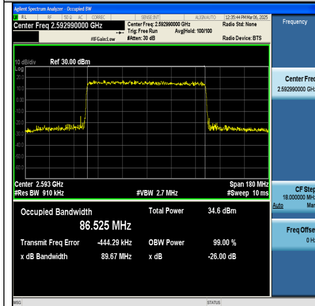
NTNV-n41-PC2-30-90-M-DFT-16QAM-Outer_Full-Ant1- PASS
