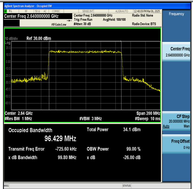
NTNV-n41-PC2-30-100-H-DFT-64QAM-Outer_Full-Ant1- PASS
