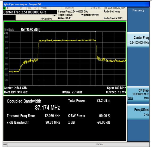
NTNV-n41-PC2-30-90-L-CP-256QAM-Outer_Full-Ant1-PASS
