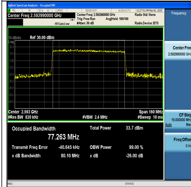
NTNV-n41-PC2-30-80-M-CP-QPSK-Outer_Full-Ant1-PASS
