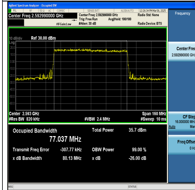
NTNV-n41-PC2-30-80-M-DFT-QPSK-Outer_Full-Ant1- PASS
