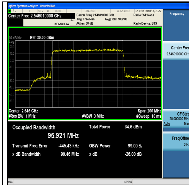
NTNV-n41-PC2-30-100-L-DFT-16QAM-Outer_Full-Ant1- PASS
