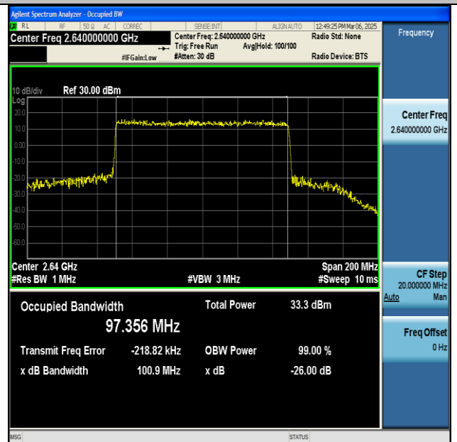
NTVN-n41-PC2-30-100-H-CP-64QAM-Outer_Full-Ant1- PASS
