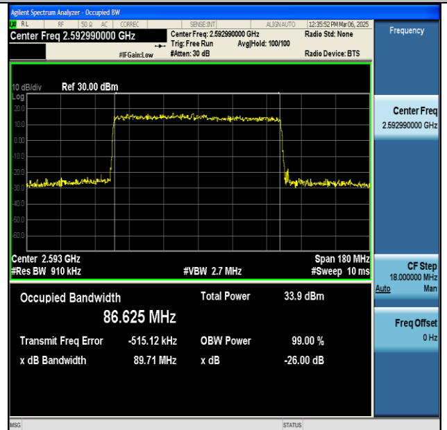
NTNV-n41-PC2-30-90-M-DFT-64QAM-Outer_Full-Ant1- PASS
