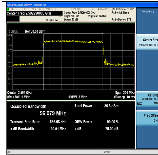
NTNV-n41-PC2-30-100-M-DFT-QPSK-Outer_Full-Ant1- PASS
