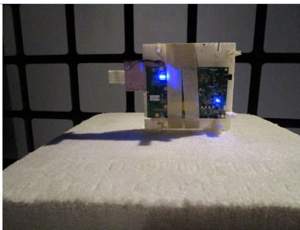
Horizontal/Side Orientation
