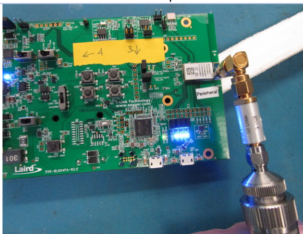
Conducted Measurements
