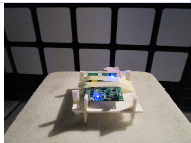
Flat Orientation
