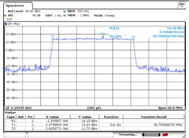
30 MHz DFT-S-OFDM QPSK
