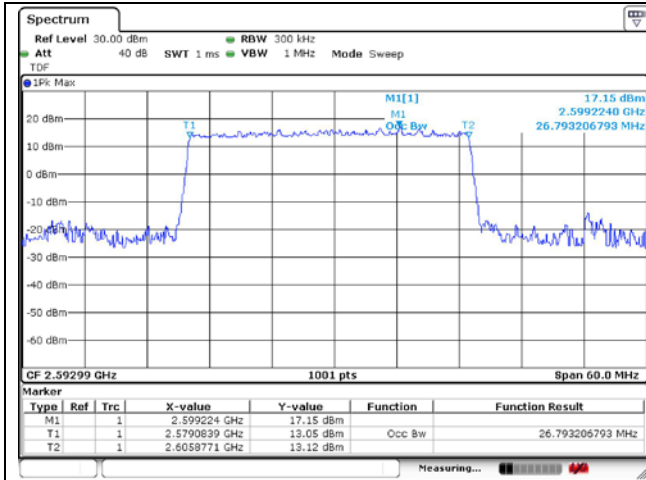
30 MHz DFT-S-OFDM BPSK
