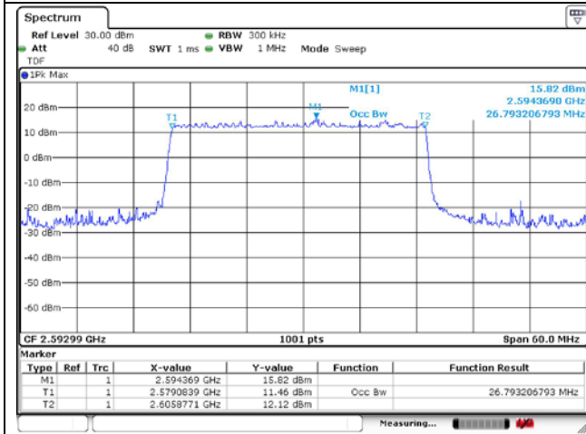
30 MHz DFT-S-OFDM 16QAM
