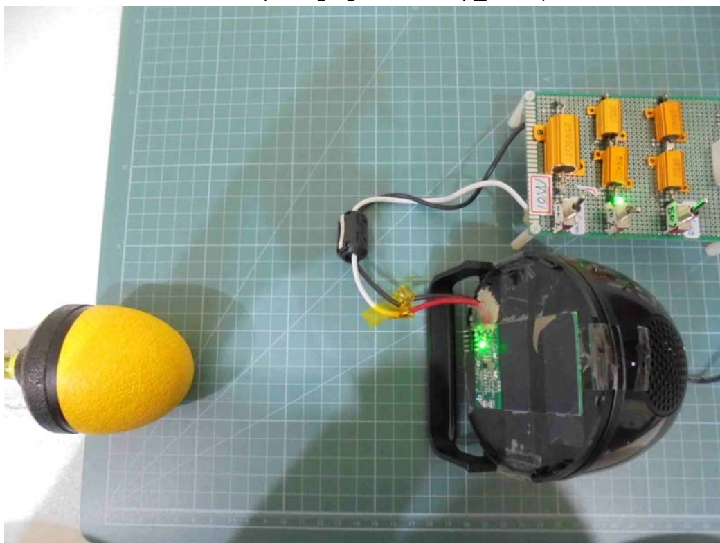
E-Field (Charging Mode - Top_20cm)
