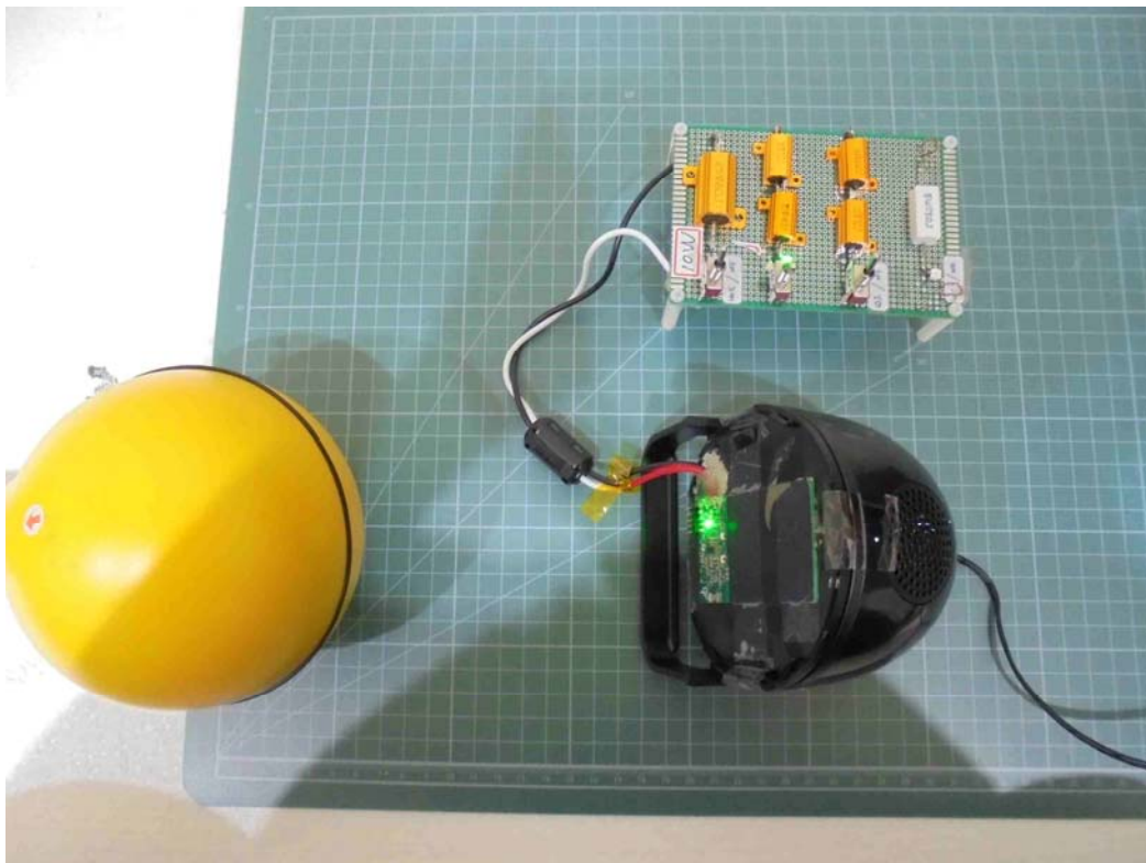
H-Field (Charging Mode - Top_20cm)
