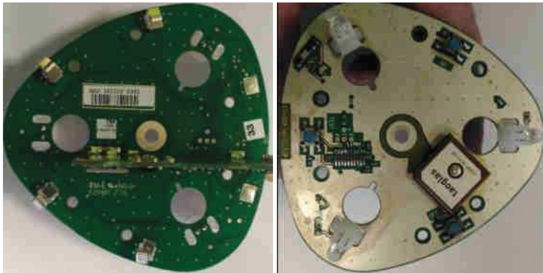
Figure 13 – McMurdo and Kannad Internal photo3
