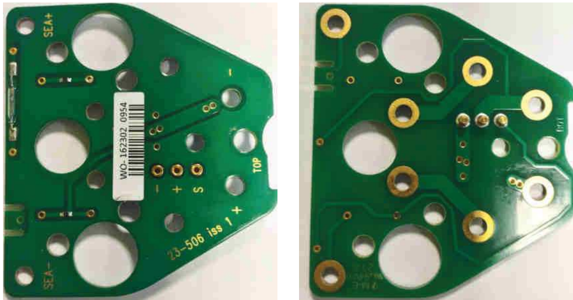
Figure 15 - McMurdo and Kannad Internal photo5
