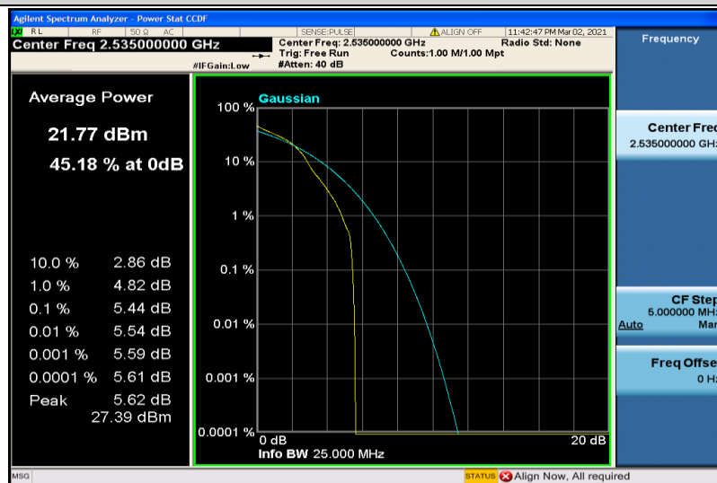
Band7-20MHz-16QAM-21100-1RB#0
