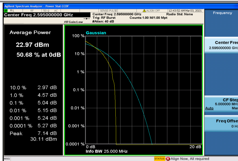
Band38-15MHz-QPSK-38000-1RB#0
