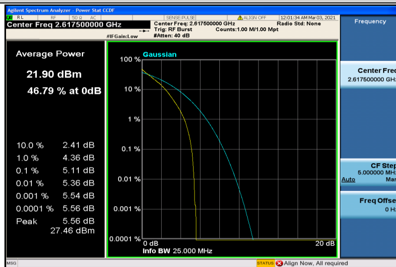
Band38-5MHz-QPSK-38225-25RB#0
