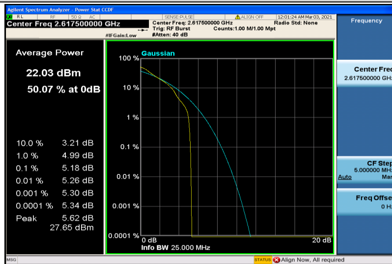
Band38-5MHz-QPSK-38225-1RB#0
