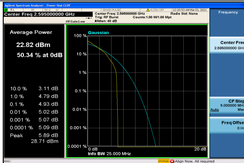
Band38-10MHz-QPSK-38000-1RB#0
