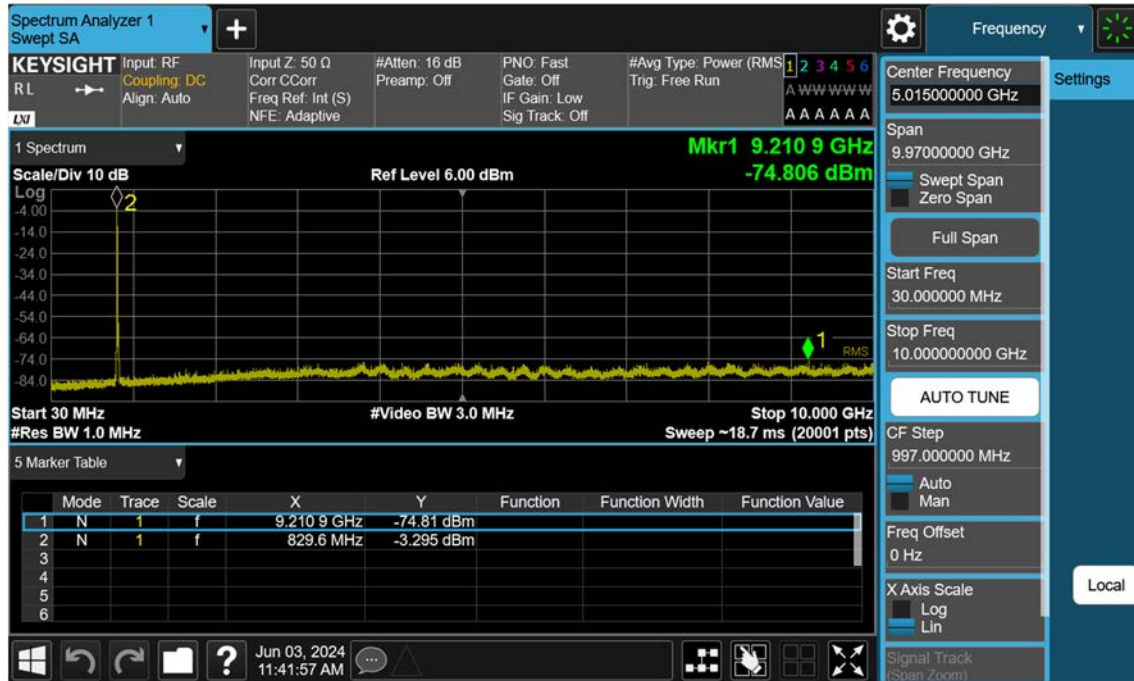
Sub6 n5_15 M_Conducted Spurious(30 M-10 G)_Mid_BPSK_1RB
