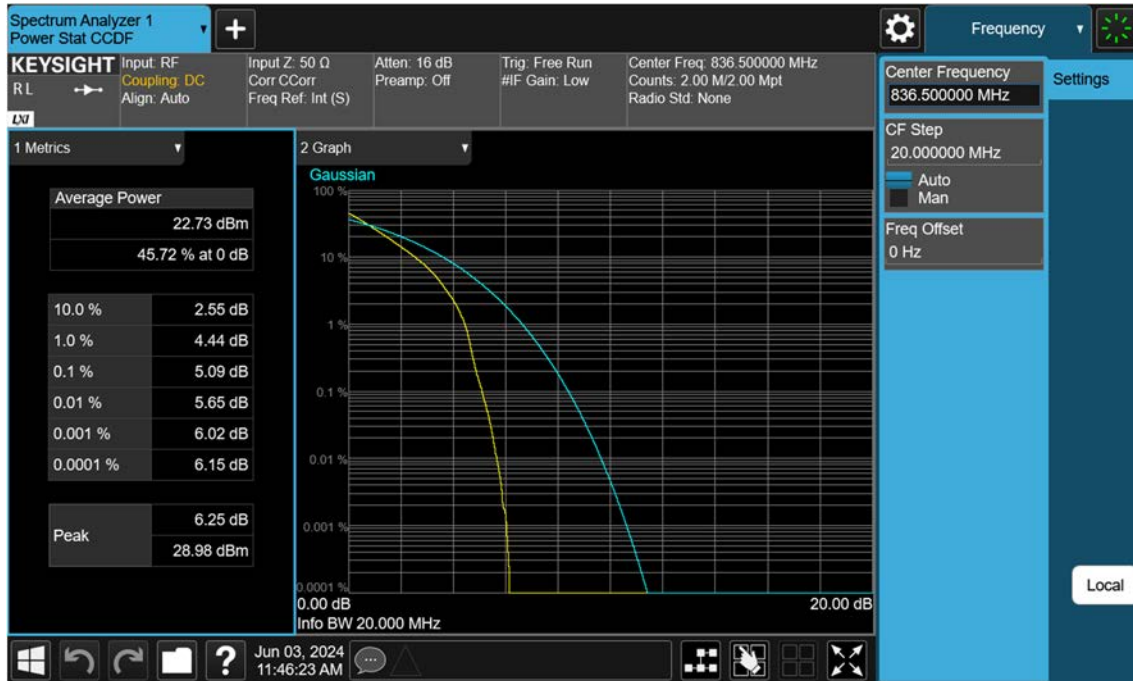
Sub6 n5_20 M_PAR_Mid_QPSK_FullRB
