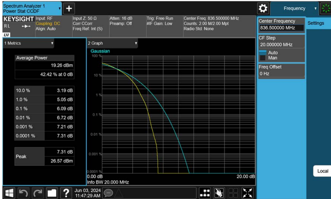
Sub6 n5_20 M_PAR_Mid_256QAM_FullRB
