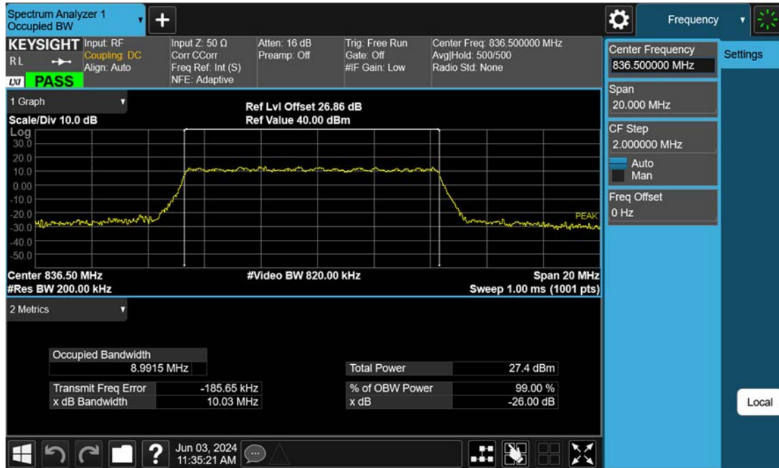
Sub6 n5_10 M_OBW_Mid_256QAM_FullRB
