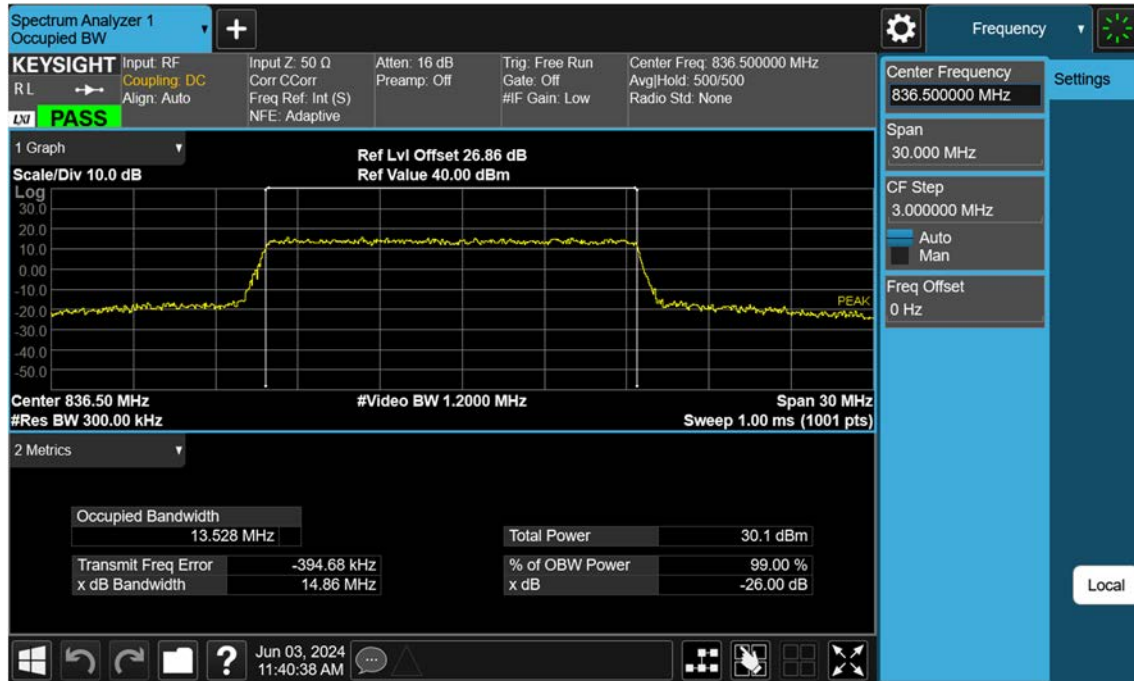
Sub6 n5_15 M_OBW_Mid_16QAM_FullRB
