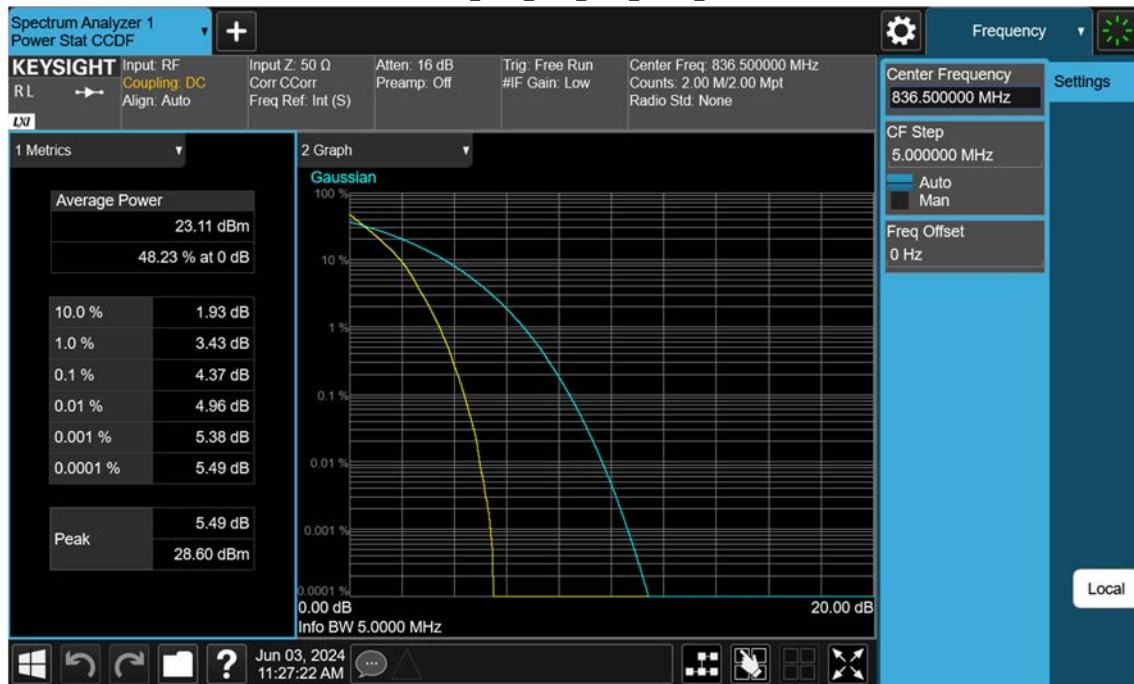
Sub6 n5_5 M_PAR_Mid_BPSK_FullRB
