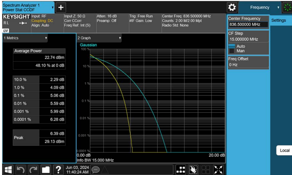
Sub6 n5_15 M_PAR_Mid_QPSK_FullRB
