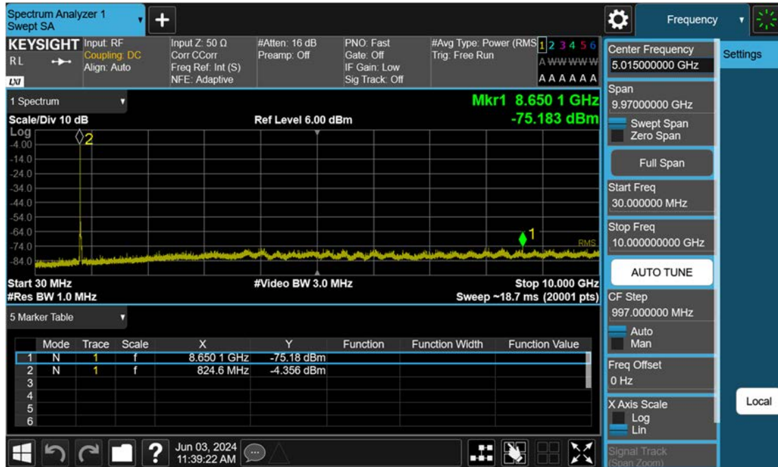
Sub6 n5_15 M_Conducted Spurious(30 M-10 G)_Low_BPSK_1RB
