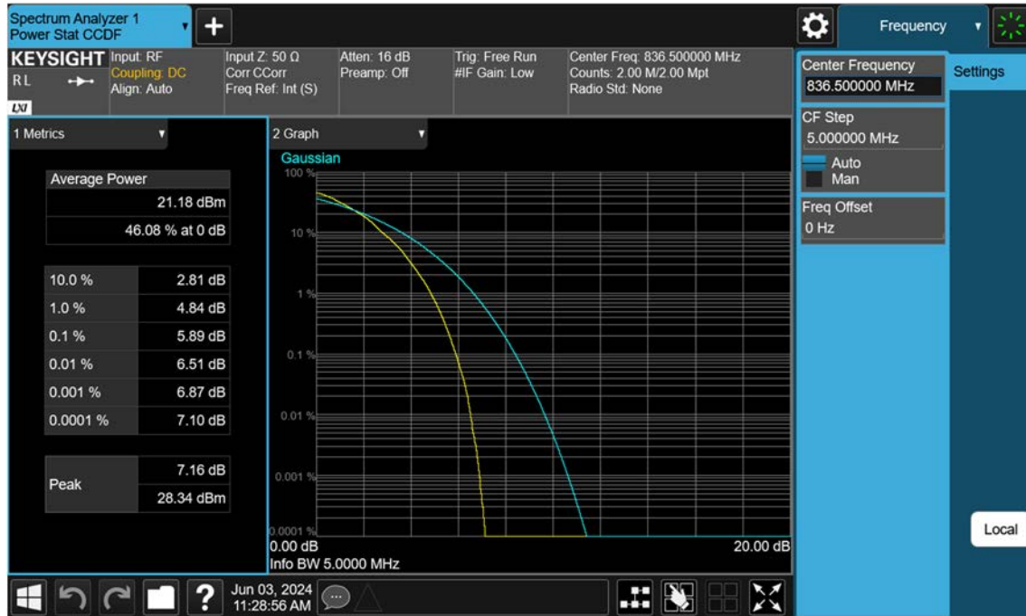
Sub6 n5_5 M_PAR_Mid_64QAM_FullRB
