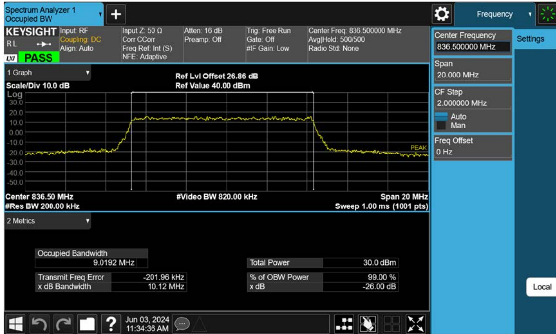
Sub6 n5_10 M_OBW_Mid_16QAM_FullRB
