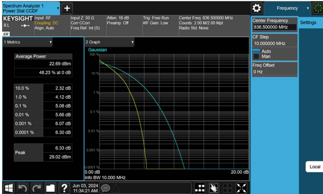
Sub6 n5_10 M_PAR_Mid_QPSK_FullRB
