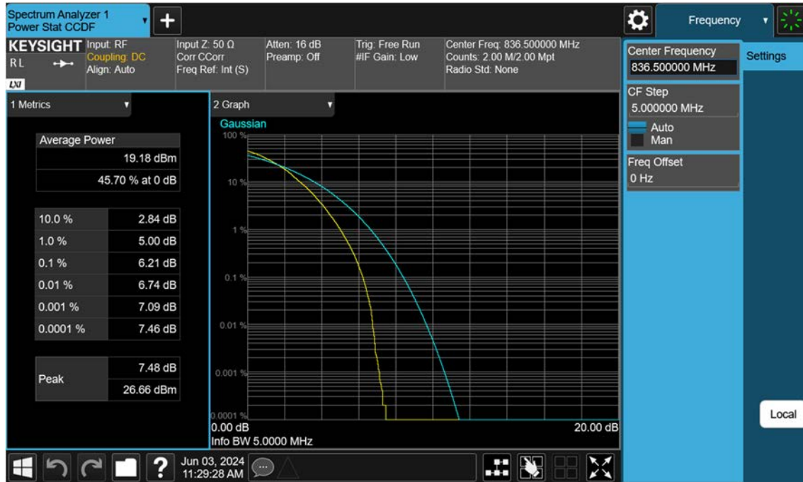
Sub6 n5_5 M_PAR_Mid_256QAM_FullRB
