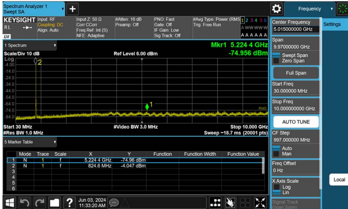
Sub6 n5_10 M_Conducted Spurious(30 M-10 G)_Low_BPSK_1RB
