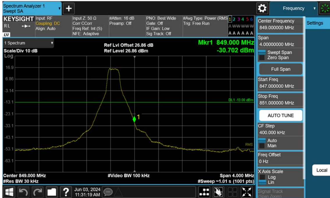
Sub6 n5_5 M_Band Edge_High_BPSK_1RB
