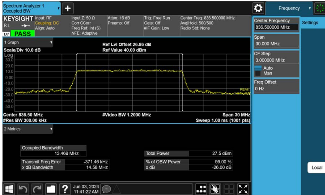
Sub6 n5_15 M_OBW_Mid_256QAM_FullRB
