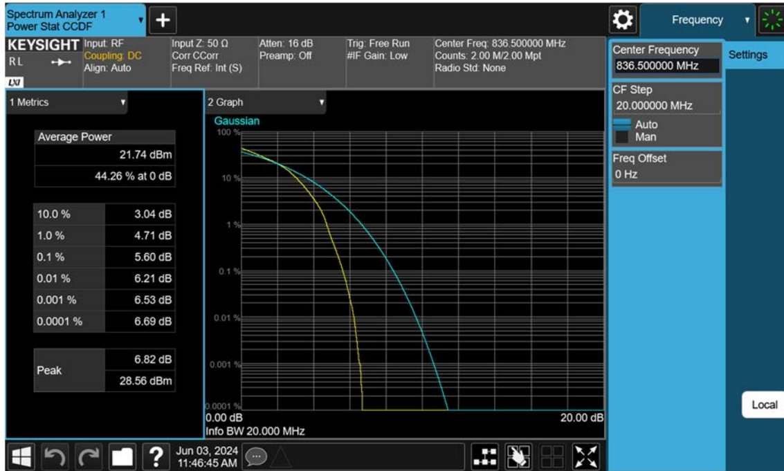
Sub6 n5_20 M_PAR_Mid_16QAM_FullRB
