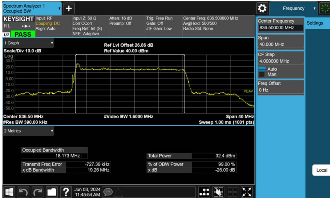
Sub6 n5_20 M_OBW_Mid_BPSK_FullRB
