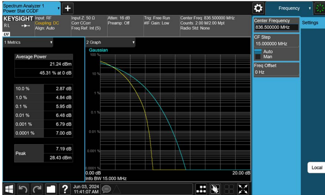
Sub6 n5_15 M_PAR_Mid_64QAM_FullRB
