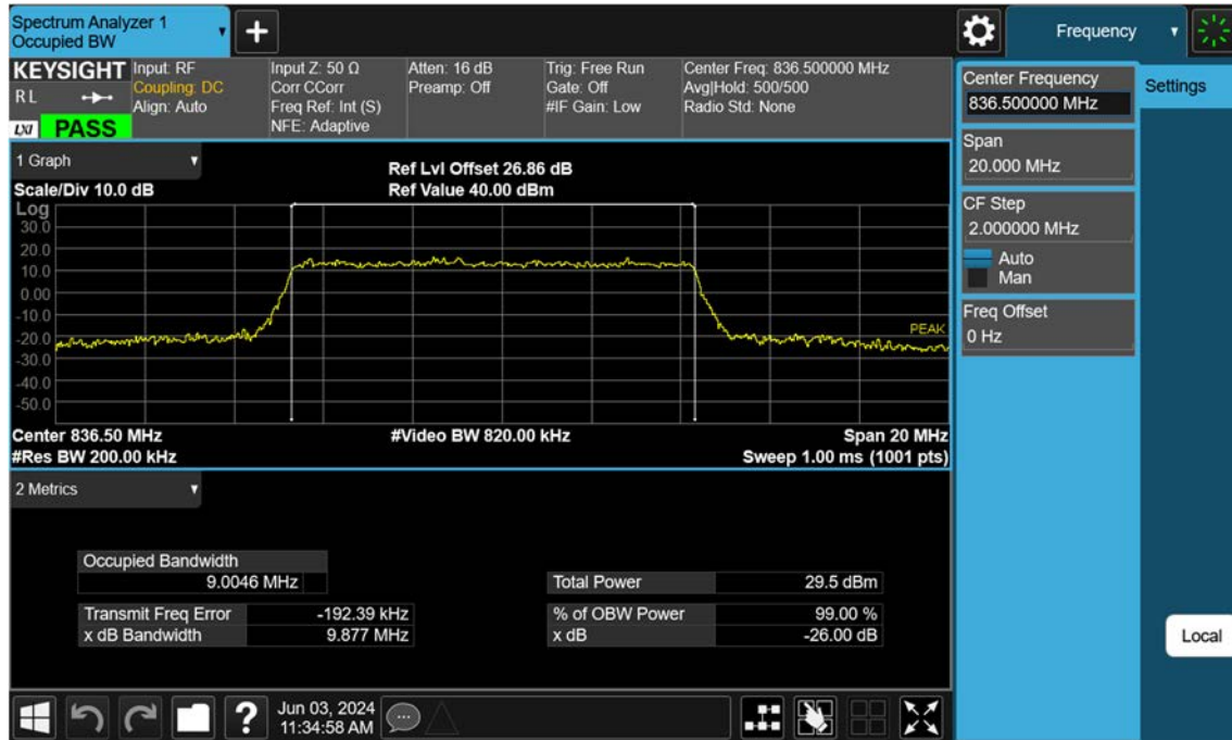
Sub6 n5_10 M_OBW_Mid_64QAM_FullRB
