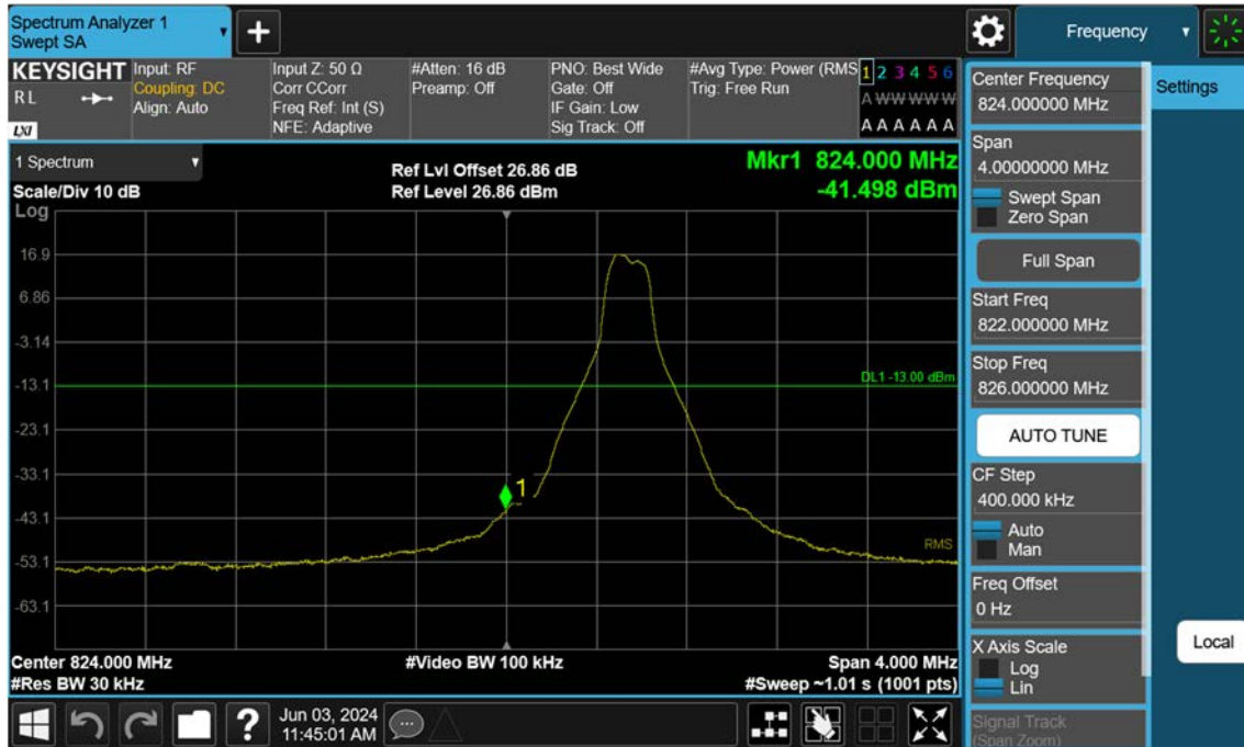
Sub6 n5_20 M_Band Edge_Low_BPSK_1RB
