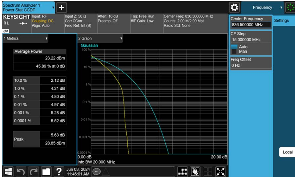
Sub6 n5_20 M_PAR_Mid_BPSK_FullRB
