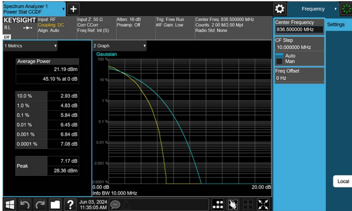
Sub6 n5_10 M_PAR_Mid_64QAM_FullRB
