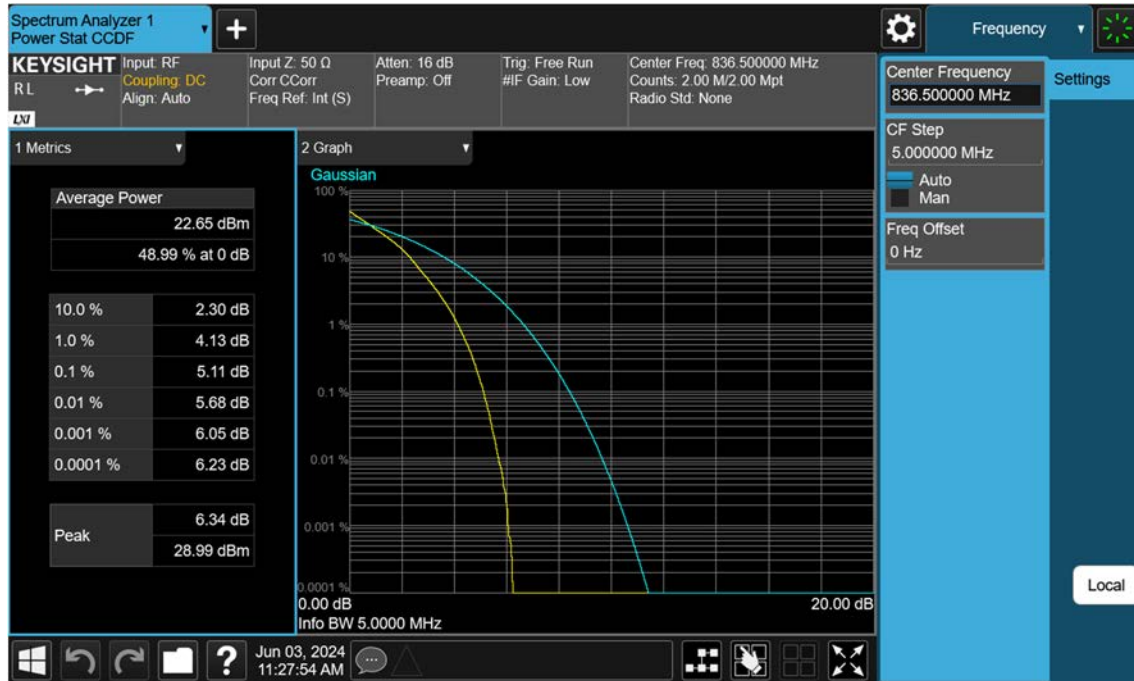
Sub6 n5_5 M_PAR_Mid_QPSK_FullRB
