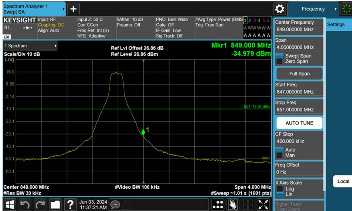
Sub6 n5_10 M_Band Edge_High_BPSK_1RB
