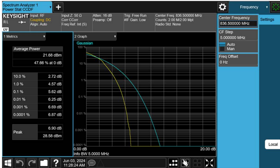
Sub6 n5_5 M_PAR_Mid_16QAM_FullRB
