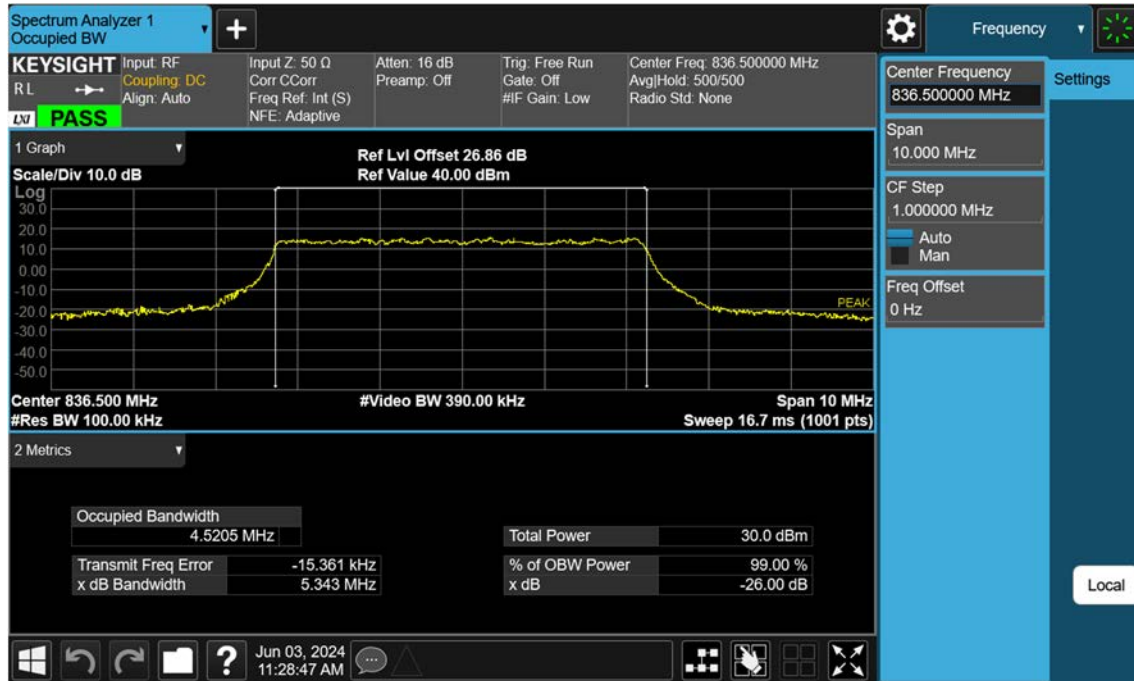
Sub6 n5_5 M_OBW_Mid_64QAM_FullRB
