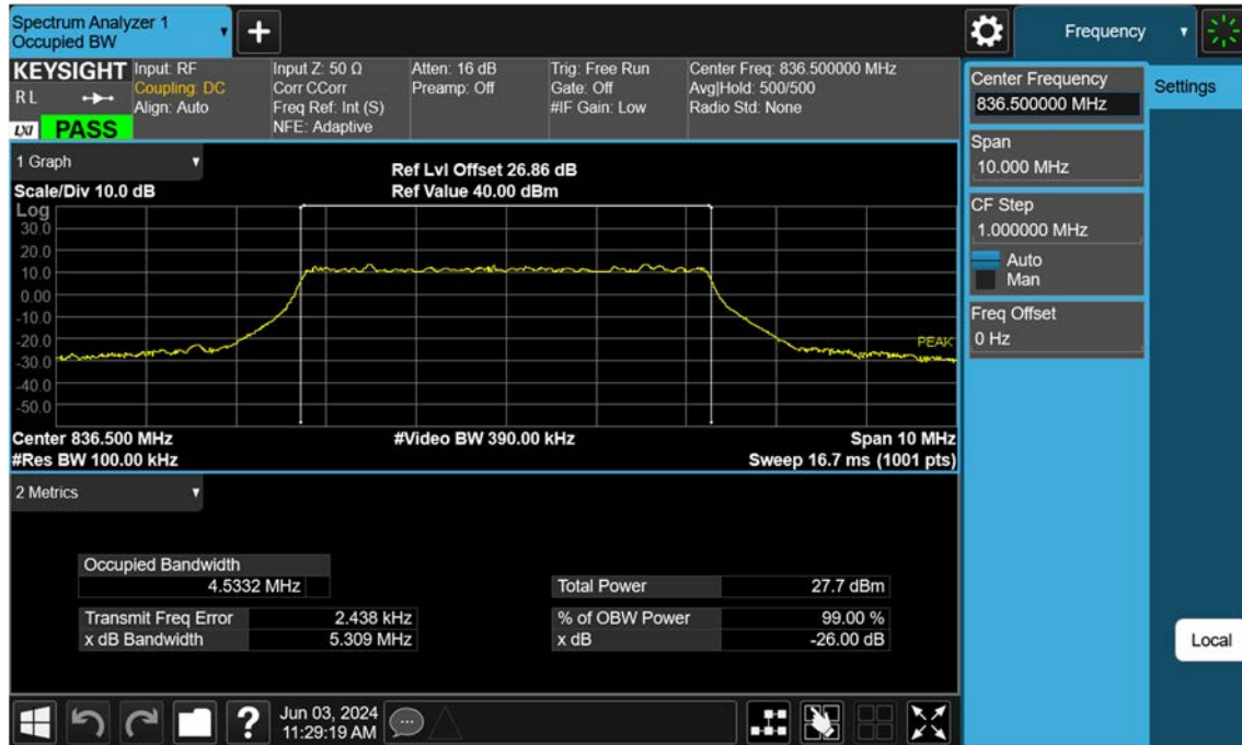
Sub6 n5_5 M_OBW_Mid_256QAM_FullRB
