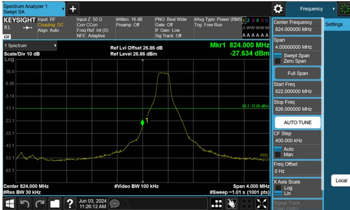
Sub6 n5_5 M_Band Edge_Low_BPSK_1RB
