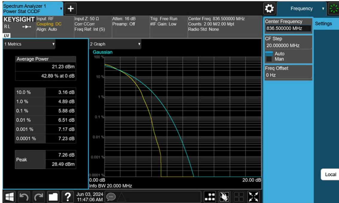
Sub6 n5_20 M_PAR_Mid_64QAM_FullRB
