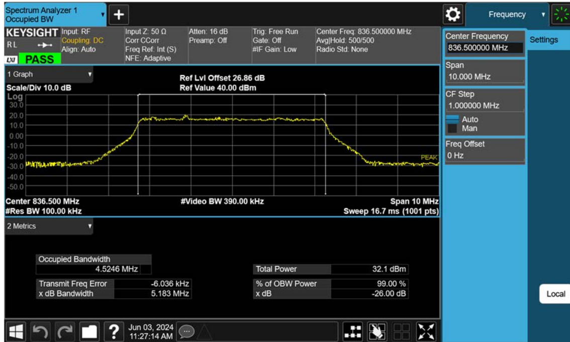
Sub6 n5_5 M_OBW_Mid_BPSK_FullRB
