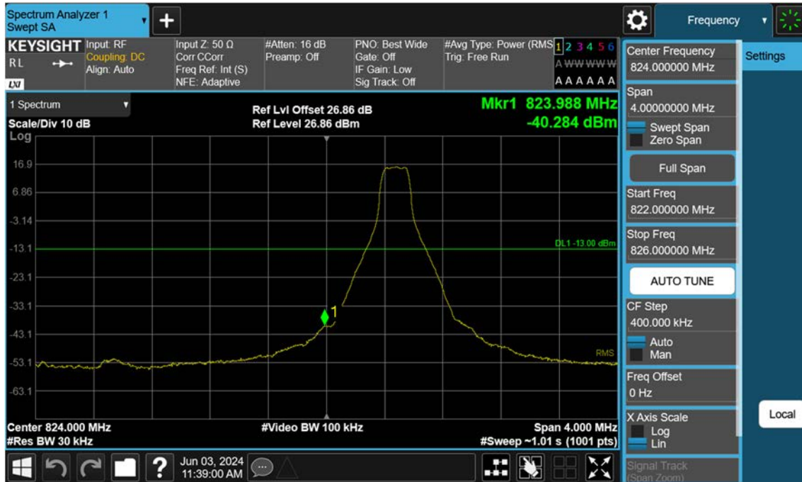
Sub6 n5_15 M_Band Edge_Low_BPSK_1RB
