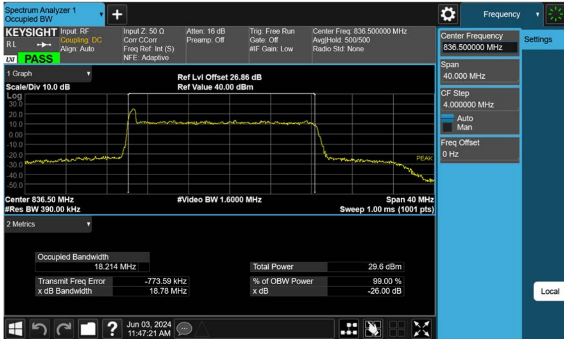
Sub6 n5_20 M_OBW_Mid_256QAM_FullRB
