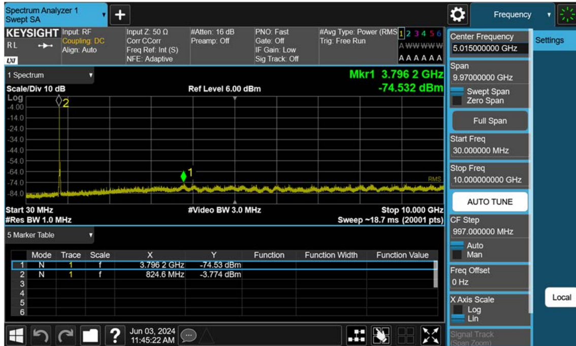
Sub6 n5_20 M_Conducted Spurious(30 M-10 G)_Low_BPSK_1RB
