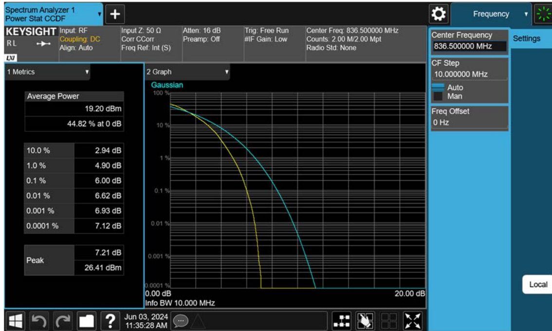
Sub6 n5_10 M_PAR_Mid_256QAM_FullRB
