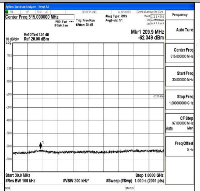
Band4_5MHz_16QAM_19975_1RB#0_30~1000_30~1000
