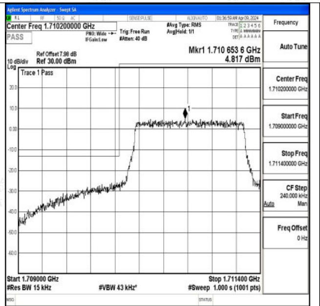
Band4_1.4MHz_16QAM_19957_6RB#0
