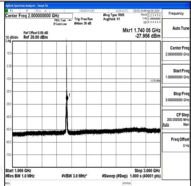
Band4_3MHz_QPSK_20175_1RB#0_1000~3000_1000~3000 00
