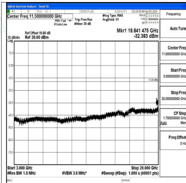
Band4_5MHz_QPSK_19975_1RB#0_3000~20000_3000~20000
