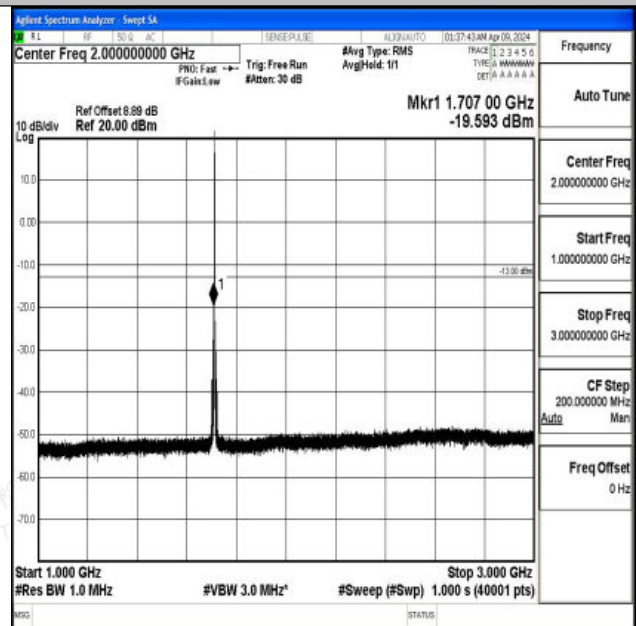
Band4_1.4MHz_QPSK_19957_1RB#0_1000~3000_1000~3000
