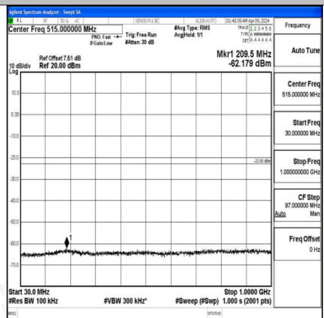
Band4_1.4MHz_16QAM_20393_1RB#0_30~1000_30~1000
