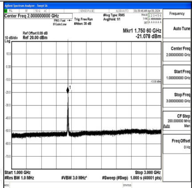
Band4_1.4MHz_QPSK_20393_1RB#0_1000~3000_1000~3000
