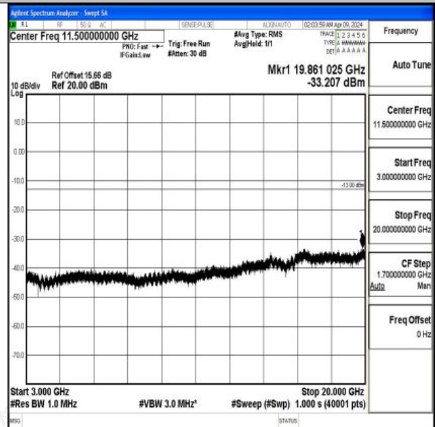
Band4_3MHz_16QAM_20385_1RB#0_3000~20000_3000~20000
