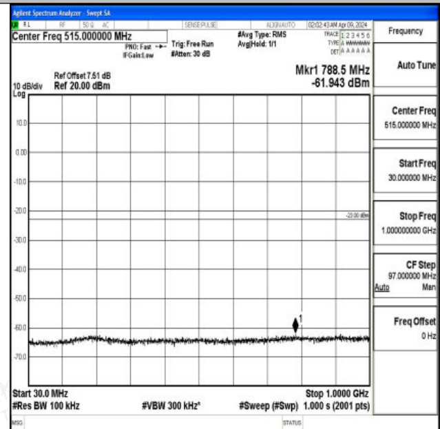
Band4_3MHz_16QAM_20175_1RB#0_30~1000_30~1000
