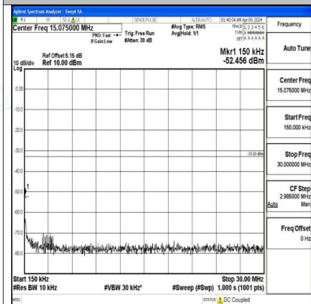
Band4_1.4MHz_16QAM_20393_1RB#0_0.15~30_0.15~30
