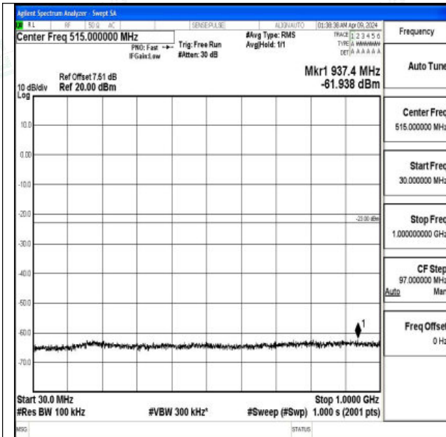
Band4_1.4MHz_QPSK_20175_1RB#0_30~1000_30~1000
