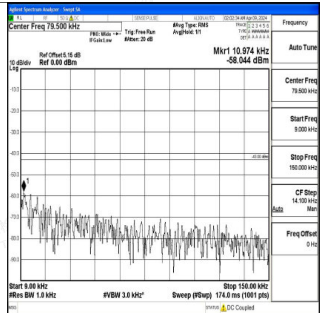
Band4_3MHz_16QAM_20175_1RB#0_0.009~0.15_0.009~0.15
