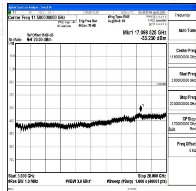
Band4_1.4MHz_QPSK_20393_1RB#0_3000~20000_3000~20000
