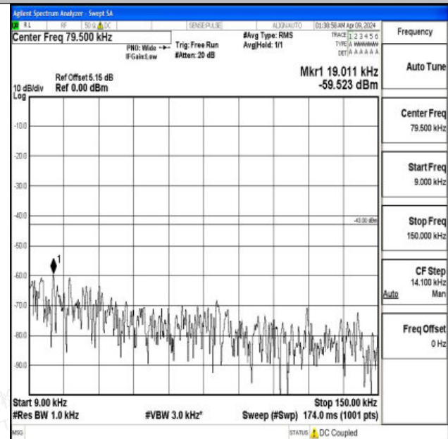
Band4_1.4MHz_16QAM_20175_1RB#0_0.009~0.15_0.009~0.15
