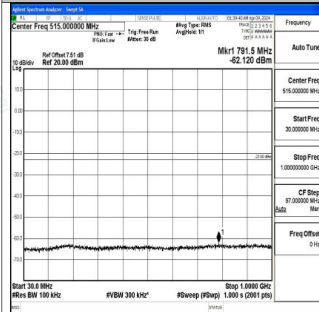
Band4_1.4MHz_QPSK_20393_1RB#0_30~1000_30~1000
