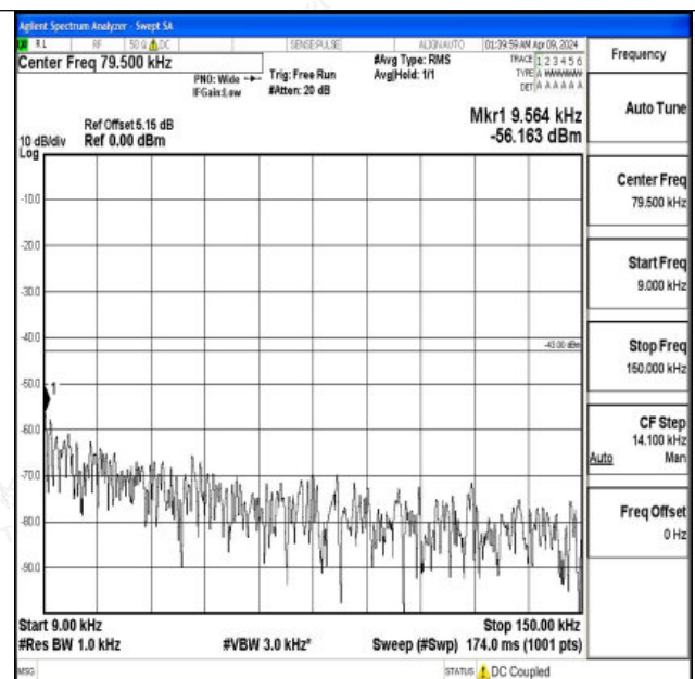
Band4_1.4MHz_16QAM_20393_1RB#0_0.009~0.15_0.009~0.15
