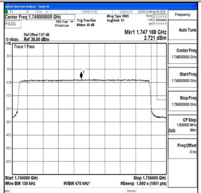
Band4_15MHz_16QAM_20325_75RB#0
