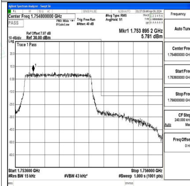
Band4_1.4MHz_QPSK_20393_6RB#0
