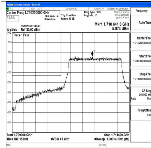
Band4_1.4MHz_QPSK_19957_6RB#0
