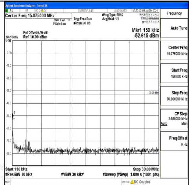
Band4_5MHz_QPSK_20175_1RB#0_0.15~30_0.15~30
