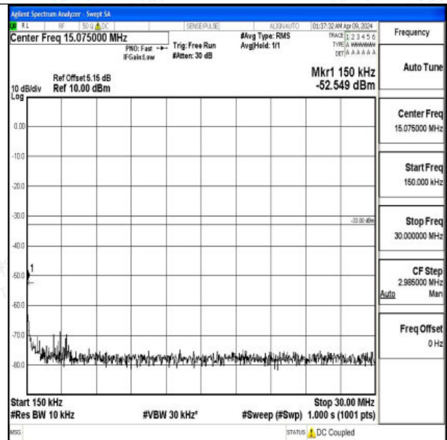
Band4_1.4MHz_QPSK_19957_1RB#0_0.15~30_0.15~30
