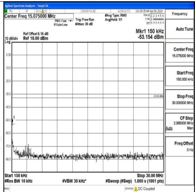
Band4_1.4MHz_QPSK_20393_1RB#0_0.15~30_0.15~30
