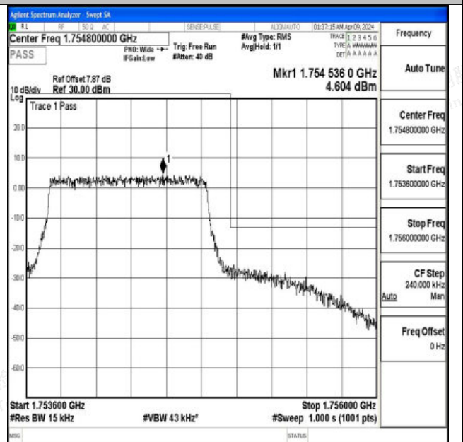
Band4_1.4MHz_16QAM_20393_6RB#0
