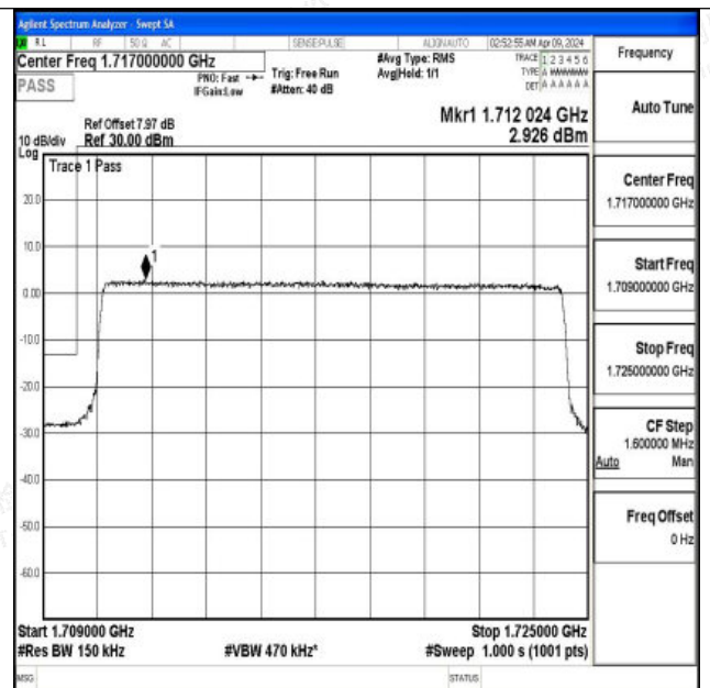
Band4_15MHz_16QAM_20025_75RB#0
