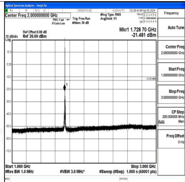
Band4_1.4MHz_QPSK_20175_1RB#0_1000~3000_1000~3000
