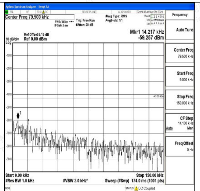
Band4_5MHz_16QAM_19975_1RB#0_0.009~0.15_0.009~0.15
