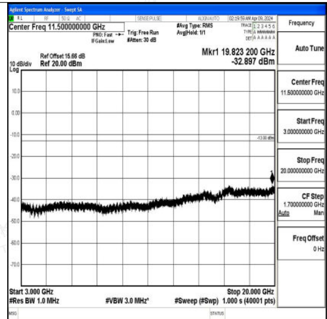
Band4_5MHz_16QAM_19975_1RB#0_3000~20000_3000~20000
