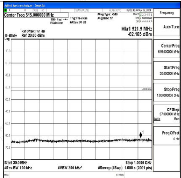
Band4_3MHz_16QAM_20385_1RB#0_30~1000_30~1000
