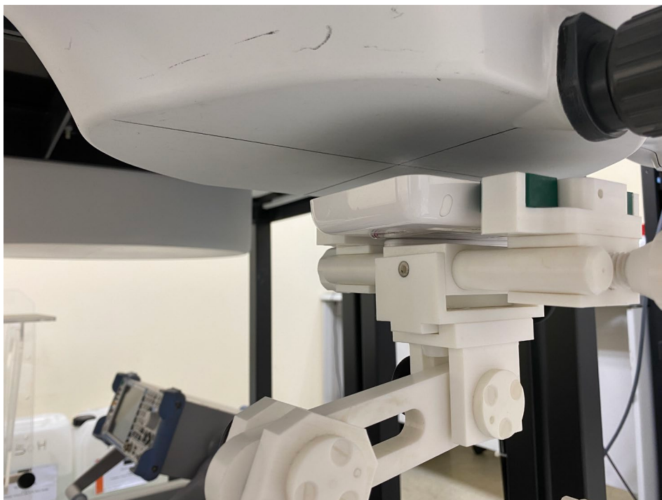
Figure 1 – Front with 25mm Separation
