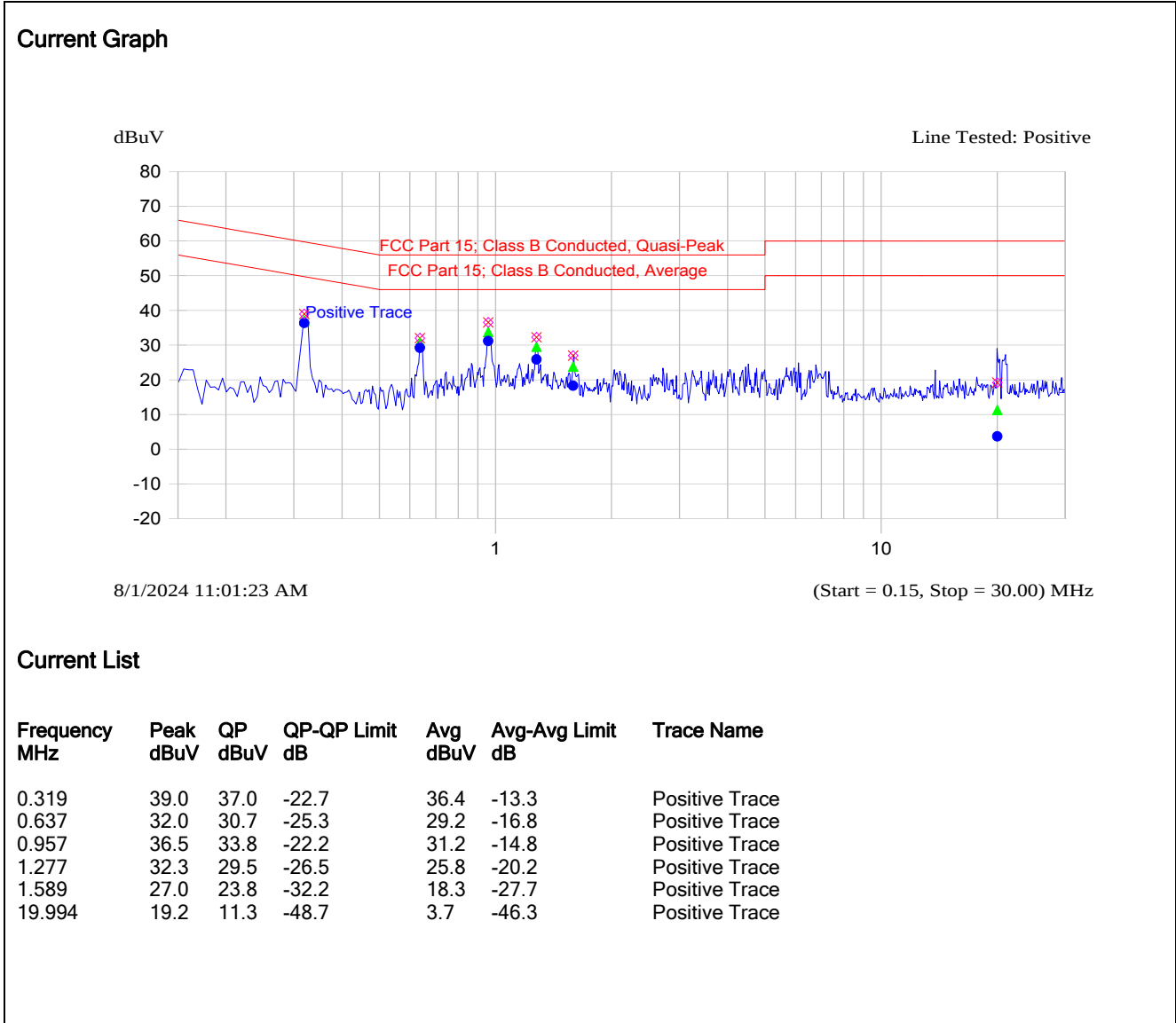
Plot 5.1.4.3. Power Line Conducted Emissions (BLE 1M, Rx Mode) Line Voltage: 3.6 VDC; Line Tested: Positive Trace
