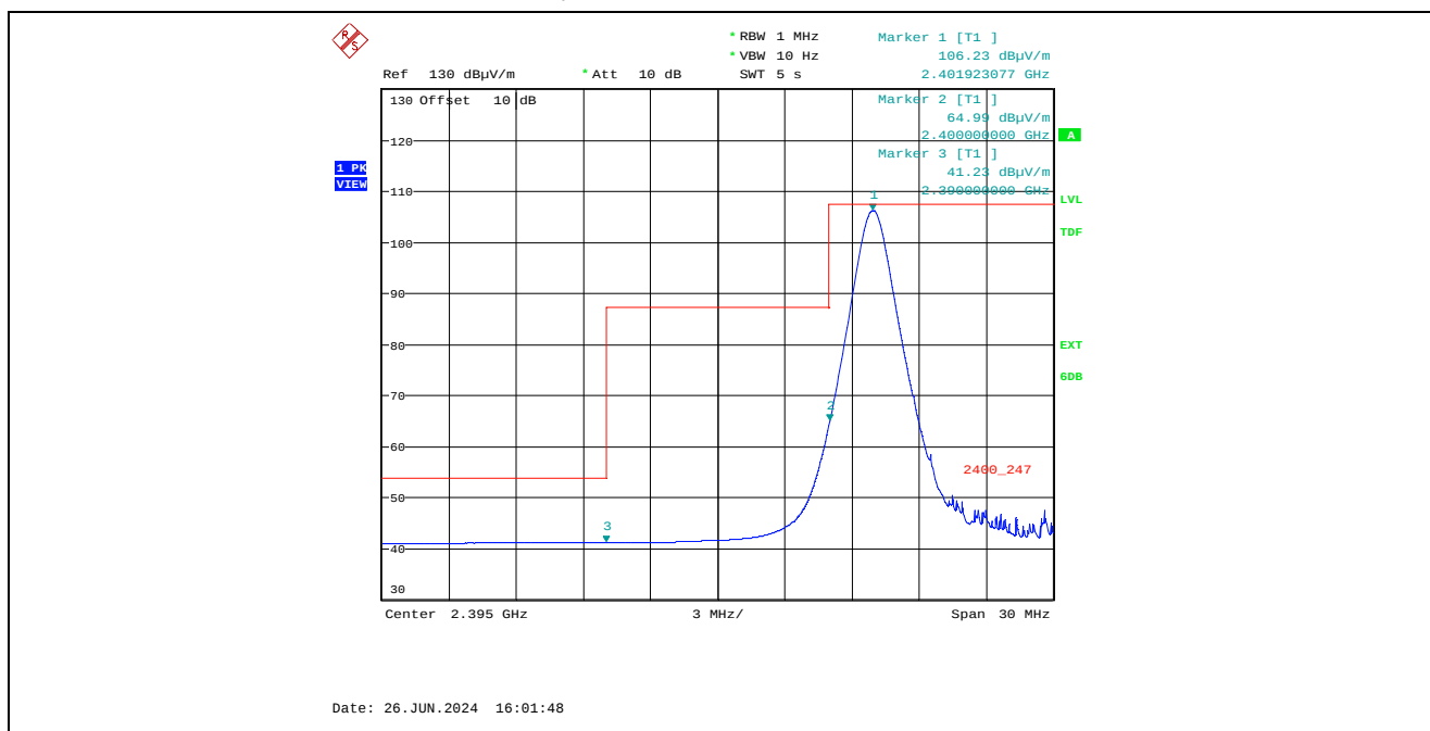
Plot 5.4.4.1.2.2. Radiated Band-Edge Emission at 3 m, Vertical Polarization, Average Low End of Frequency Band, 2402 MHz, GFSK Modulation, 1M, 1 Mb/s
