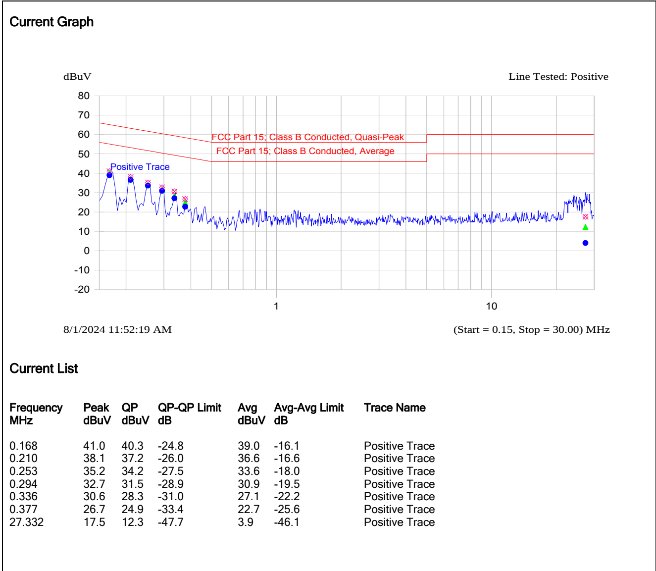
Plot 5.1.4.5. Power Line Conducted Emissions (BLE Coded PHY, Tx Mode) Line Voltage: 3.6 VDC; Line Tested: Positive Trace
