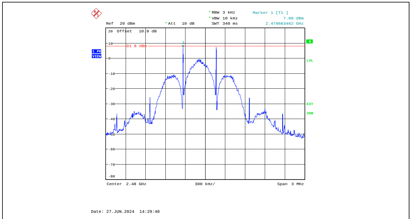
Plot 5.5.4.6. Power Spectral Density, GFSK Modulation, Coded PHY, 125 kb/s, 2480 MHz
