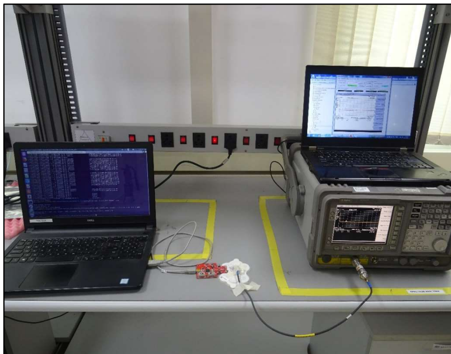
Antenna Port Test Setup Photo
