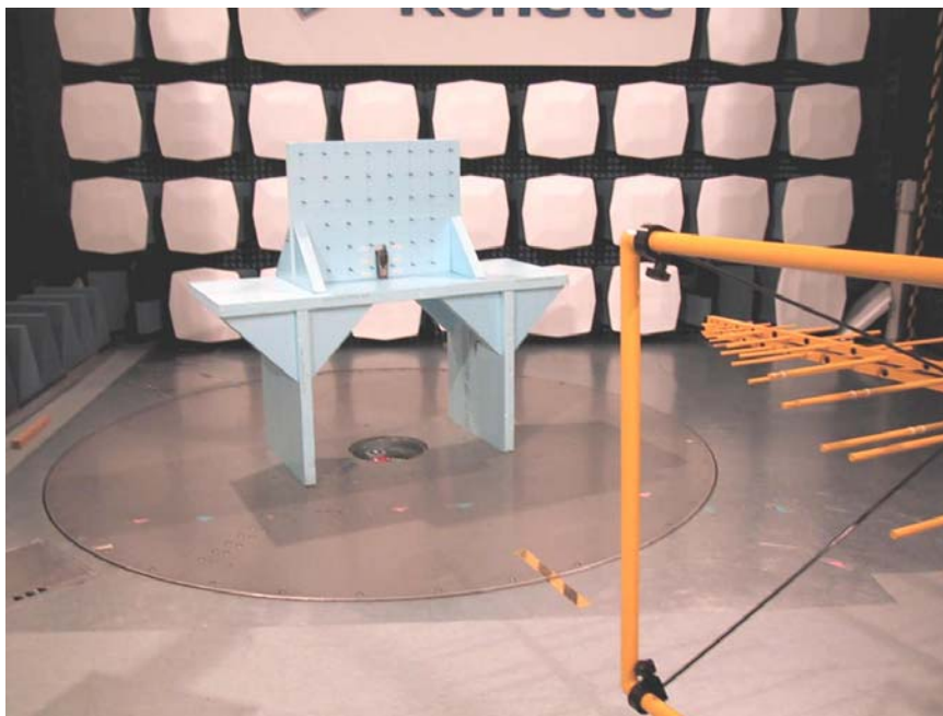
Picture 2: Radiated spurious emission measurement set-up for below 3 GHz measurements, EUT in vertical orientation
