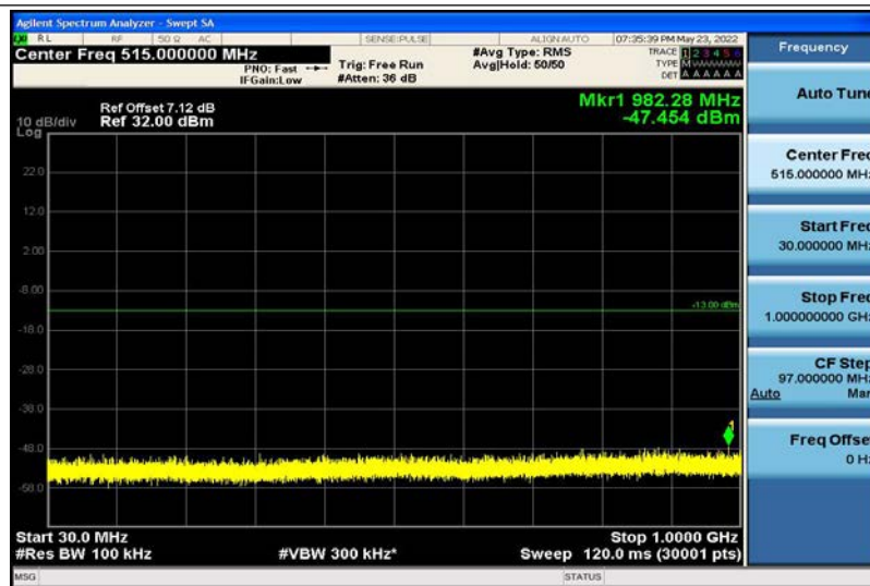
Band4-5MHz-QPSK-20175-1RB#0-30~1000MHz
