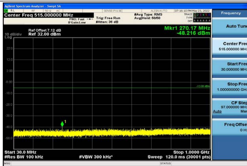
Band4-3MHz-16QAM-19965-1RB#0-30~1000MHz
