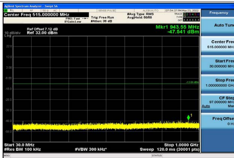
Band4-10MHz-QPSK-20175-1RB#0-30~1000MHz
