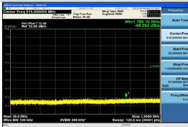
Band2-10MHz-16QAM-18900-1RB#0-30~1000MHz
