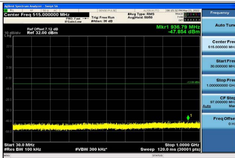
Band4-15MHz-QPSK-20175-1RB#0-30~1000MHz
