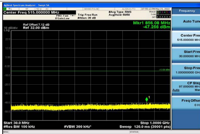
Band4-10MHz-16QAM-20175-1RB#0-30~1000MHz
