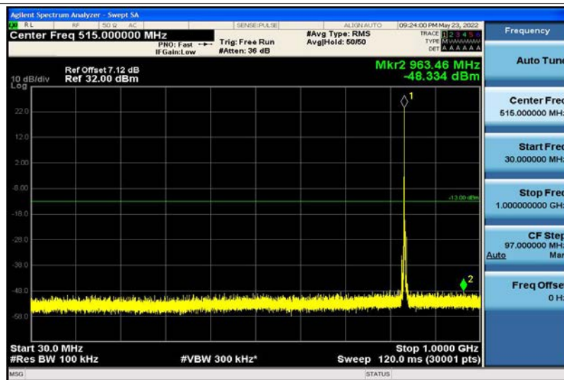
Band5-3MHz-QPSK-20525-1RB#0-30~1000MHz
