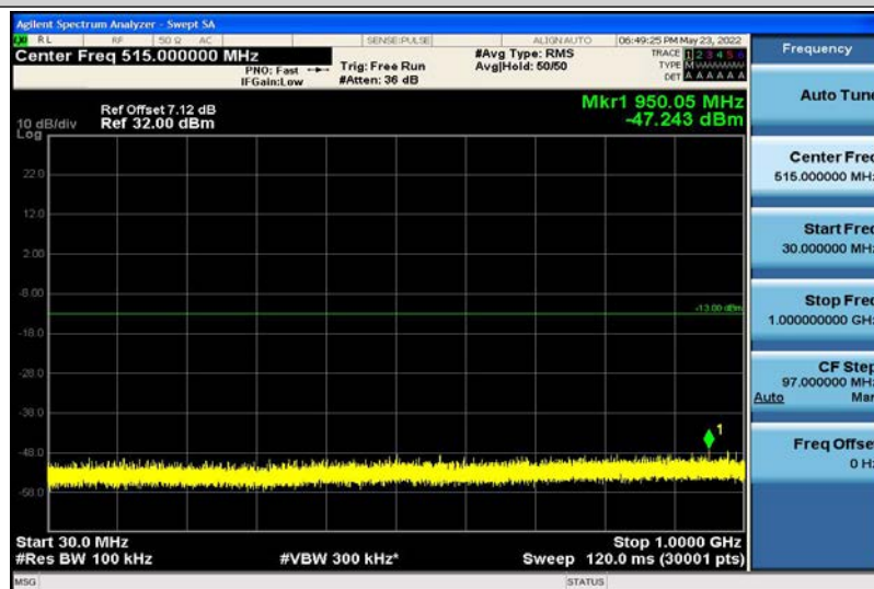
Band4-1.4MHz-16QAM-19957-1RB#0-30~1000MHz
