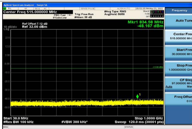
Band2-15MHz-QPSK-18900-1RB#0-30~1000MHz
