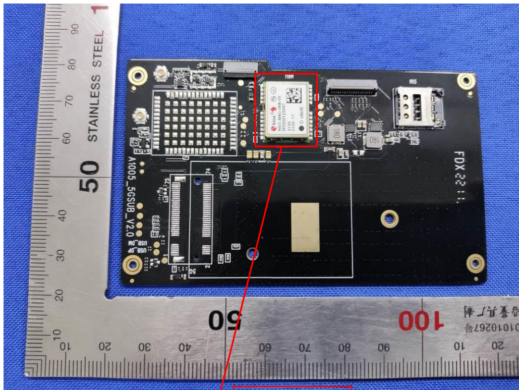
GPS RFchip
