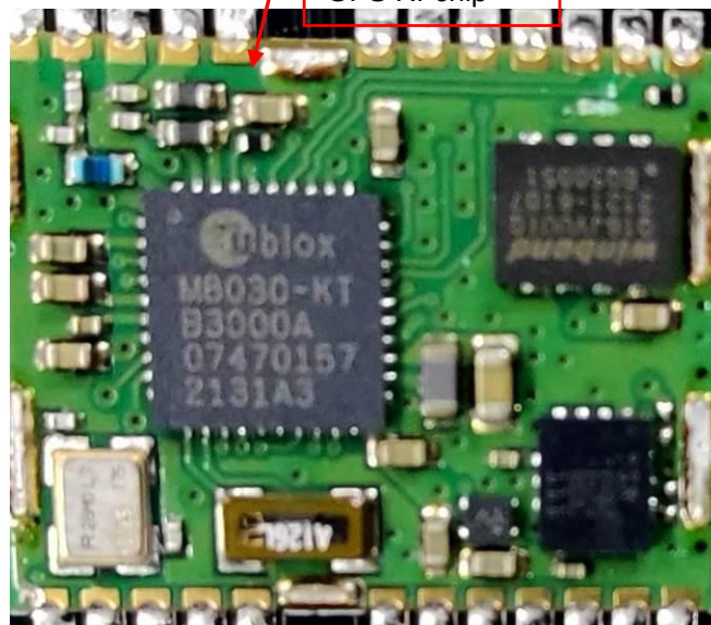
GPS RFchip
