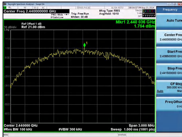
BLE_2M-Ant1-2440-0~Reference-PASS
